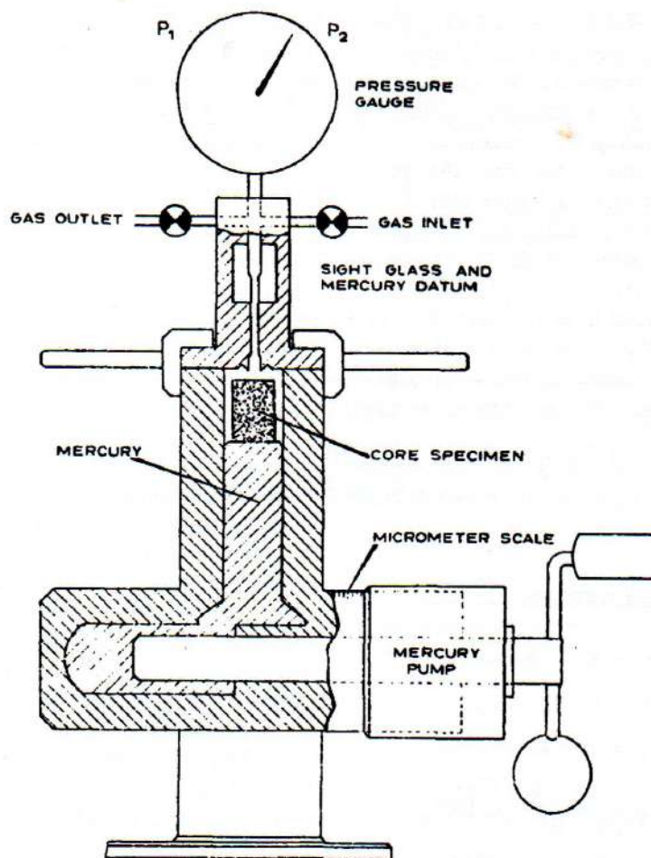
Fig. 1. Schematic diagram of a Kobe Boyle's law porosimeter.
