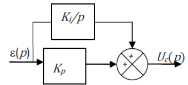
FIGURE 4 – Correction PI
