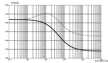
FIGURE 1.1 – Courbe de phase
