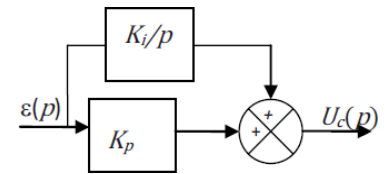
FIGURE 11.3 – Correction PI
