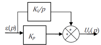
FIGURE 12.2 – Correction PI
