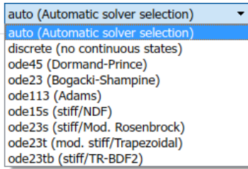
FIGURE 3.1 – Solveurs Matlab
