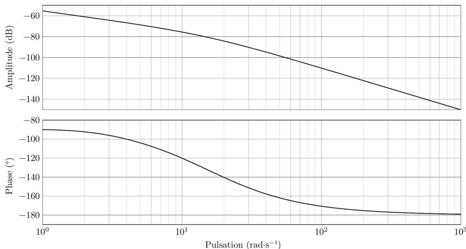
FIGURE 1.19 – Diagramme de Bode de H_{BOf}(p)
