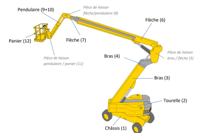
FIGURE 5.5 – Architecture globale de la nacelle
