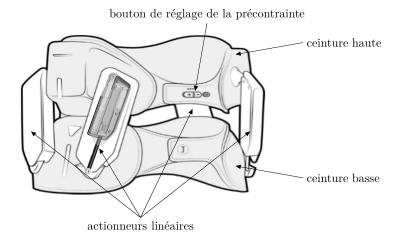
FIGURE 2.12 : Exosquelette lombaire Japet
