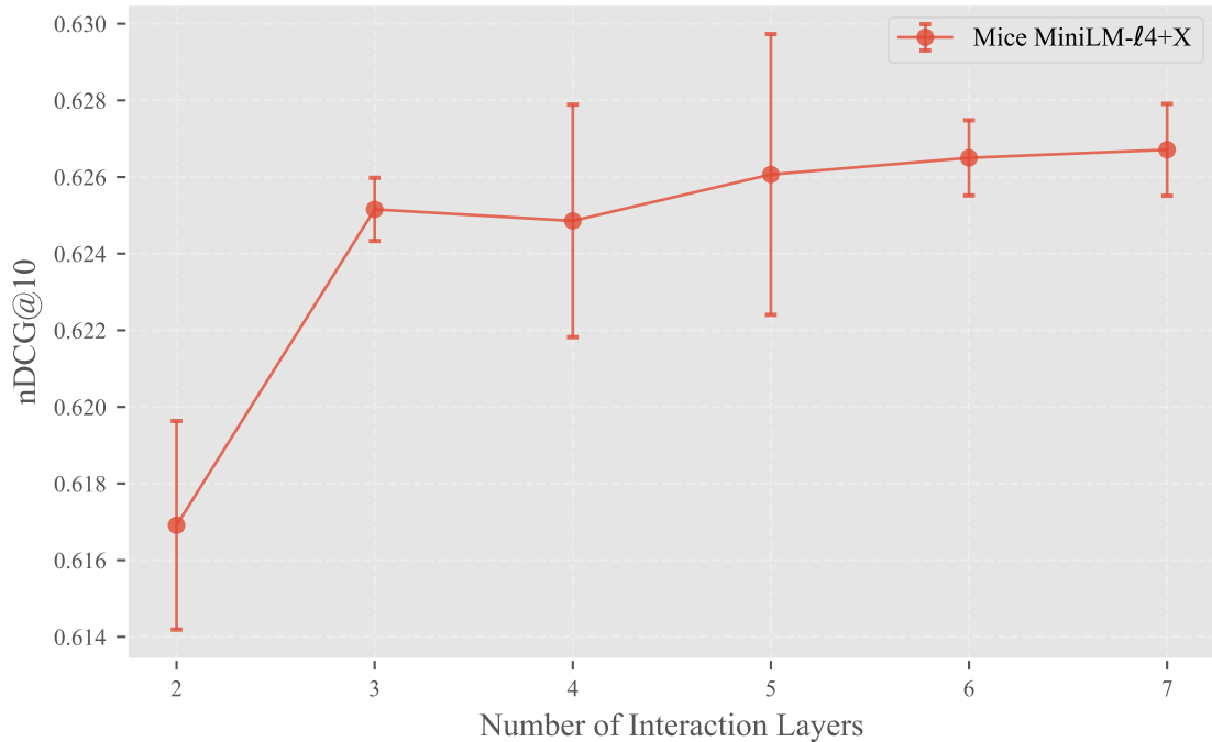
nDCG@10 vs Interaction Layers (In Domain)
