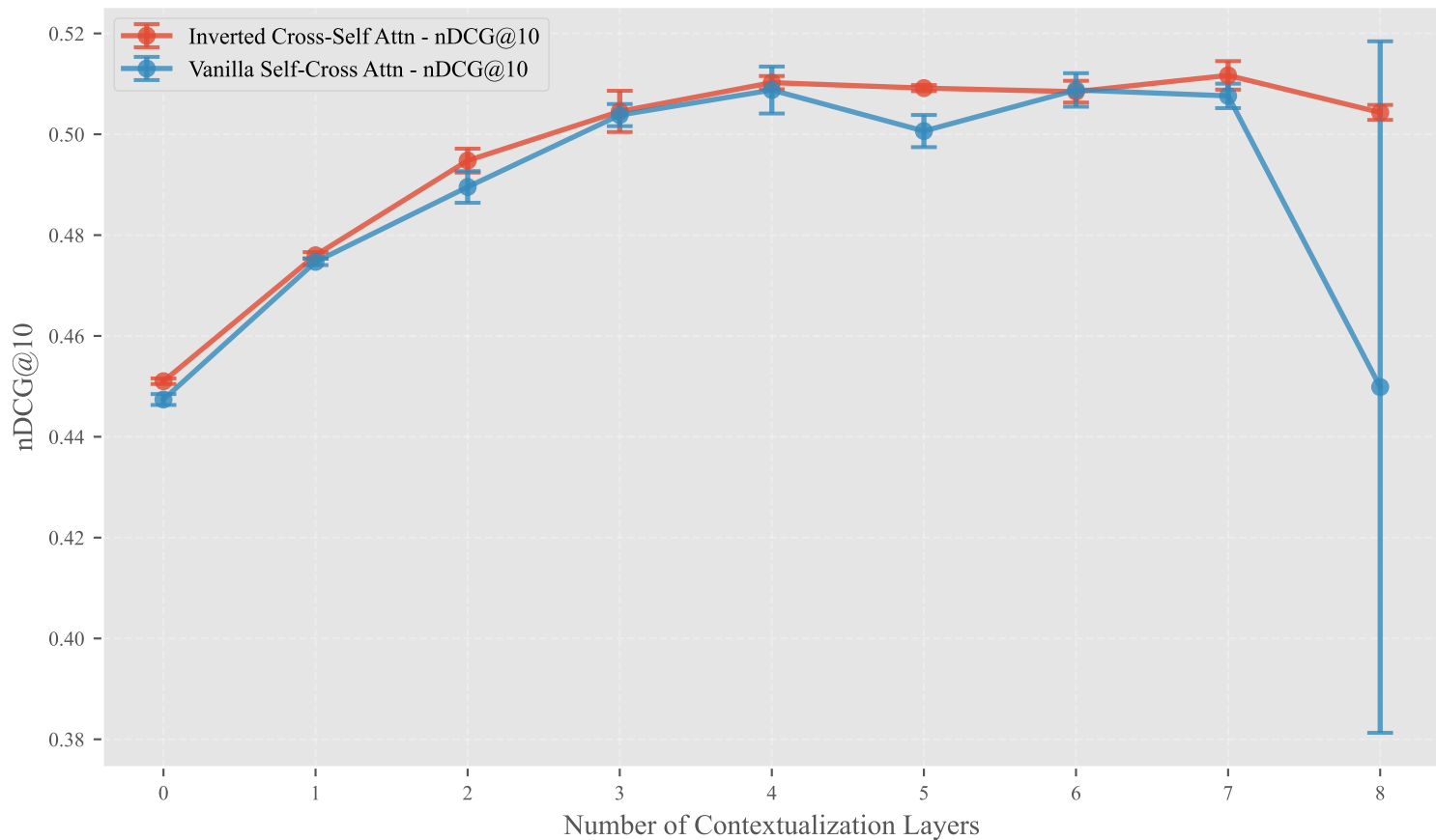
nDCG@10 vs Contextualization Layers (mean)
