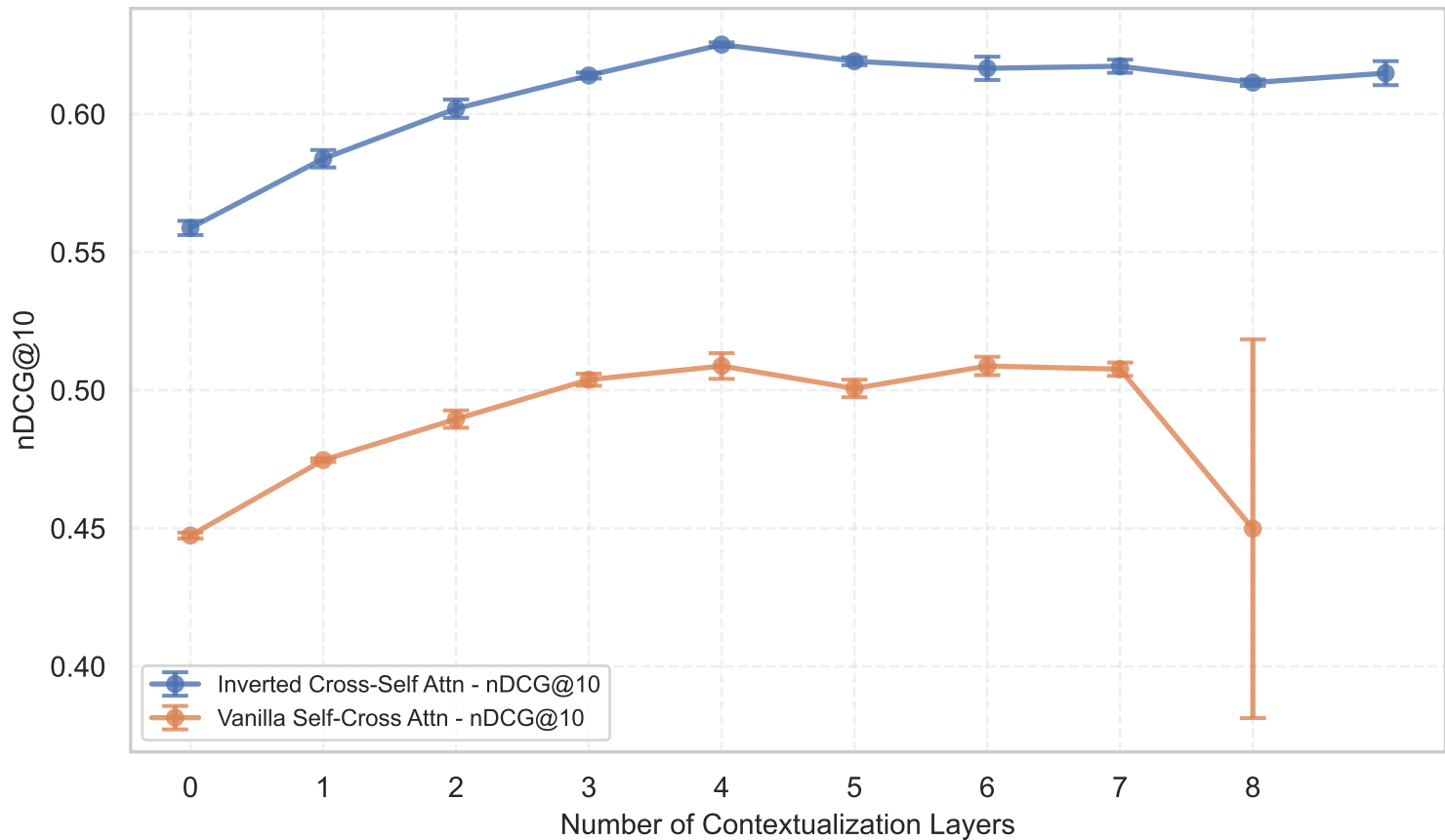
nDCG@10 vs Contextualization Layers (mean)
