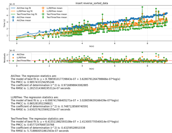
Figure 3: Comparison of insertion time under reverse-sorted keys.
