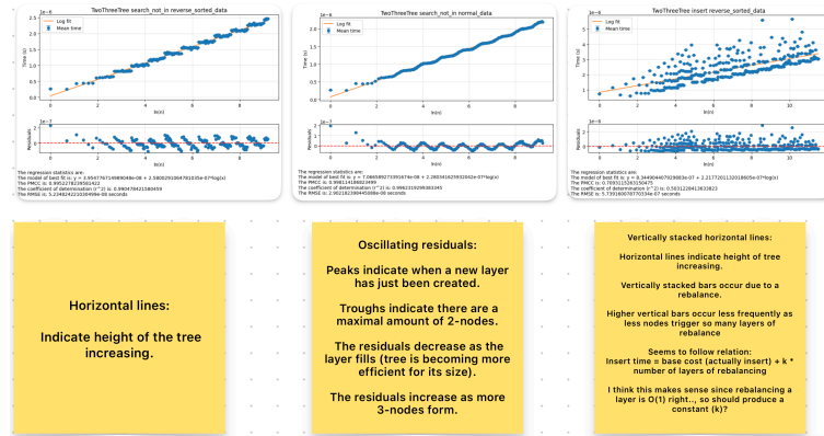
Figure 2: Representative 2-3 tree plots illustrating residual patterns.
