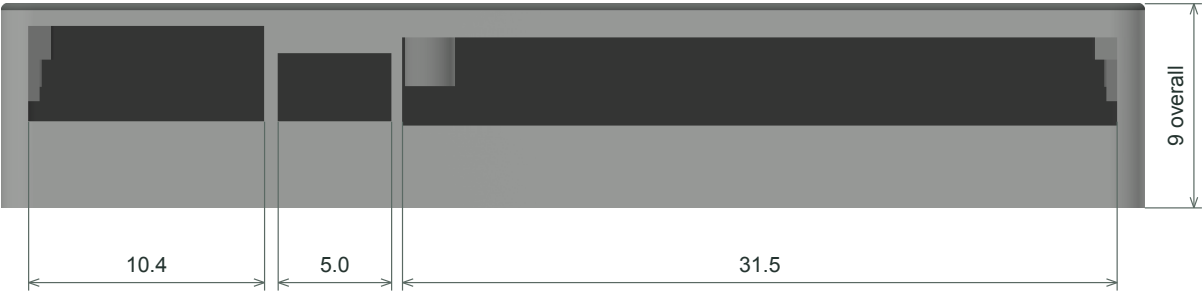
FRONT / CONNECTOR EDGE
