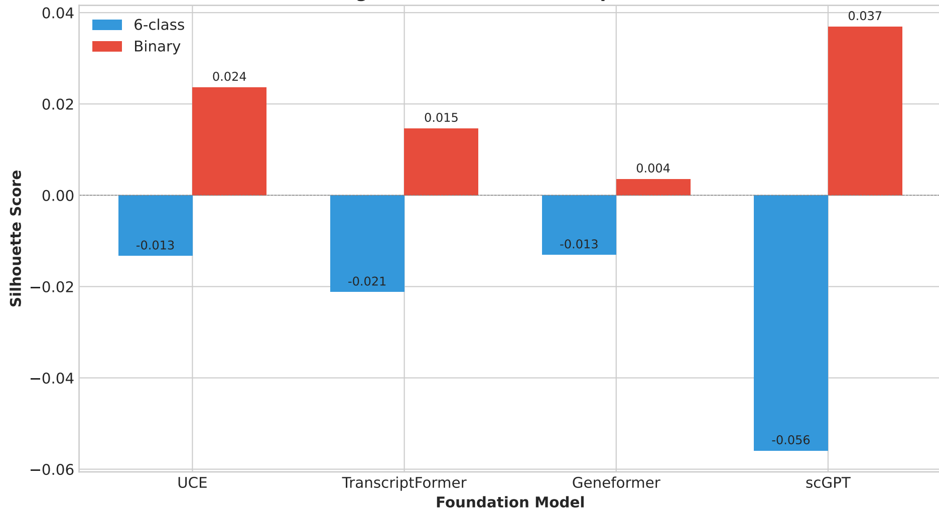
Embedding Quality: Silhouette Score by Model (Higher = Better Cluster Separation)
