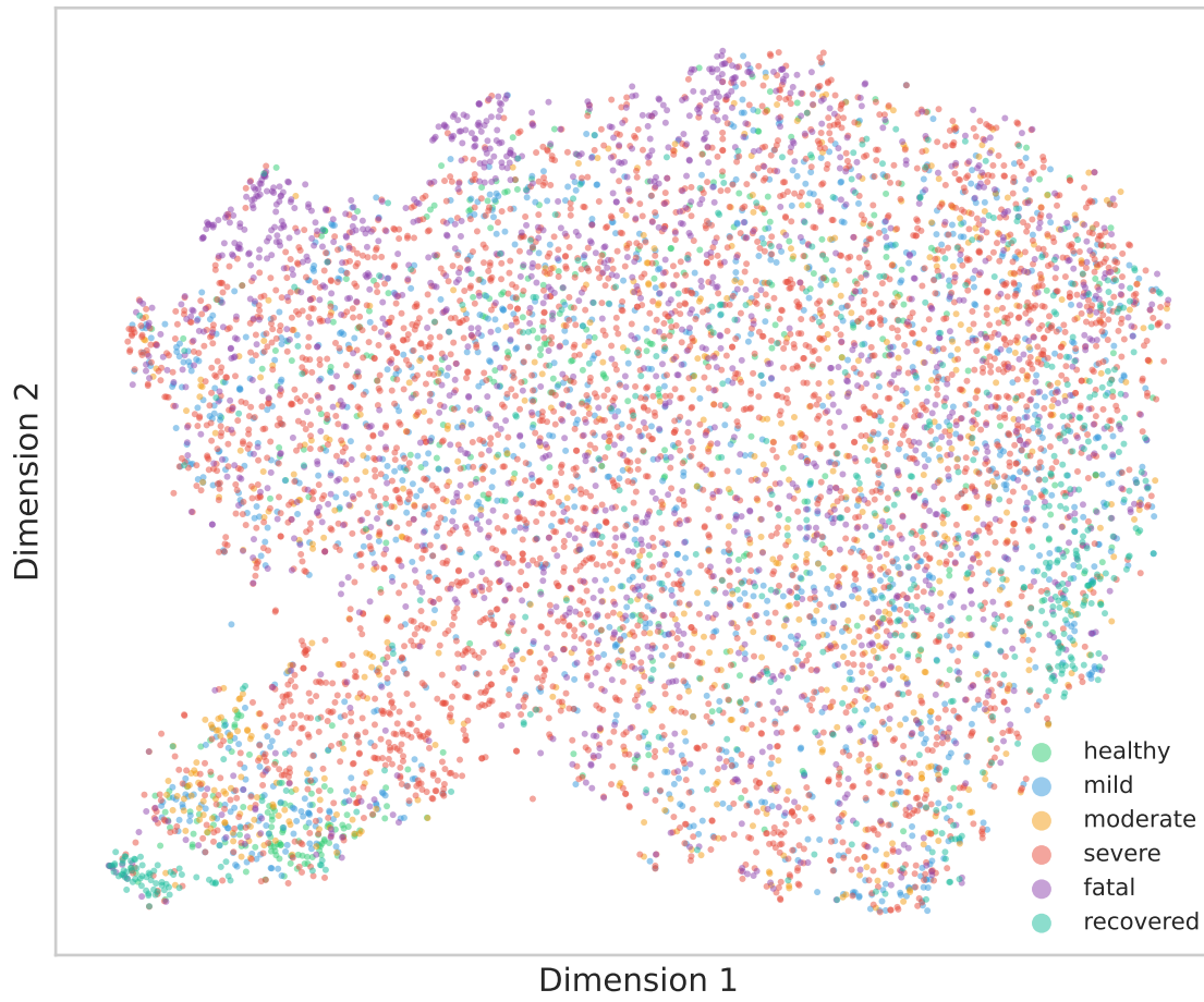
TranscriptFormer - tSNE
