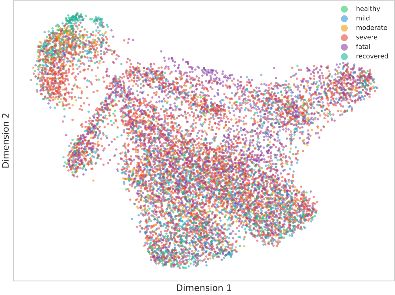
Geneformer (1152 dims)
