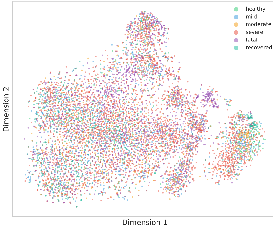
Geneformer - tSNE
