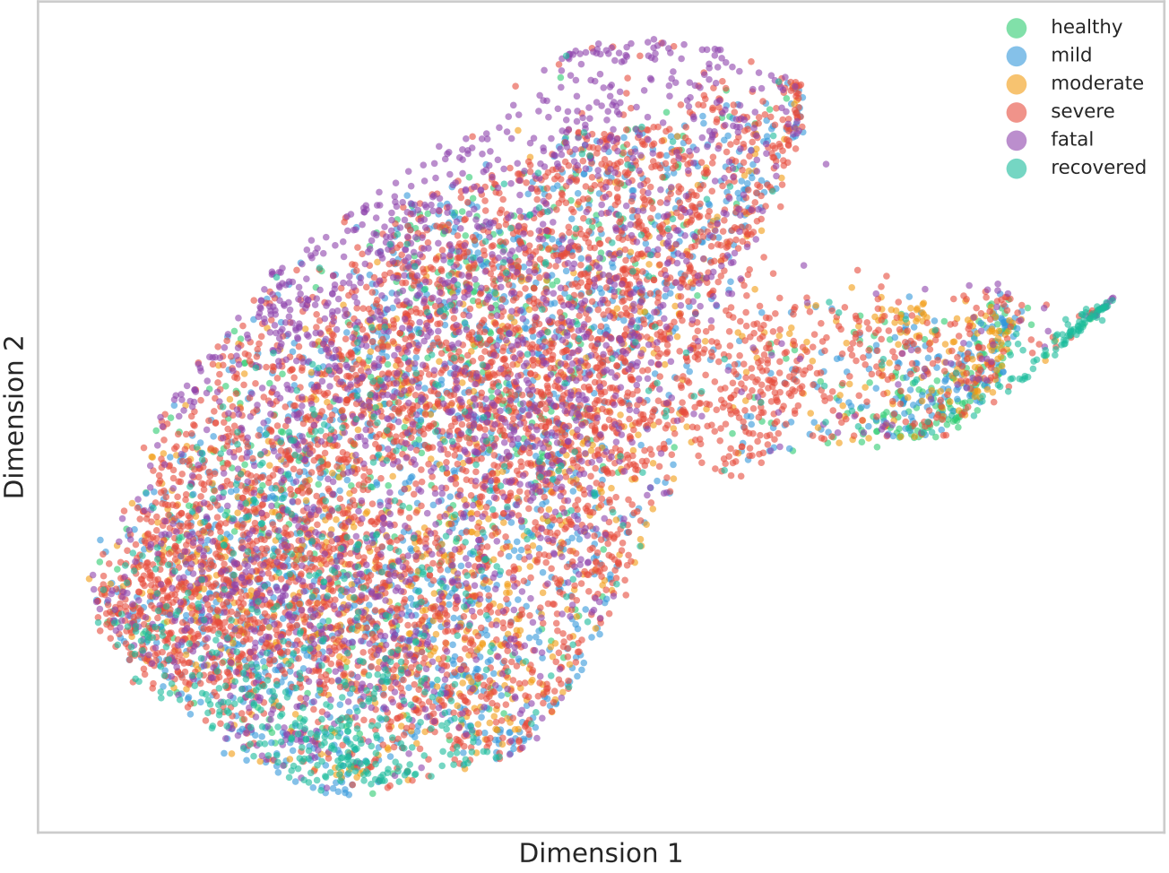
scGPT (512 dims)
