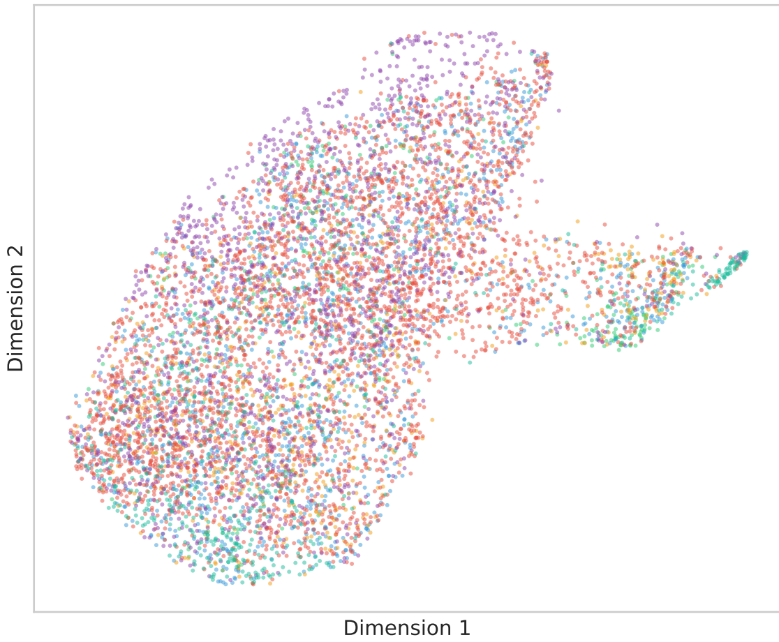
TranscriptFormer - UMAP
