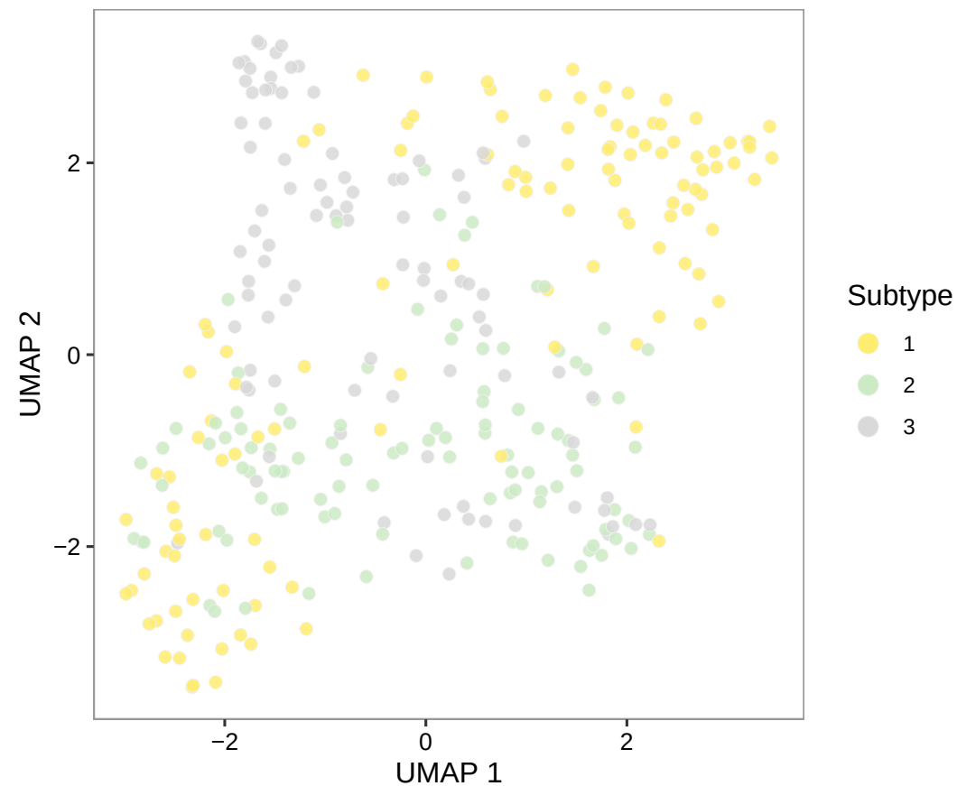
TCGA-Defined Subtypes
