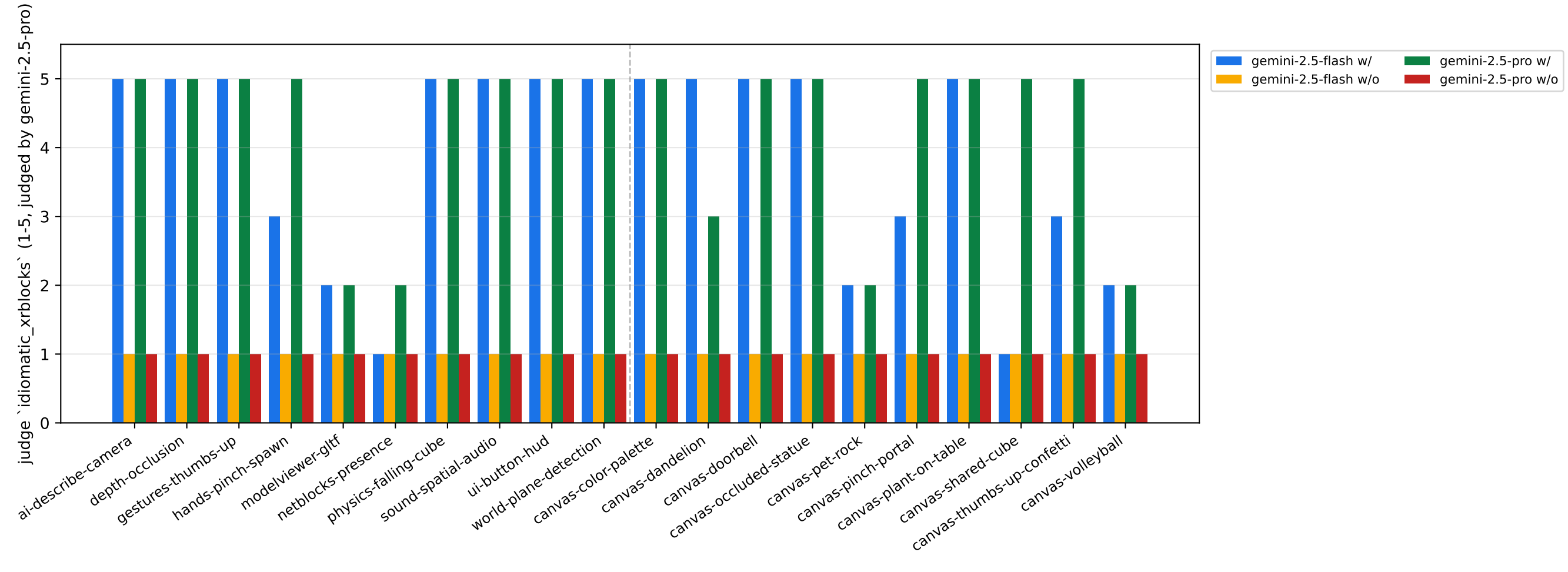
llm judge: idiomatic xrblocks usage, with vs without skill, across models engineer-spec canvas-faithful
