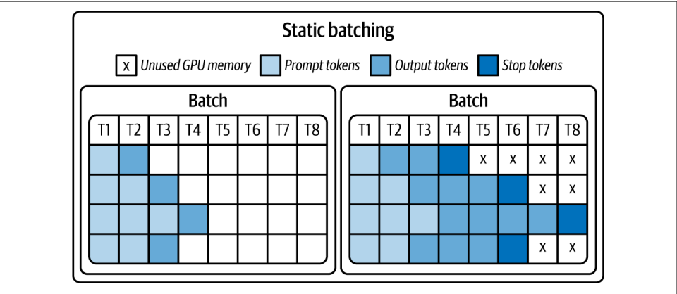
Figure 5-15. Static batching with fixed batch size
