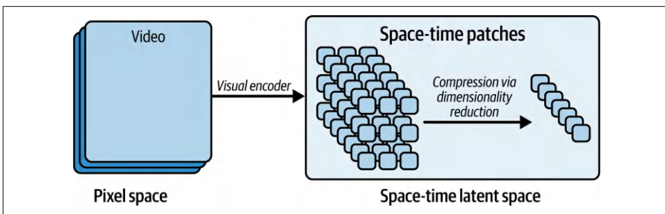
Figure 3-21. Video compression into space-time patches
