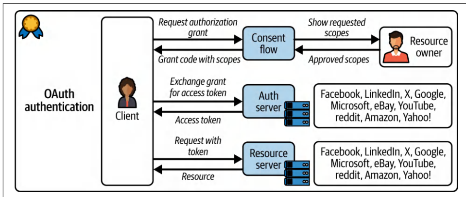
Figure 8-8. OAuth authentication flow
