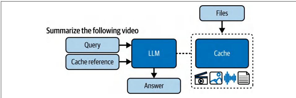
Figure 10-3. System architecture for context caching
