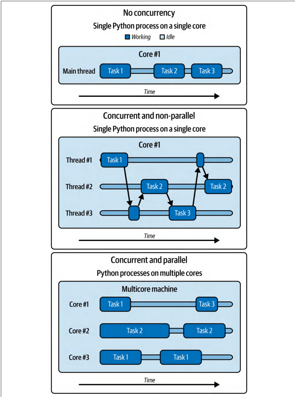
Figure 5-2. Concurrency with and without parallelism
