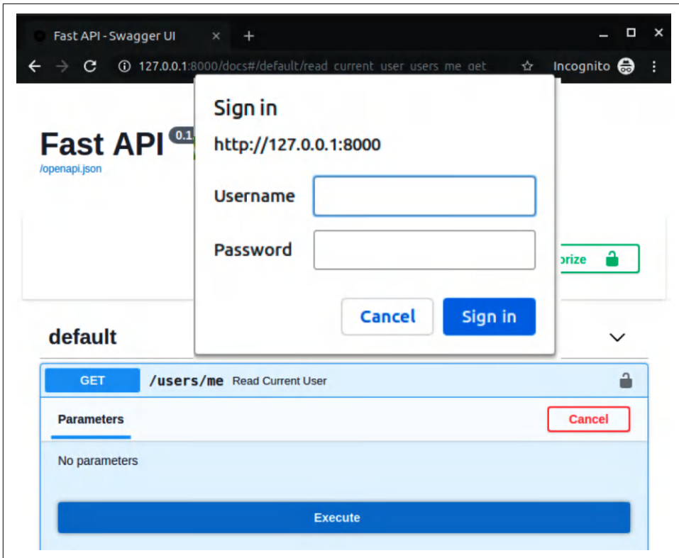
Figure 8-2. Basic authentication in FastAPI
