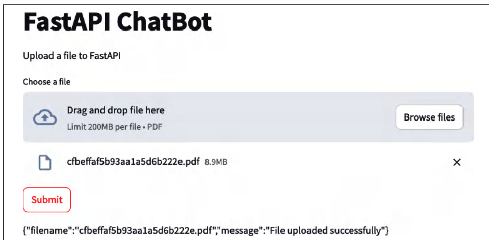
Figure 5-10. Uploading files via Streamlit to the FastAPI service
