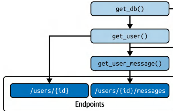
Figure 2-2. Dependency injection in FastAPI
