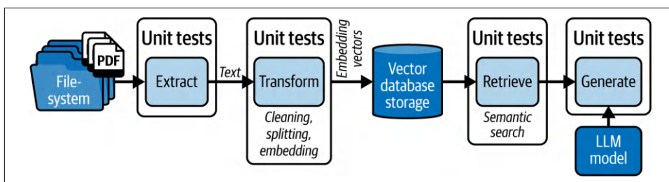
Figure 11-8. Unit test boundaries visualized on the RAG data pipeline diagram
