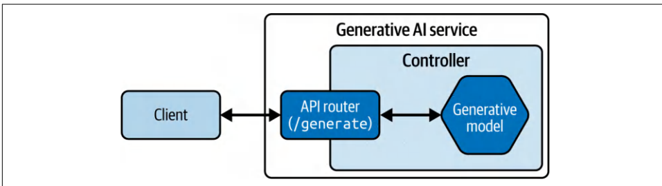
Figure 3-13. FastAPI service system architecture
