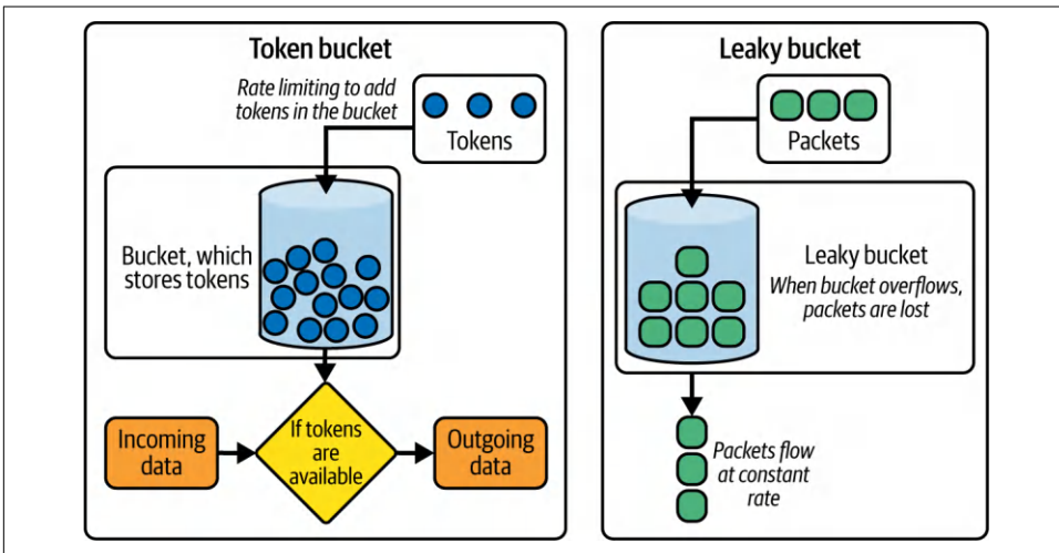
Figure 9-2. Comparison of rate-limiting strategies
