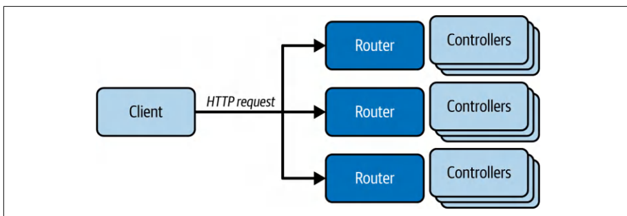
Figure 2-4. API routers and controllers
