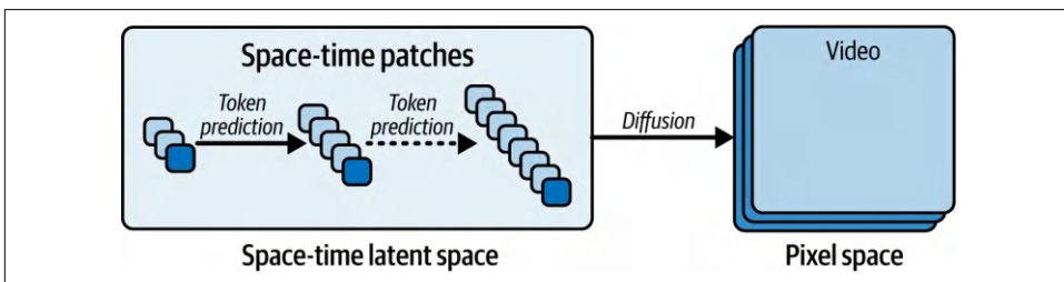
Figure 3-22. Token prediction by the vision transformer
