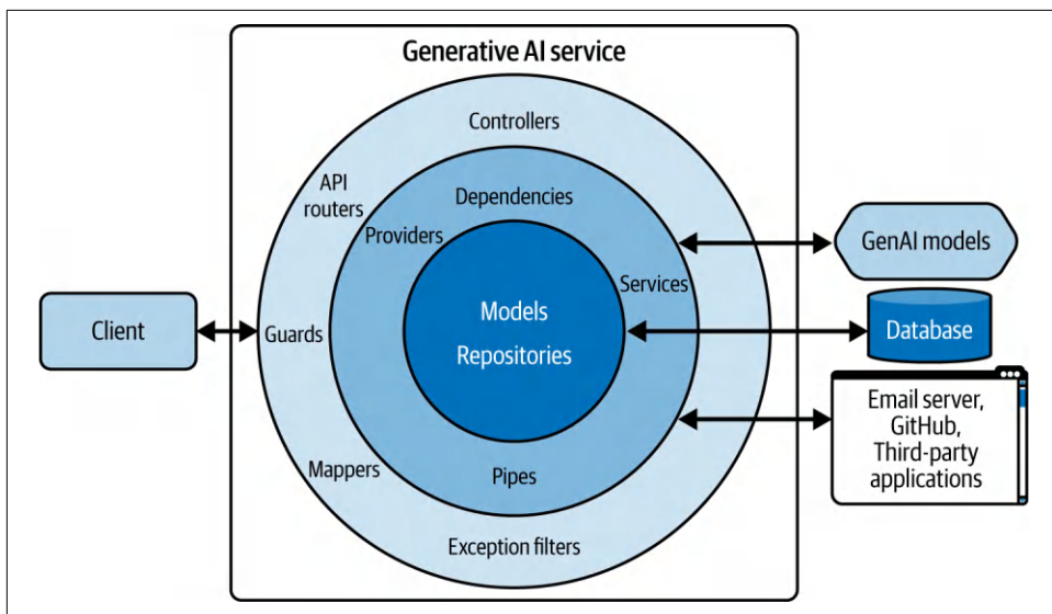
Figure 2-3. Onion design pattern
