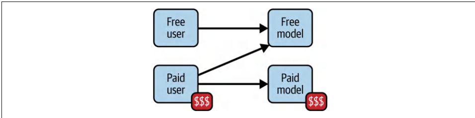
Figure 8-15. ABAC example where only paid users have access to premium GenAI models
