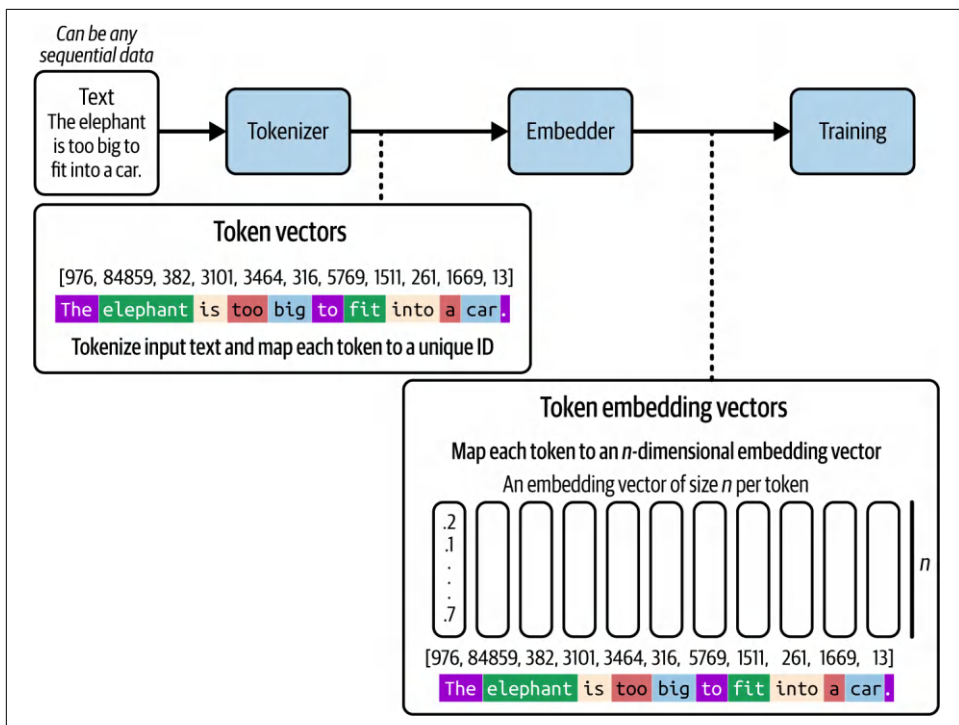
Figure 3-8. Processing sequential data like a piece of text into a vector of tokens and token embeddings
