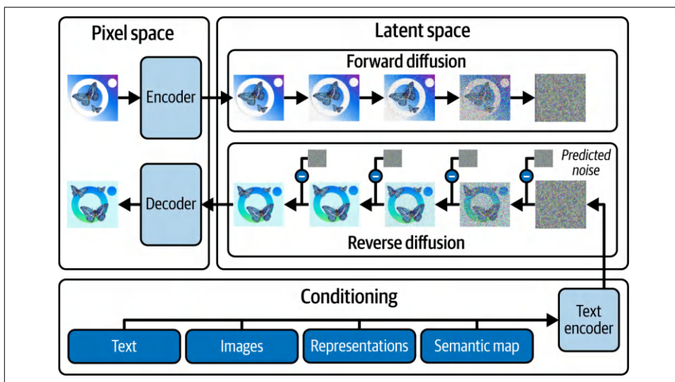
Figure 3-17. Stable Diffusion training and inference
