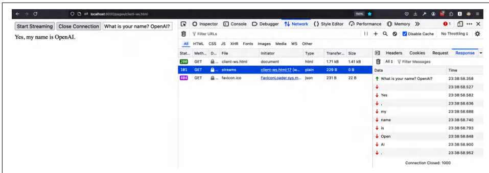
Figure 6-9. Incoming stream from the WebSocket endpoint
