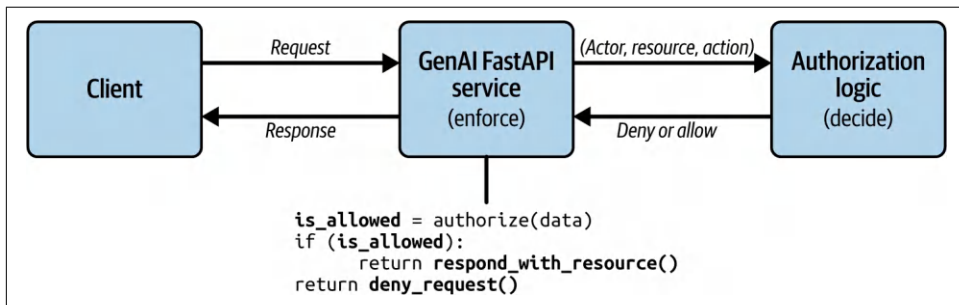
Figure 8-17. Separating the authorization service from the GenAI service
