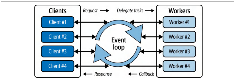
Figure 5-4. Async IO event loop
