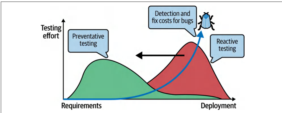
Figure 11-3. Shift-left software testing
