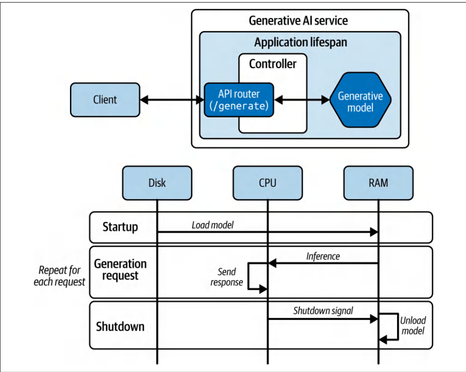
Figure 3-29. Using the FastAPI application lifespan to preload models
