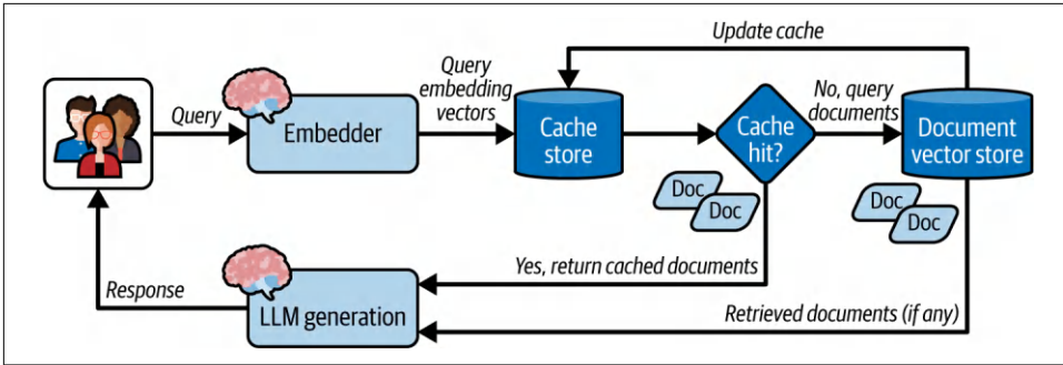
Figure 10-1. Semantic caching in RAG system architecture
