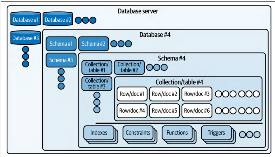
Figure 7-1. Database system breakdown
