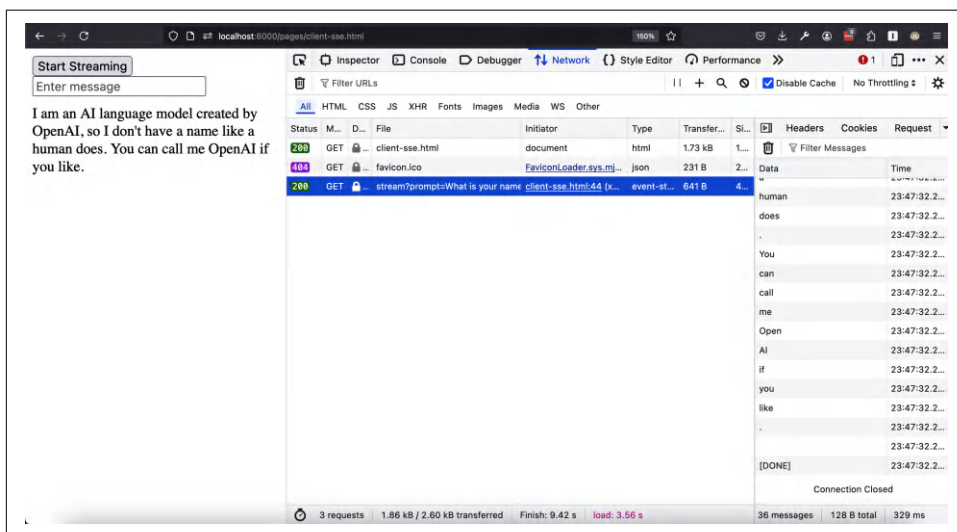
Figure 6-8. Incoming stream from the SSE endpoint
