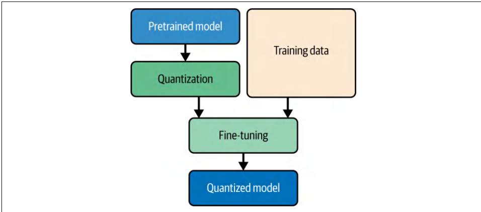
Figure 10-4. Quantization process
