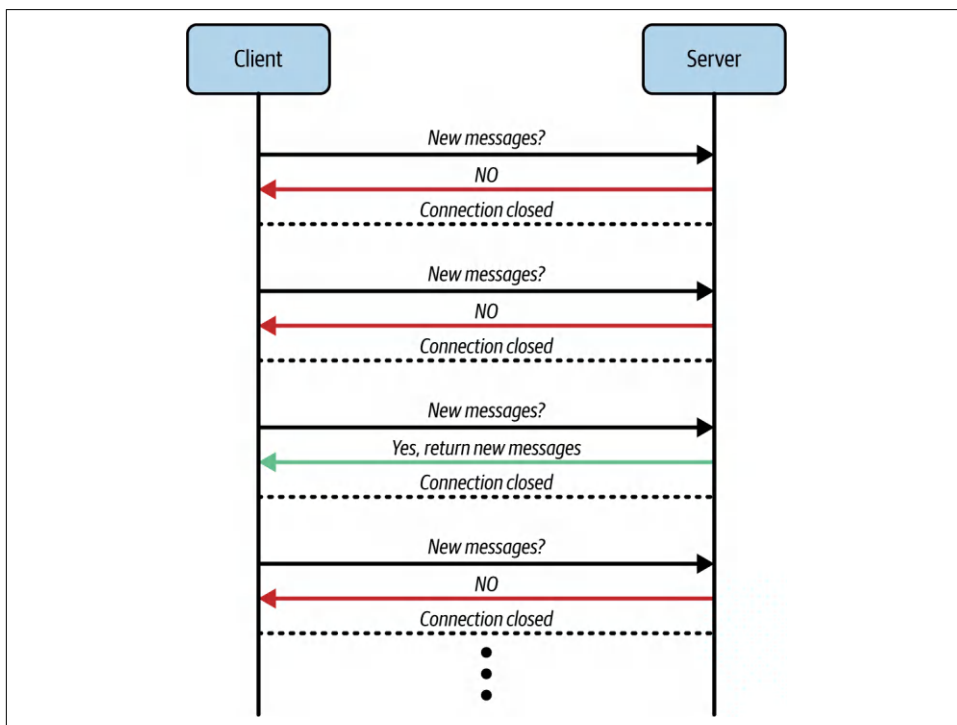
Figure 6-2. Regular/short polling
