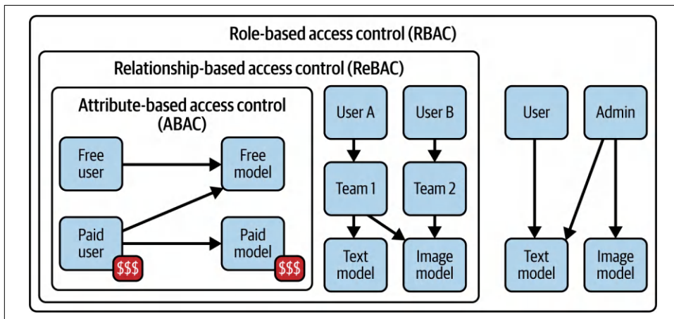
Figure 8-11. Authorization models
