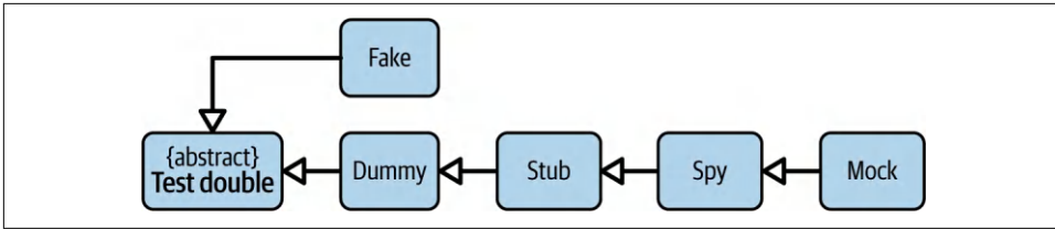
Figure 11-9. Test doubles
