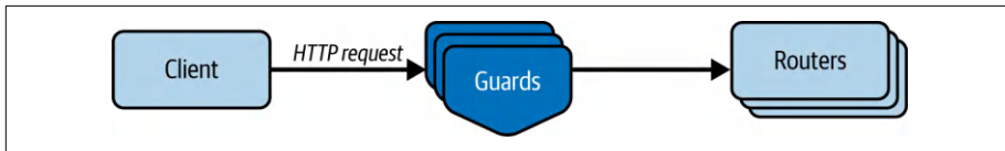
Figure 2-8. Guards
