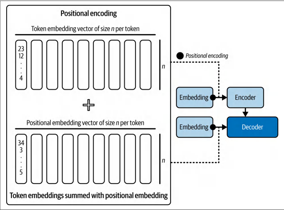
Figure 3-9. Positional encoding
