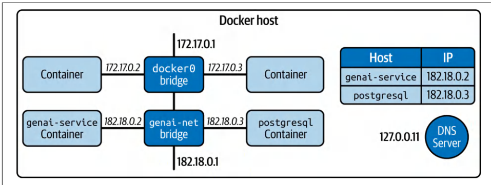
Figure 12-11. Embedded DNS
