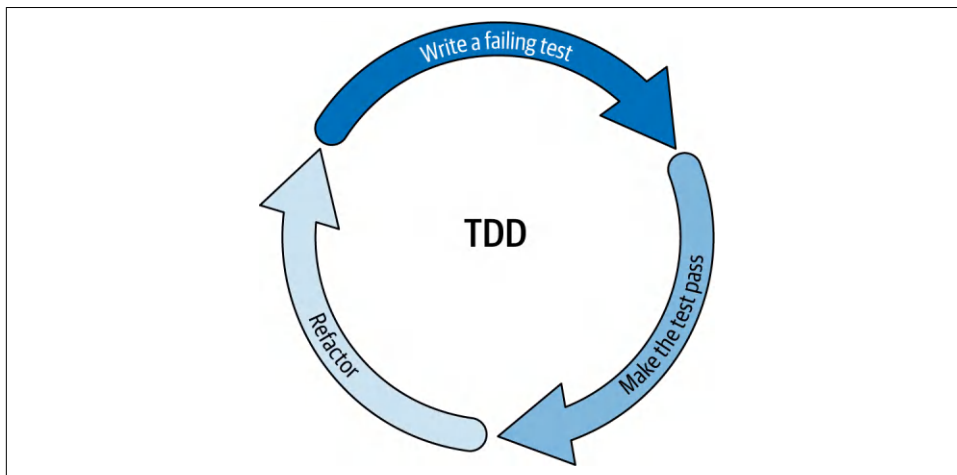
Figure 11-4. TDD
