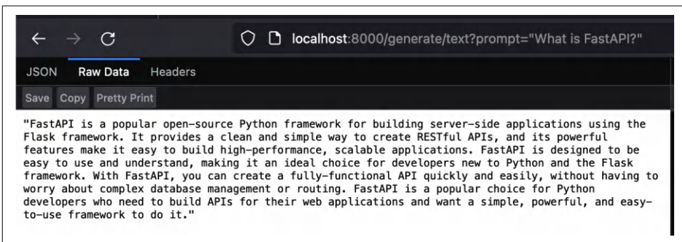
Figure 3-11. Response from TinyLlama
