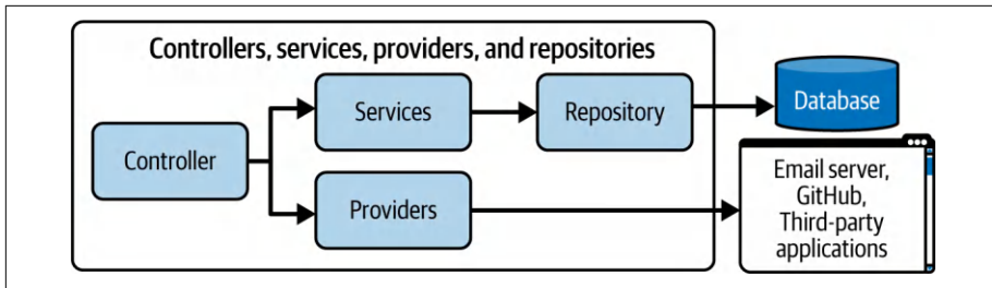
Figure 2-5. Services, providers, and repositories
