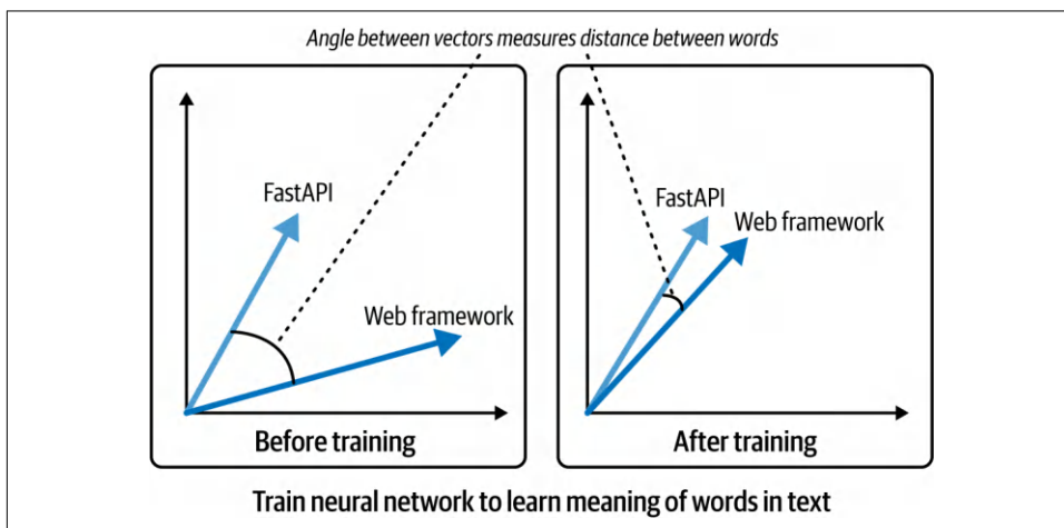
Figure 3-7. Training latent space of transformer network using embedding vectors
