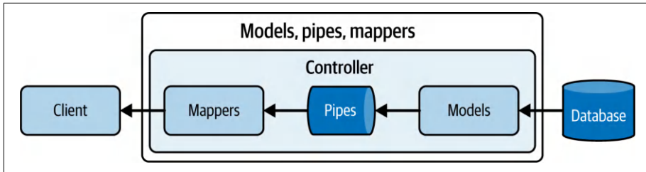
Figure 2-7. Models, pipes, and mappers
