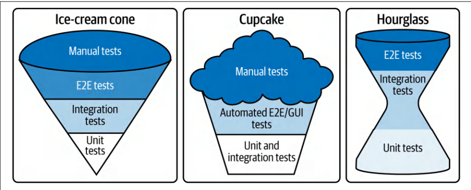
Figure 11-6. Visualization of testing anti-patterns
