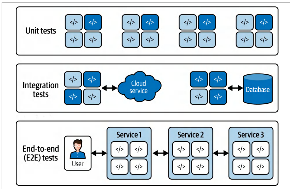
Figure 11-1. Types of tests in software testing
