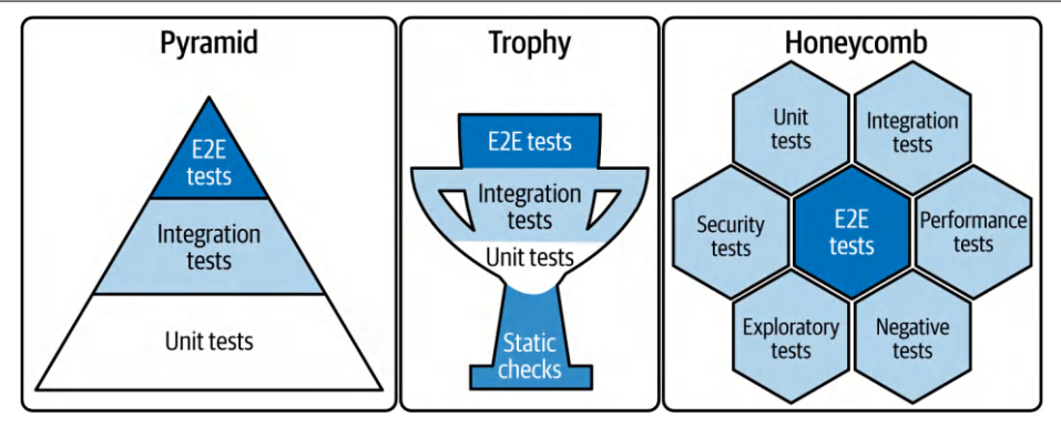
Figure 11-7. Visualization of testing strategies
