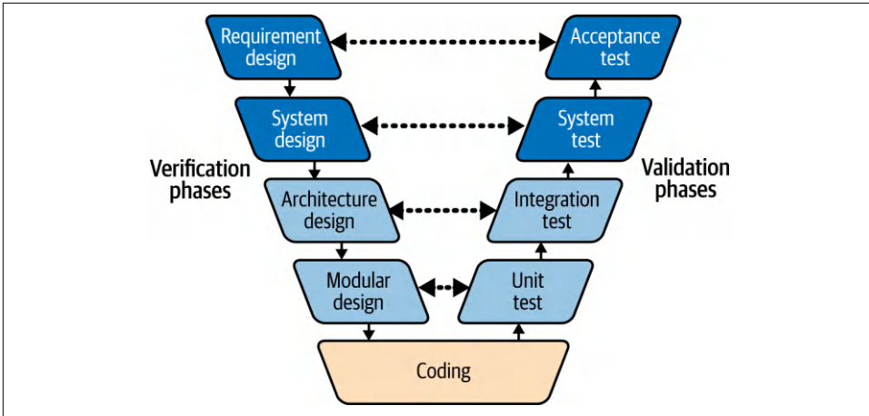
Figure 11-2. Verification and validation model
