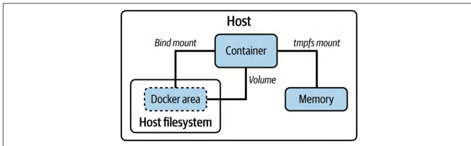
Figure 12-7. Docker storage mounts
