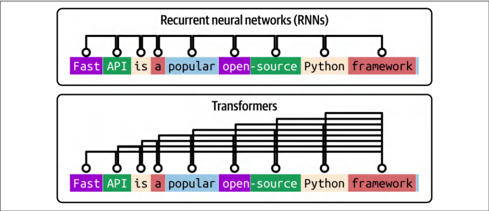
Figure 3-2. RNNs versus transformers in processing sentences
