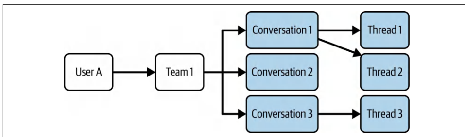
Figure 8-14. Example ReBAC where a user can see the team's private conversations and threads
