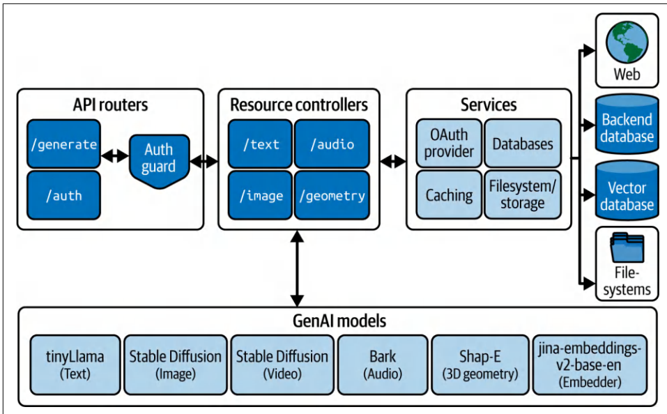
Figure 2-9. Generative AI service you’ll build with FastAPI
