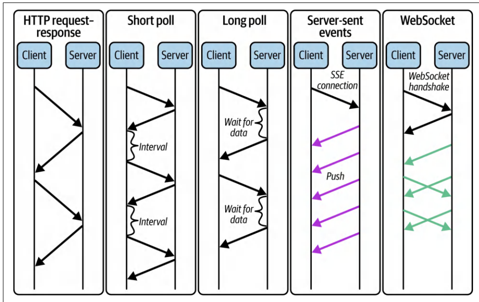
Figure 6-7. Comparison of web communication mechanisms
