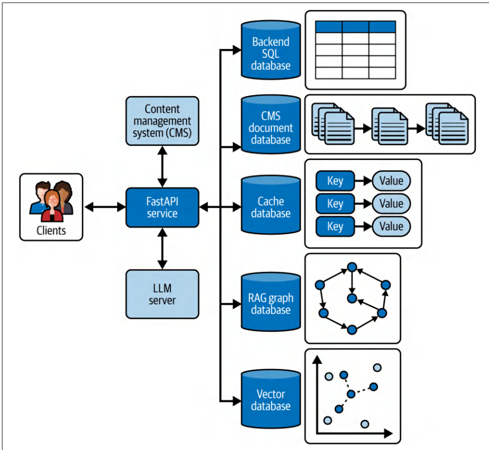
Figure 7-3. Using various database types together
