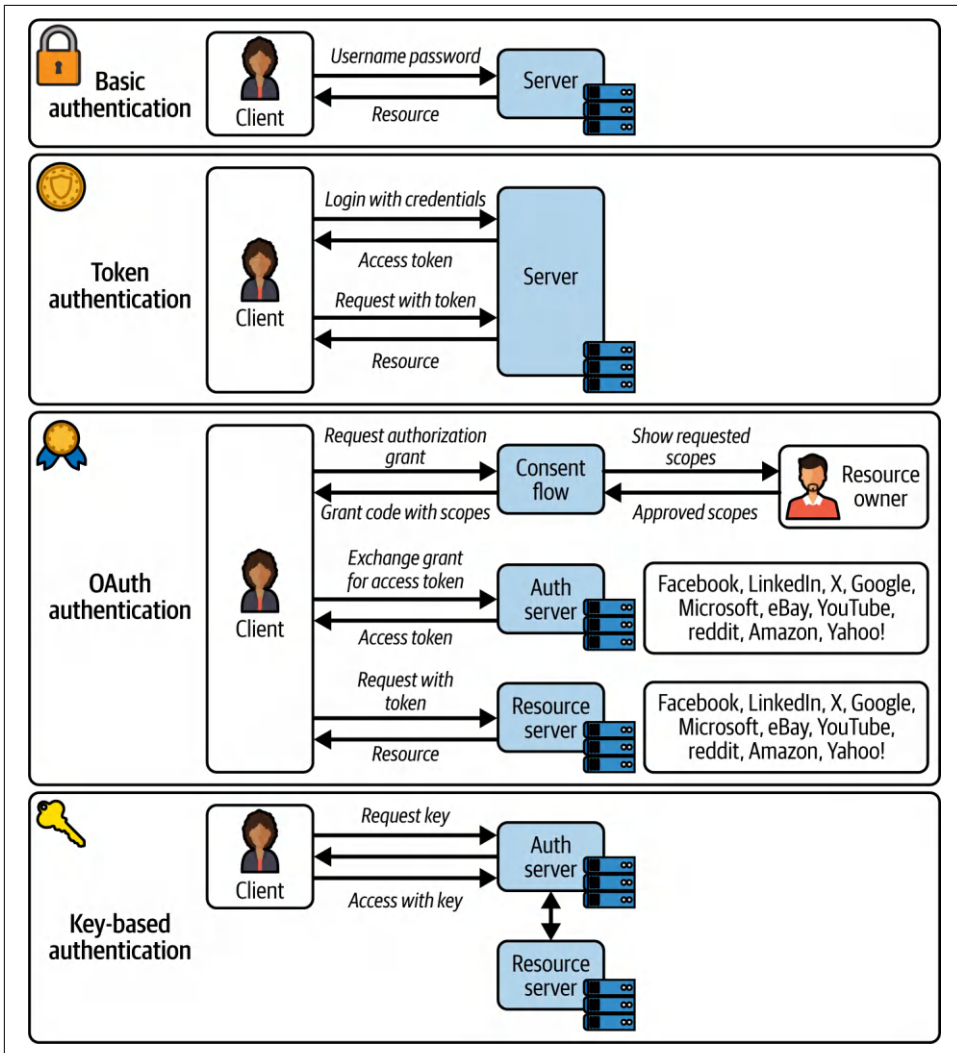
Figure 8-1. Authentication methods
