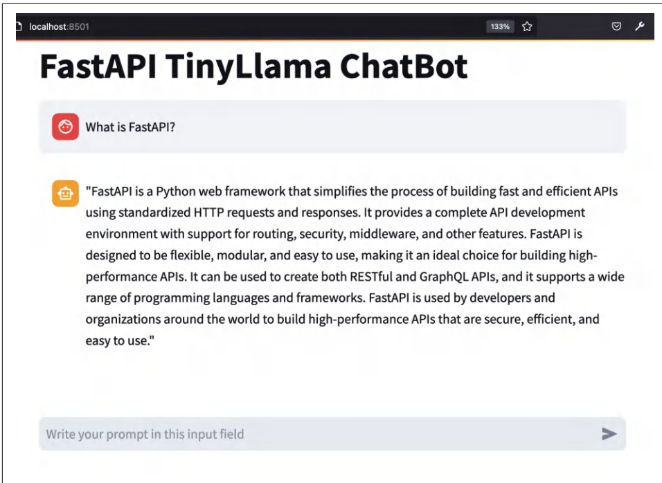
Figure 3-12. Streamlit client
