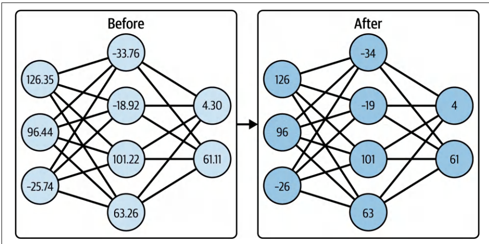
Figure 10-5. Quantization
