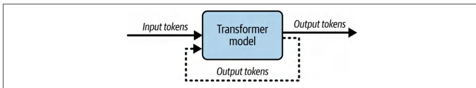
Figure 5-13. Autoregressive prediction
