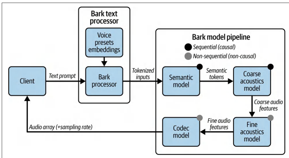
Figure 3-15. Bark synthesis pipeline
