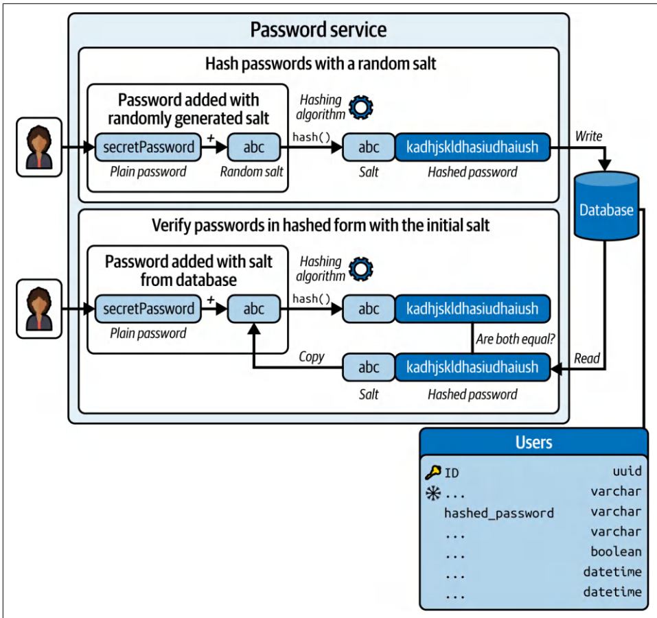
Figure 8-6. Password hash salting mechanism
