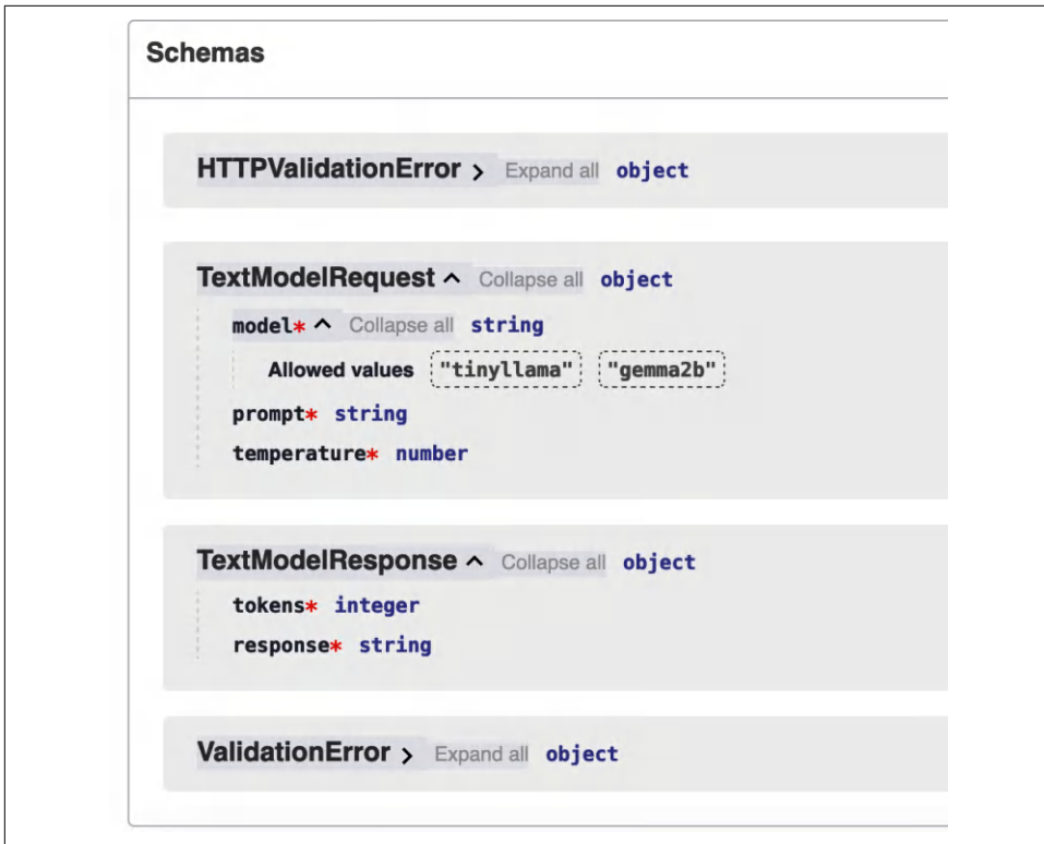
Figure 4-2. Automatic generation of validation schemas using vanilla dataclasses
