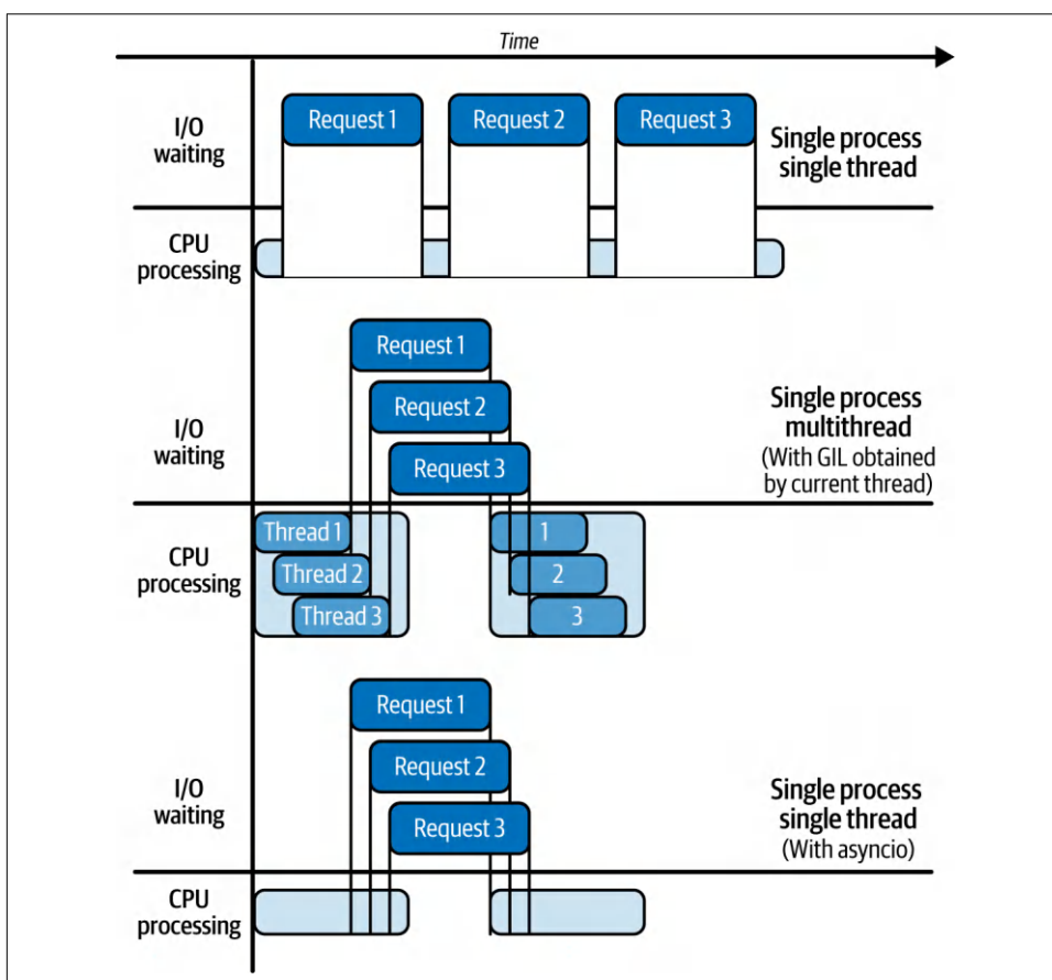
Figure 5-5. How multithreading and Async IO handle I/O blocking operations
