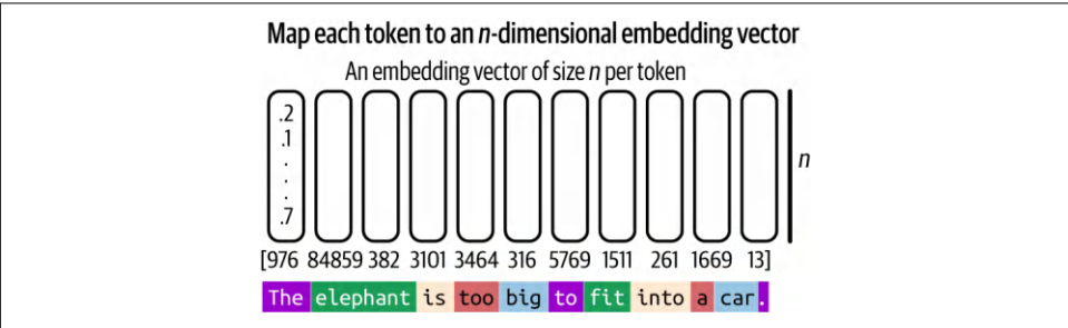
Figure 3-6. Assigning an embedding vector of size n to each token during the embedding process
