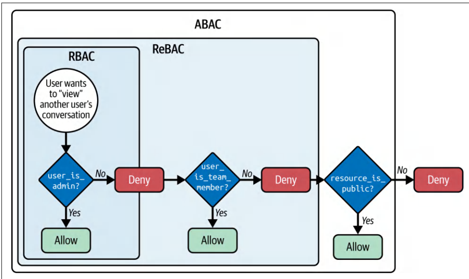
Figure 8-16. Hybrid authorization model based on roles, relationships, and attributes
