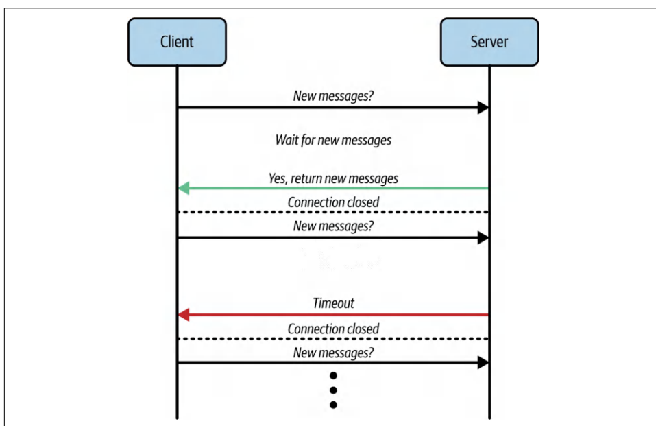
Figure 6-3. Long polling
