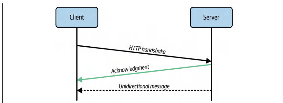
Figure 6-4. SSE
