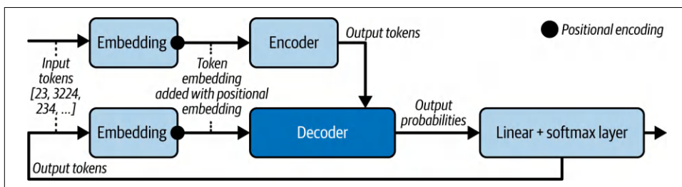
Figure 3-1. Transformer architecture
