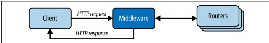
Figure 2-6. Middleware
