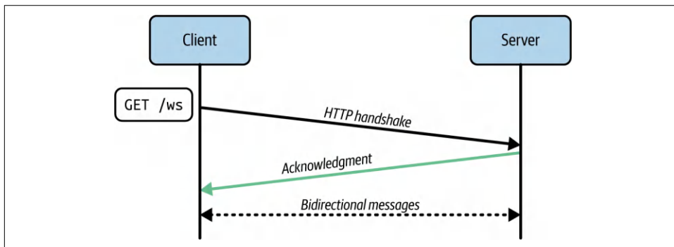
Figure 6-5. WS communication
