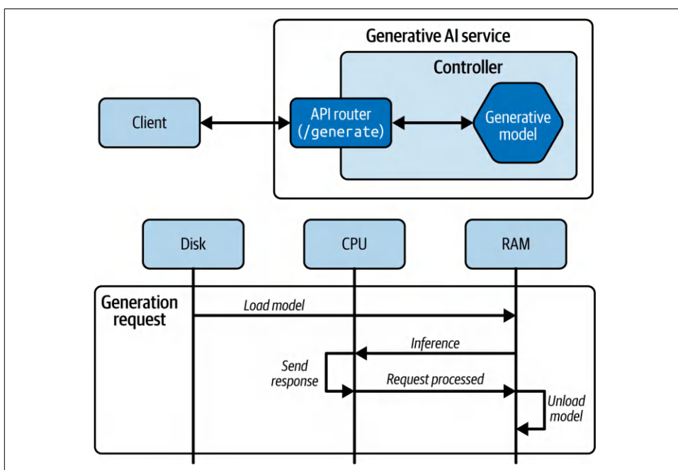
Figure 3-28. Loading and using models on every request
