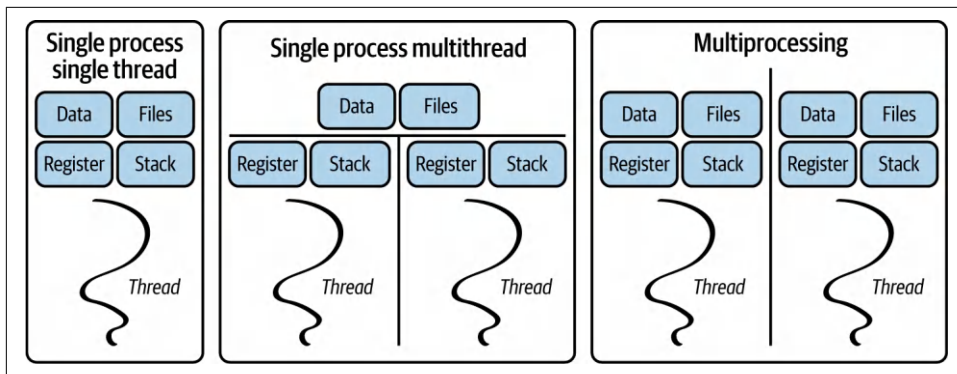
Figure 5-3. Resource sharing in multithreading and multiprocessing
