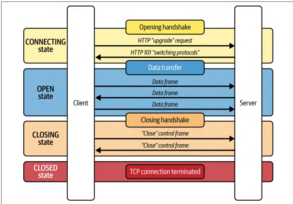
Figure 6-6. WebSocket connection lifecycle
