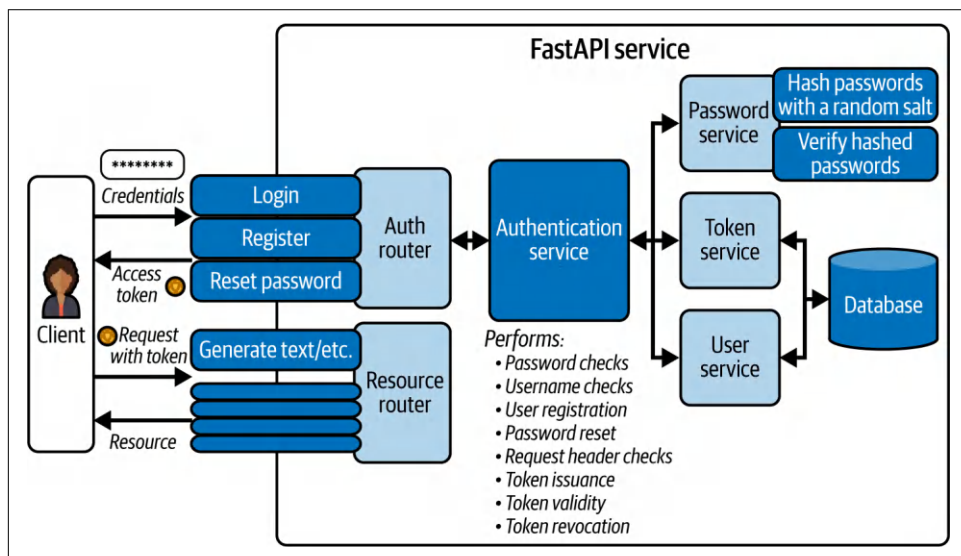
Figure 8-5. JWT authentication system architecture
