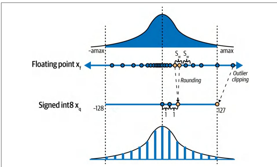
Figure 10-7. Quantization of floating-point numbers to integers
