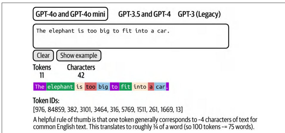
Figure 3-5. OpenAI tokenizer (Source: OpenAI )
