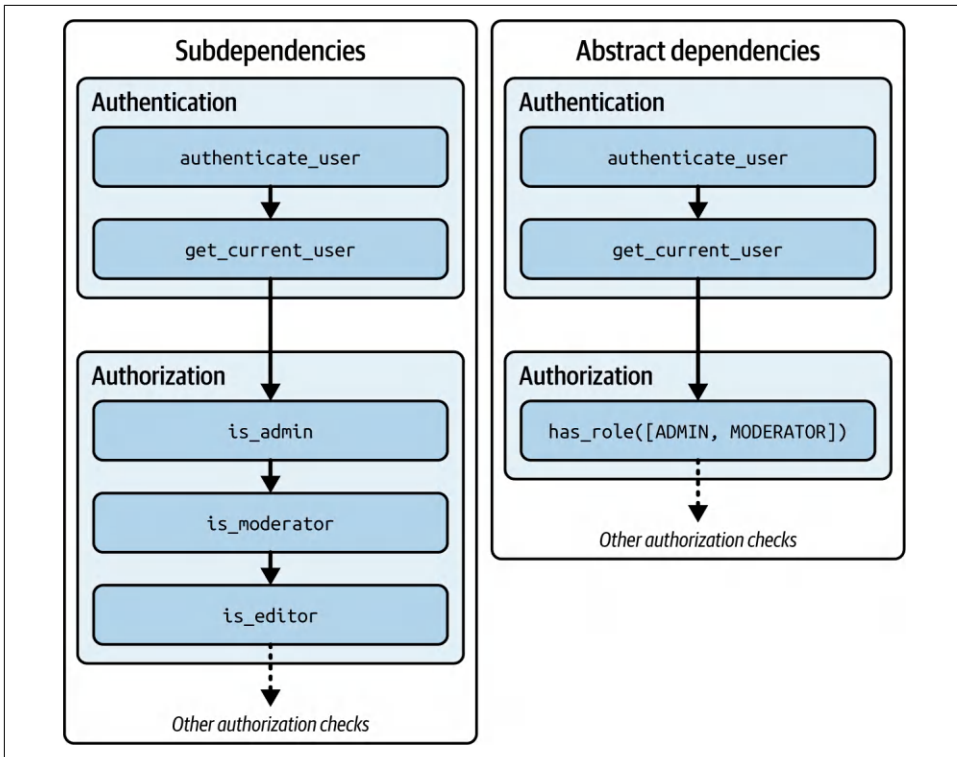
Figure 8-13. Approaches for implementing complex RBAC models
