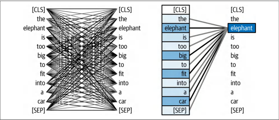
Figure 3-3. View of an attention map inside an attention head
