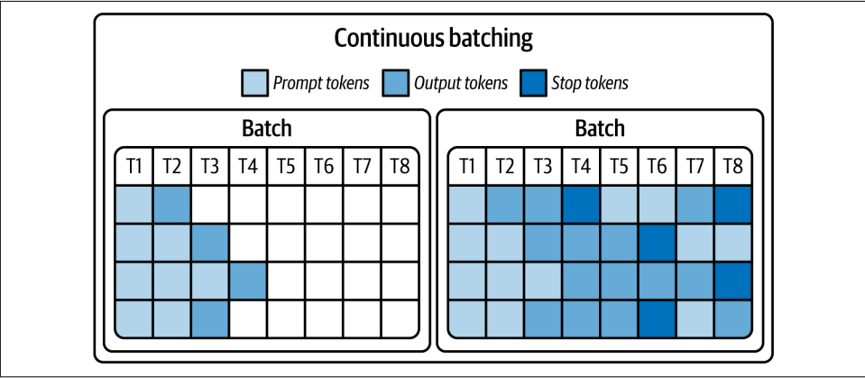
Figure 5-16. Dynamic/continuous batching with variable batch size
