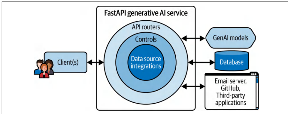
Figure 1-4. FastAPI web server with data source integrations that serve a generative model
