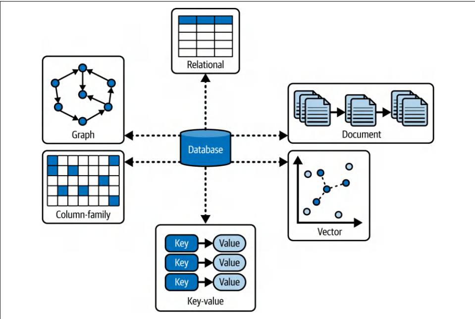
Figure 7-2. Database types
