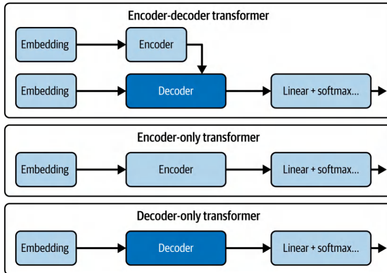
Figure 3-14. Transformer architectures
