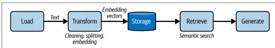
Figure 5-8. RAG pipeline
