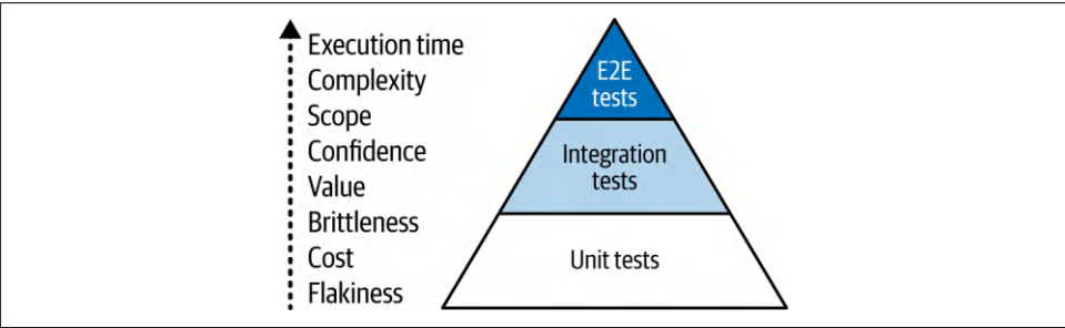
Figure 11-5. Testing pyramid
