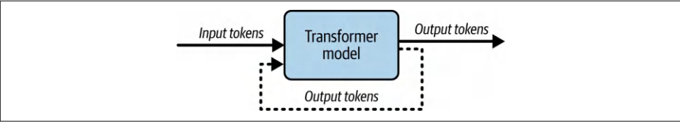
Figure 3-10. Autoregressive prediction
