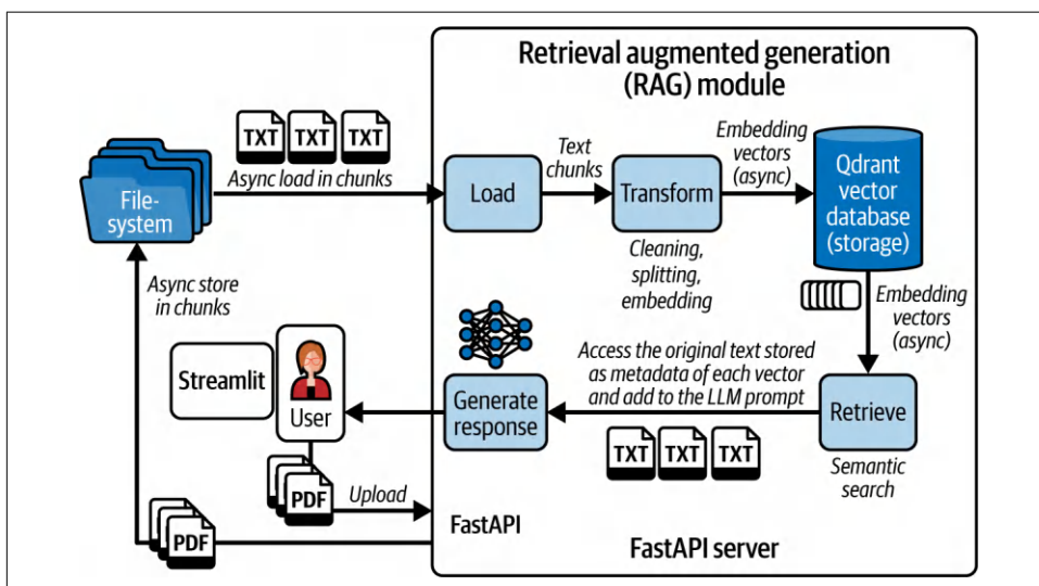
Figure 5-9. Talk to your documents system architecture
