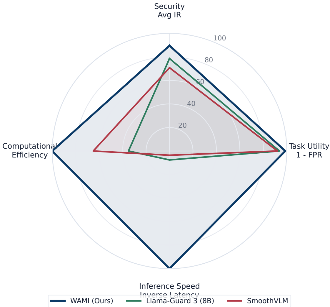
Fig. 3. Defense Efficacy Overview
