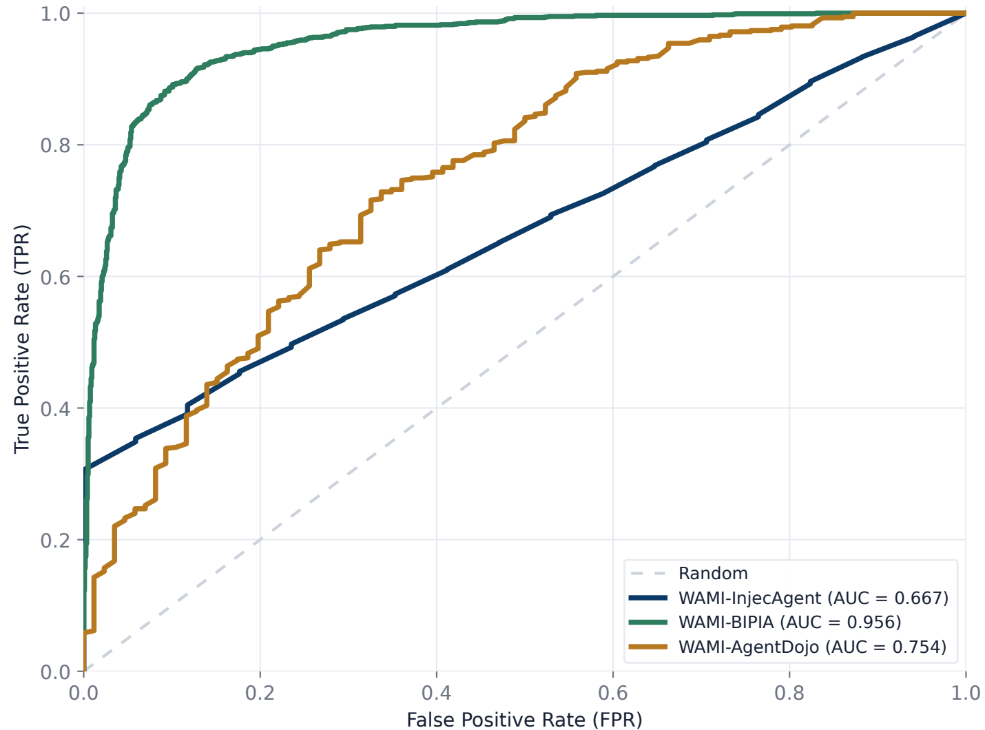
WAMI ROC Curves on Local Test Sets
