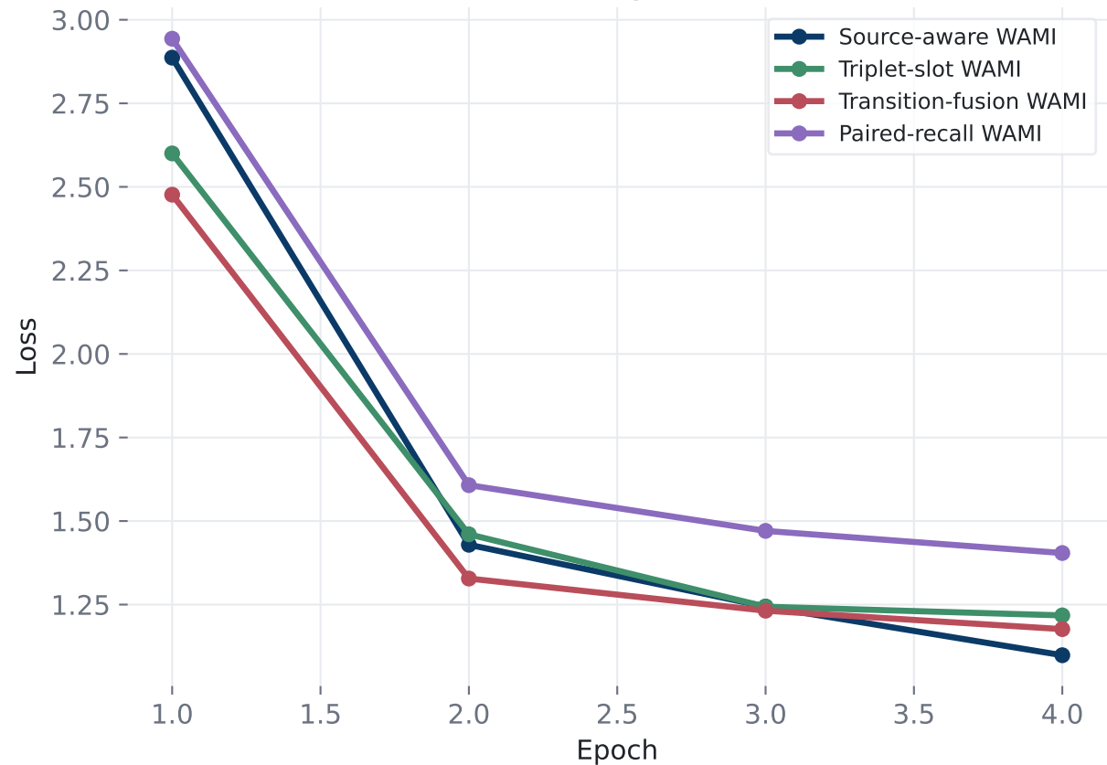
Training loss
