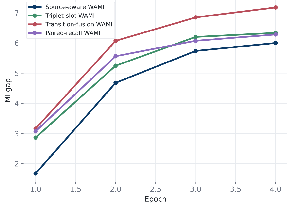
MI gap during shadow training
