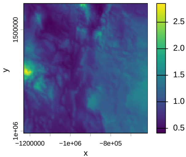
SD, bio12
