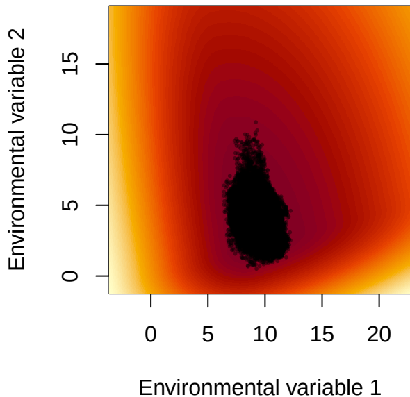
Presences (occ == 1)
