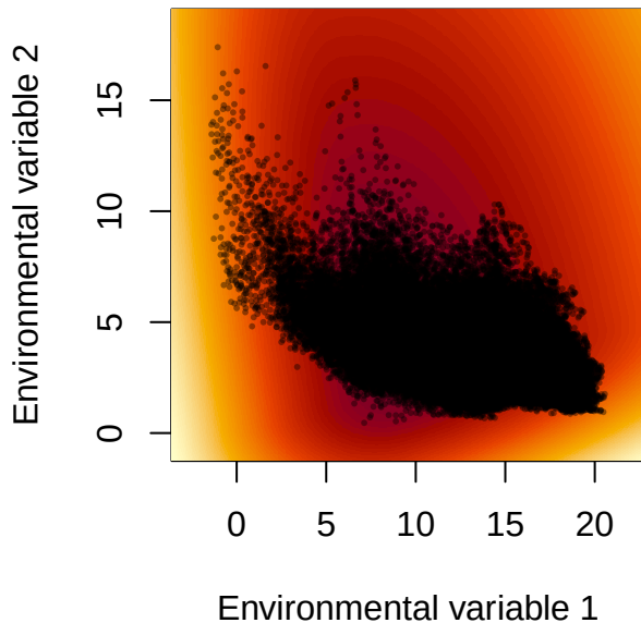
Non-detections (occ == 0)
