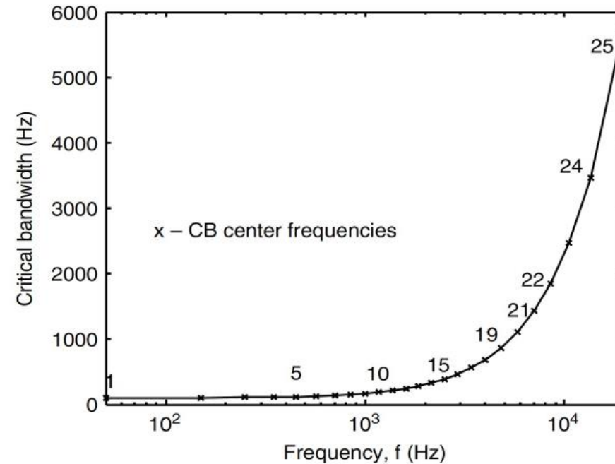
Critical bandwidth as a function of center frequency
