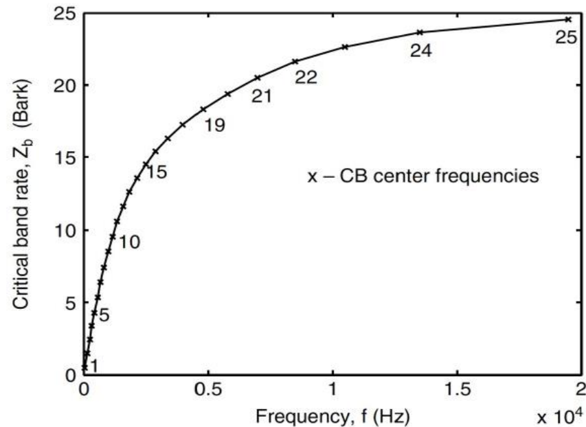
Critical band mapping from Hz to Bark
