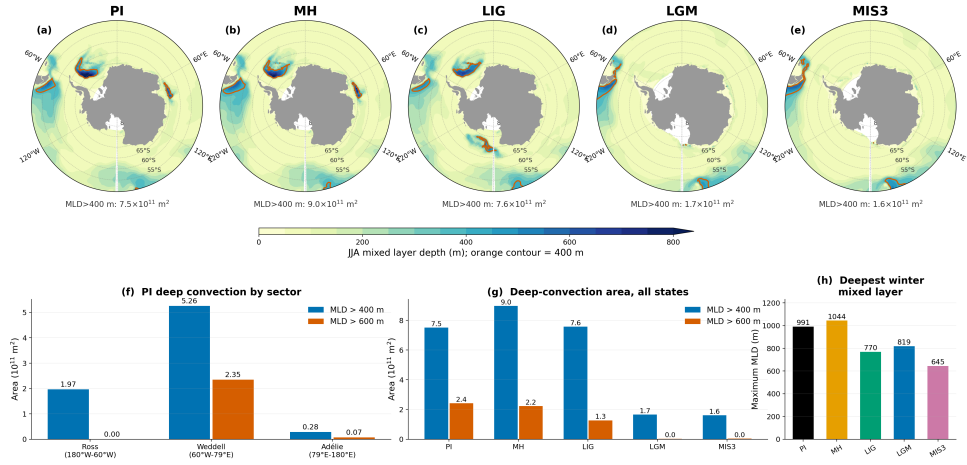
Figure R2.4 (new analysis). Where the model actually convects. (a-e) Winter mixed layer depth, 400 m contour in orange. (f) In the pre-industrial state 70% of the area with a mixed layer deeper than 400 m, and 97% of the area deeper than 600 m, lies in the Weddell sector, centred near 68^\circ\text{S} in the open gyre rather than over the shelf. (g, h) The deep-convection area and the maximum mixed layer depth both contract sharply in the glacial states. We now say this plainly in the Discussion, note that it is a limitation shared across the current
