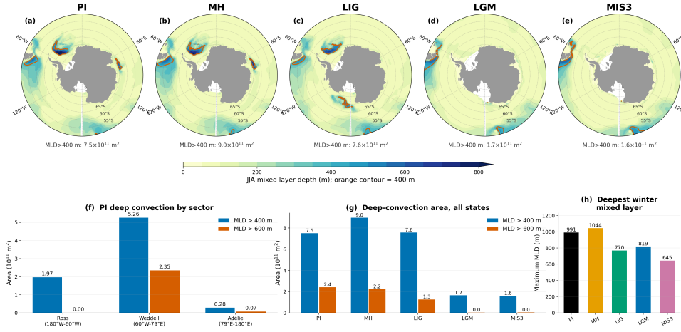
Figure R3.1 (new analysis). (a-e) Winter mixed layer depth with the 400 m contour in orange. (f) The pre-industrial sector breakdown, showing that convection is concentrated in the Weddell gyre interior rather than on the shelf, which is the bias the reviewer identified. (g, h) The glacial contraction of both the deep-convection area and the maximum mixed-layer depth. The model therefore does form its dense water by open-ocean convection, as the reviewer supposed. We now state this explicitly, cite Orsi et al. (1999) and Toggweiler and Samuels (1995) for the shelf pathway that operates in the real ocean, note that this configuration has no ice shelf cavities and therefore cannot represent basal melt at all, and place the model in context by citing Heuzé (2021), who finds 28 of 35 CMIP6 models forming deep and bottom water by open-ocean convection with no model showing convincing shelf export in the Weddell Sea.
