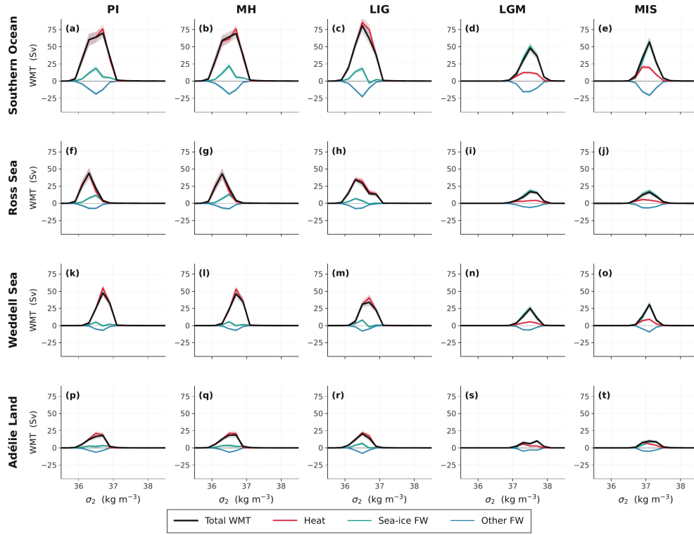
Figure R1.7 (new Supplementary Fig. S5). Winter transformation for the four sectors and five climate states on a common vertical and horizontal axis. Plotted this way the glacial weakening of the transformation maximum and its shift to denser classes are directly comparable between panels, which the independently scaled main-text version does not allow. 16. Line 174: "Section 4?" If this is intended to refer to the Methods section. — Corrected to refer to the Methods section by name. 17. Fig.3 Please consider adding the climate-state labels at the top of each column, as in the other figures. — Added, here and on the other multi-panel figures; Reviewer 3 made the same request.
