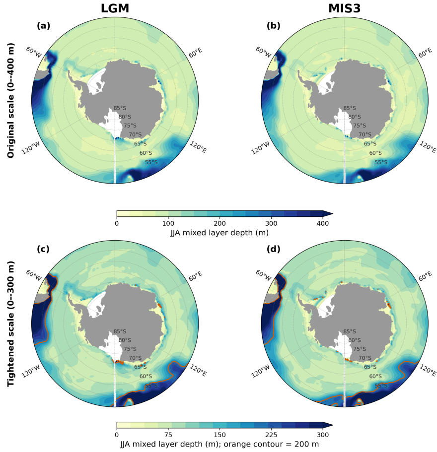
Figure R1.5 (new supplementary panel). LGM and MIS3 winter mixed layer depth on the original 0–400 m scale (top) and on a tightened 0–300 m scale with the 200 m contour marked (bottom). The tightened scale resolves discrete deep cells along the coast, in the Weddell, Prydz Bay and Ross sectors, which is where the glacial dense water is produced. This is the figure we now use in the supplement.
