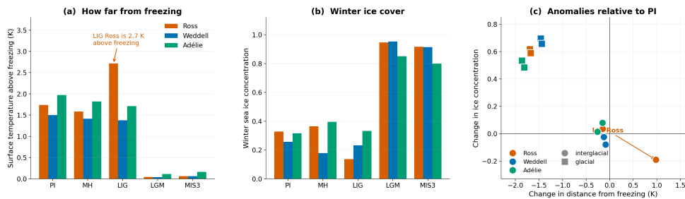
Figure R1.6 (new analysis). (a) Winter surface temperature above the local freezing point and (b) winter sea ice concentration, by sector and climate state. (c) The same quantities as anomalies relative to PI. The Ross sector separates from the others only in the last interglacial, where it warms to 2.7 K above freezing and loses 0.19 of ice concentration, an order of magnitude more than the Weddell or Adélie response. In the glacial states all three sectors collapse onto the freezing point and gain ice comparably.
