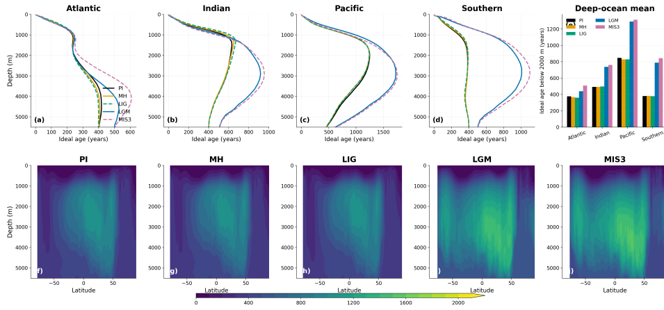
Figure R3.7 (manuscript Fig. 7). Basin-mean ideal age profiles (a-d), mean age below 2000 m (e), and zonal-mean sections for the five states (f-j). The glacial ageing is concentrated
