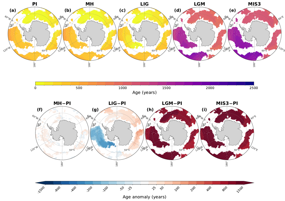
Figure R1.4 (revised manuscript figure). The ventilation age figure as an example of the labelling now applied throughout. Every panel carries labelled latitude circles and labelled meridians, and the climate state is named above each panel. The mixed layer, wind stress and composite figures have been treated the same way; please refer to the revised manuscript and supplement for the complete set.
