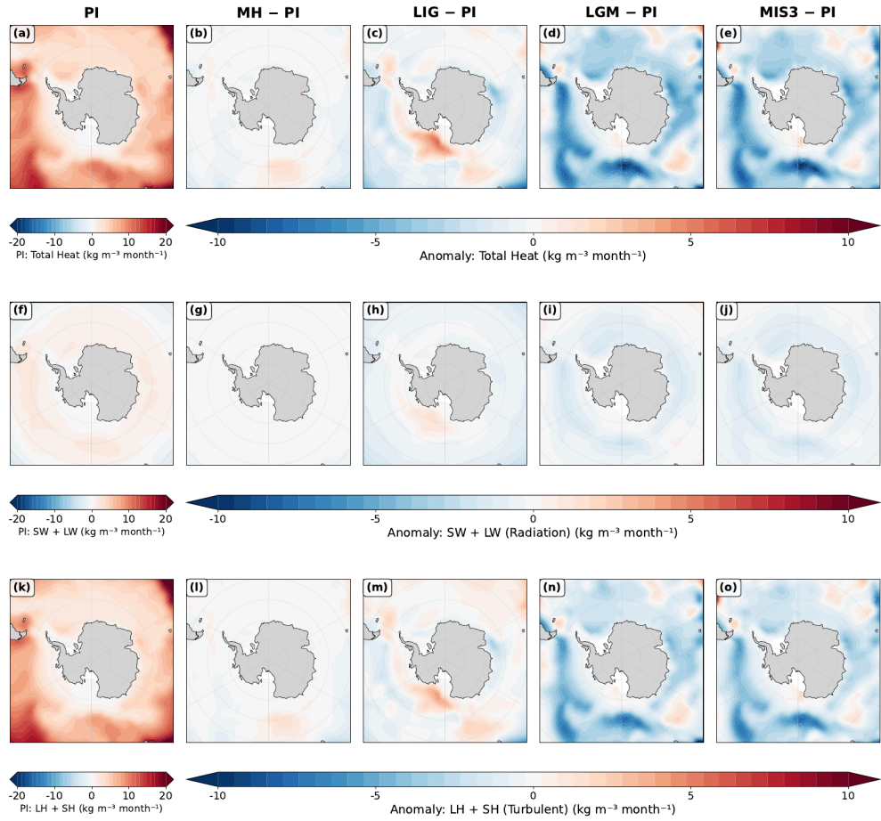
Figure R1.8 (revised manuscript Fig. 3). The surface density tendency figure with the climate-state headings added, so that the columns are identified in the same way as in the other figures. The freshwater counterpart, Fig. 4, has been given the same headings.
