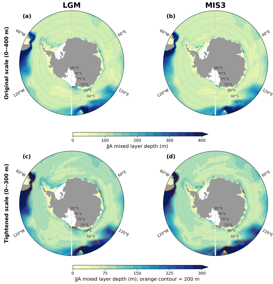
Figure R1.3 (new supplementary panel). LGM and MIS3 winter mixed layer depth on the original 0-400 m scale (top) and on a tightened 0-300 m scale with the 200 m contour marked (bottom). The 99th percentile of the glacial winter mixed layer south of 55 deg S is only 280 m (LGM) and 296 m (MIS3), which is why the shared interglacial scale leaves the glacial panels almost featureless. The tightened scale resolves the discrete coastal cells where the glacial dense water is produced.
