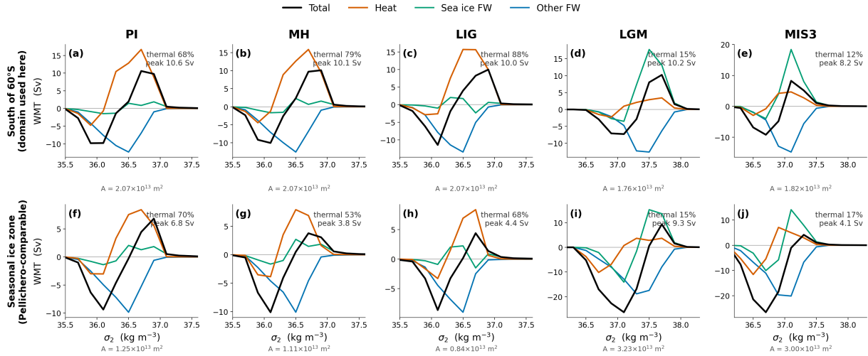
Figure R3.2 (manuscript Fig. 8). The like-for-like comparison the reviewer asked for. Transformation integrated over the published domain south of 60 deg S (top) and over the seasonal sea ice zone that reproduces the observational domain (bottom). The haline share rises in the restricted domain, but the glacial-interglacial contrast is unaffected, which is why we conclude the regime shift is not an artefact of the biased pre-industrial end member.
