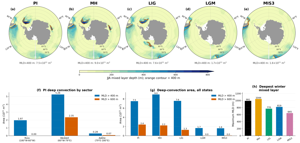
Figure R1.2 (new analysis). (a-e) Winter mixed layer depth for the five states, with the 400 m contour in orange. (f) In the pre-industrial state the Weddell sector accounts for 70% of the area with a mixed layer deeper than 400 m and 97% of the area deeper than 600 m, and the convection sits in the interior of the gyre near 68 deg S rather than over the shelf. (g) The deep-convection area contracts to roughly one fifth of its pre-industrial value in the glacial states. (h) The deepest
