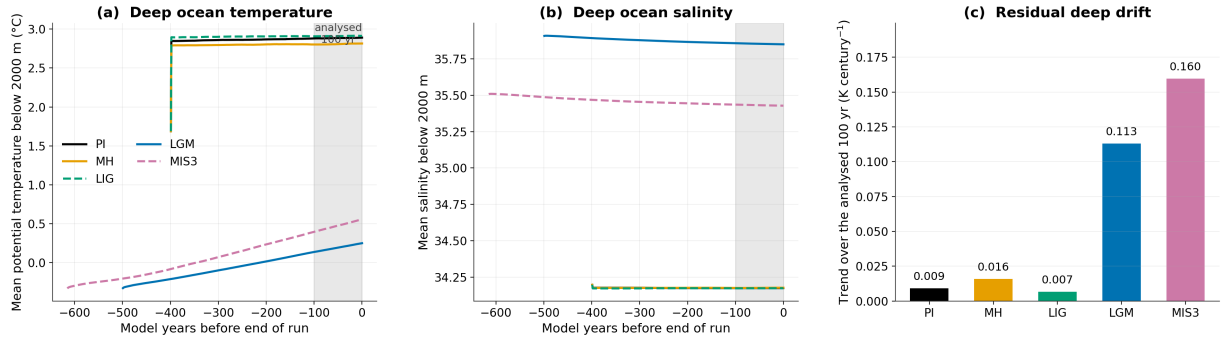
Figure R3.5 (new analysis). Volume-weighted mean (a) potential temperature and (b) salinity below 2000 m over all available output years, with the analysed final century shaded. (c) The residual trend over that century. The interglacial deep ocean is flat and still decelerating, with the trend over the second half of each record 0.13 to 0.41 times that over the first half. The two glacial experiments are further from equilibrium: they drift at 0.113 and 0.160 K per century, warm by 0.58 and 0.89 K over the record, and are not decelerating.
