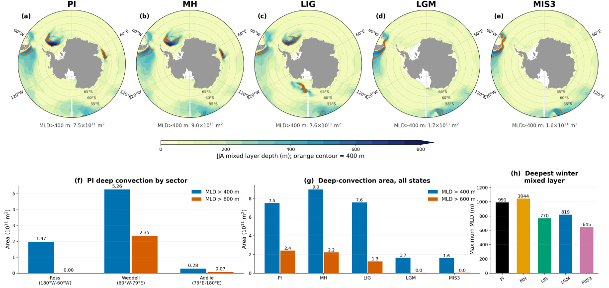
Figure R2.3 (new analysis). Where the model actually convects. (a-e) Winter mixed layer depth, 400 m contour in orange. (f) In the pre-industrial state 70% of the area with a mixed layer deeper than 400 m, and 97% of the area deeper than 600 m, lies in the Weddell sector, centred near 68 deg S in the open gyre rather than over the shelf. (g, h) The deep-convection area and the maximum mixed layer depth both contract sharply in the glacial states. We now say this plainly in the Discussion, note that it is a limitation shared across the current model generation rather than specific to AWI-ESM2 (Heuzé, 2021: 28 of 35 CMIP6 models), and state that this configuration has no ice shelf cavities.
