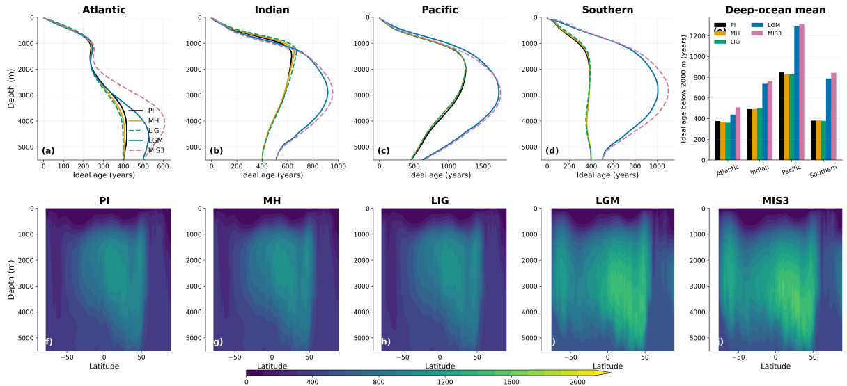
Figure R3.7 (manuscript Fig. 7). Basin-mean ideal age profiles (a-d), mean age below 2000 m (e), and zonal-mean sections for the five states (f-j). The glacial ageing is concentrated below about 2000 m and is largest in the deep Pacific and Southern Ocean, while the Atlantic, which remains ventilated from the north, changes comparatively little.
