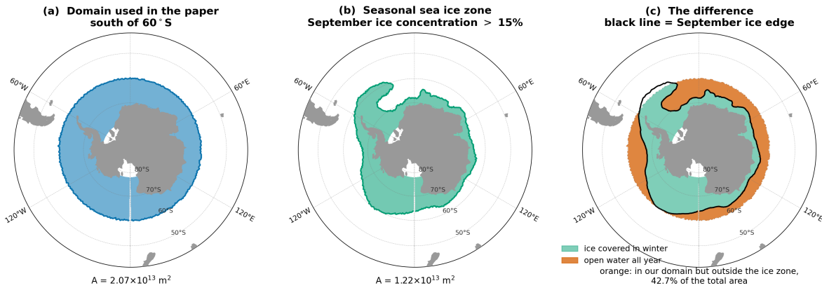
Figure R2.1 (new analysis). (a) The domain used in the submitted manuscript, everything south of 60 deg S, covering 2.07 \times 10^{13} \text{ m}^2 . (b) The seasonal sea ice zone of the model, inside the September 15% contour, which is the definition Pellichero et al. use, covering 1.22 \times 10^{13} \text{ m}^2 . (c) The two overlaid. The orange ring is inside our domain but outside the ice zone: it is 42.7% of the area we integrated over, it is open water all year, and it is water their analysis does not include.
