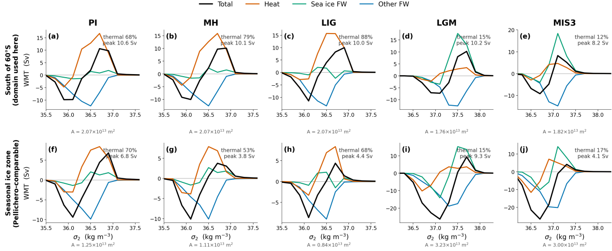
Figure R2.2 (manuscript Fig. 8). Transformation integrated south of 60 deg S, the domain used in the submitted version (top row), and over the seasonal sea ice zone alone, which reproduces the domain of Pellichero et al. to within 2.5% in area (bottom row). Restricting the integration to the ice-covered sector raises the haline share, as the reviewer would expect, but the contrast between thermally dominated interglacials and haline dominated glacials survives intact.
