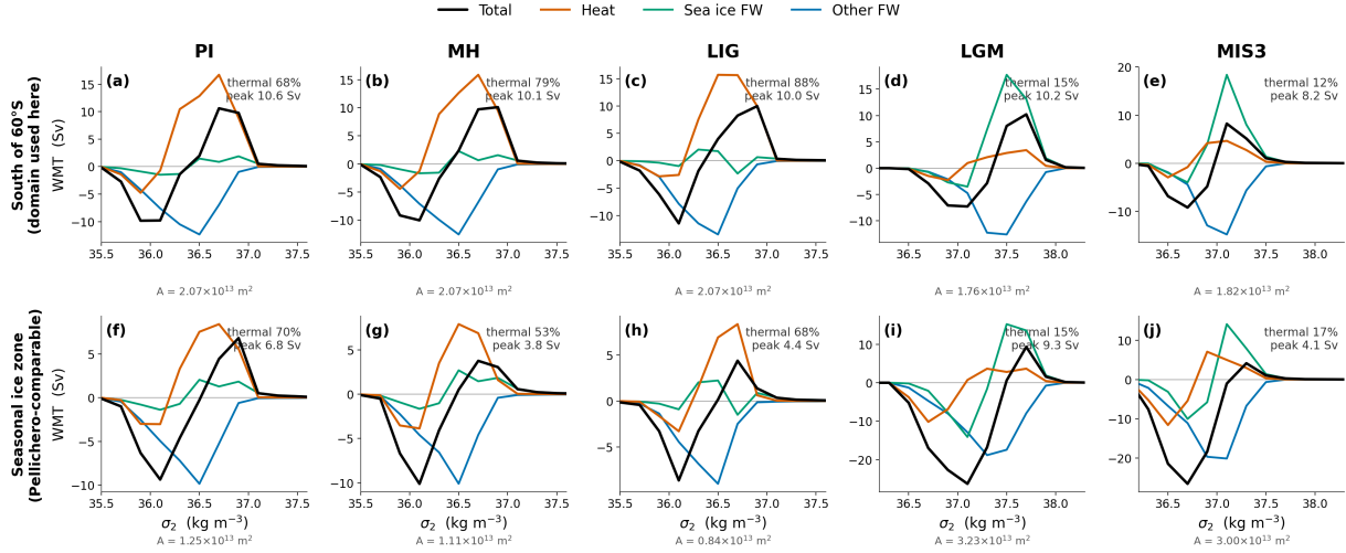
Figure R1.1 (manuscript Fig. 8). Transformation integrated south of 60 deg S, the domain used in the submitted version (top row), and over the seasonal sea ice zone alone, which reproduces the domain of Pellichero et al. to within 2.5% in area (bottom row). The thermal share at the transformation maximum and the area of each domain are given in each panel. The haline share increases in the restricted domain, as expected, but the contrast between thermally dominated interglacials and haline dominated glacials is unchanged.
