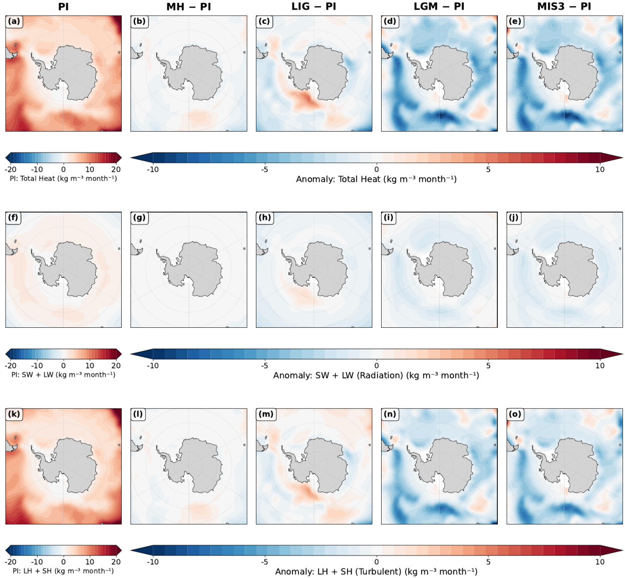
Figure R1.8 (revised manuscript Fig. 3). The surface density tendency figure with the climate-state headings added, so that the columns are identified in the same way as in the other figures. The freshwater counterpart, Fig. 4, has been given the same headings.
