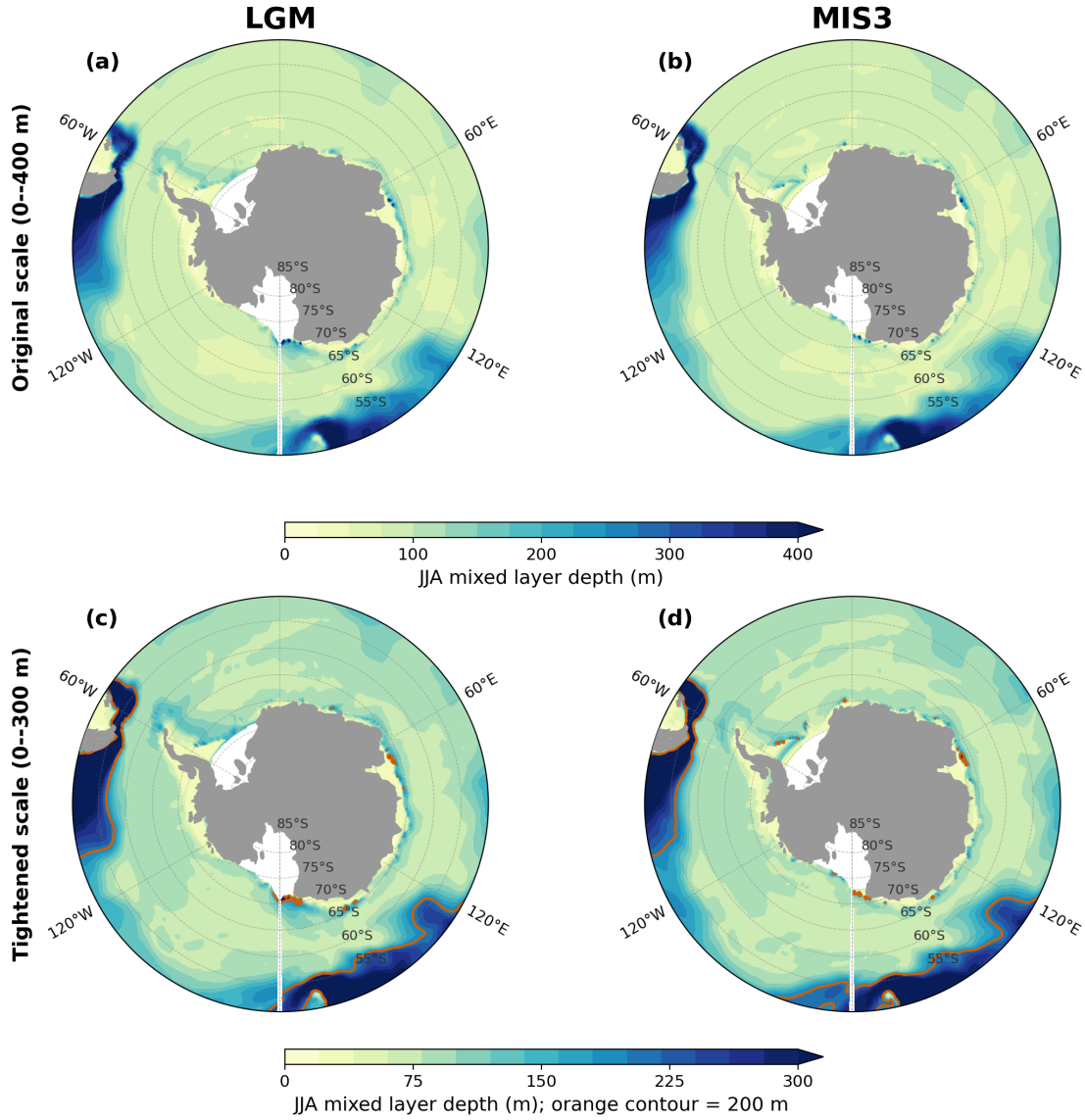
Figure R1.4 (new supplementary panel). LGM and MIS3 winter mixed layer depth on the original 0-400 m scale (top) and on a tightened 0-300 m scale with the 200 m contour marked (bottom). The tightened scale resolves discrete deep cells along the coast, in the Weddell, Prydz Bay and Ross sectors, which is where the glacial dense water is produced. This is the figure we now use in the supplement.
