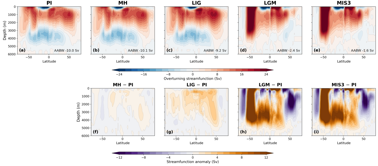
Figure R3.5 (manuscript Fig. 6). Global overturning streamfunction for the five climate states (top) and anomalies relative to PI (bottom). The blue abyssal cell, representing northward spreading of southern-sourced bottom water, nearly disappears in the glacial states while the upper cell is largely maintained.
