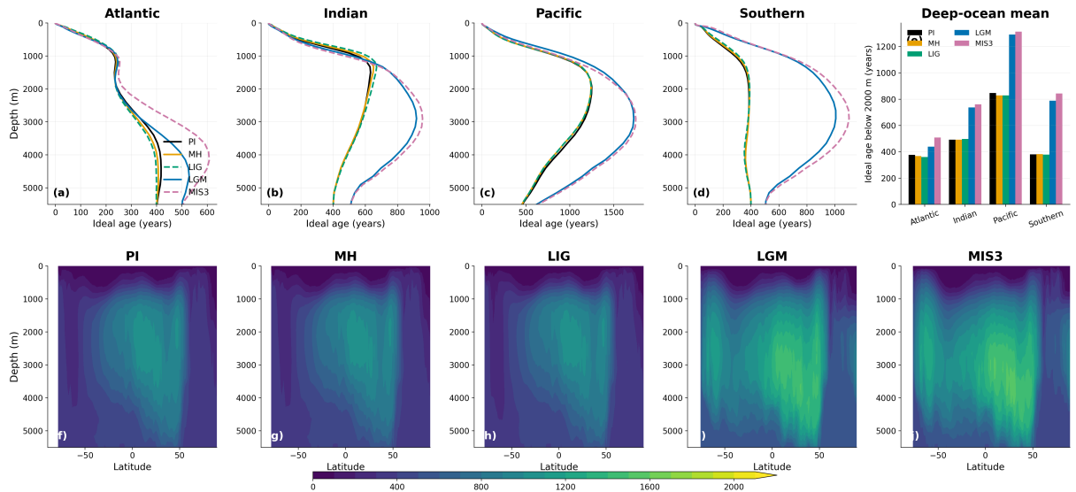
Figure R3.6 (manuscript Fig. 7). Basin-mean ideal age profiles (a-d), mean age below 2000 m (e), and zonal-mean sections for the five states (f-j). The glacial ageing is concentrated below about 2000 m and is largest in the deep Pacific and Southern Ocean, while the Atlantic, which remains ventilated from the north, changes comparatively little.
