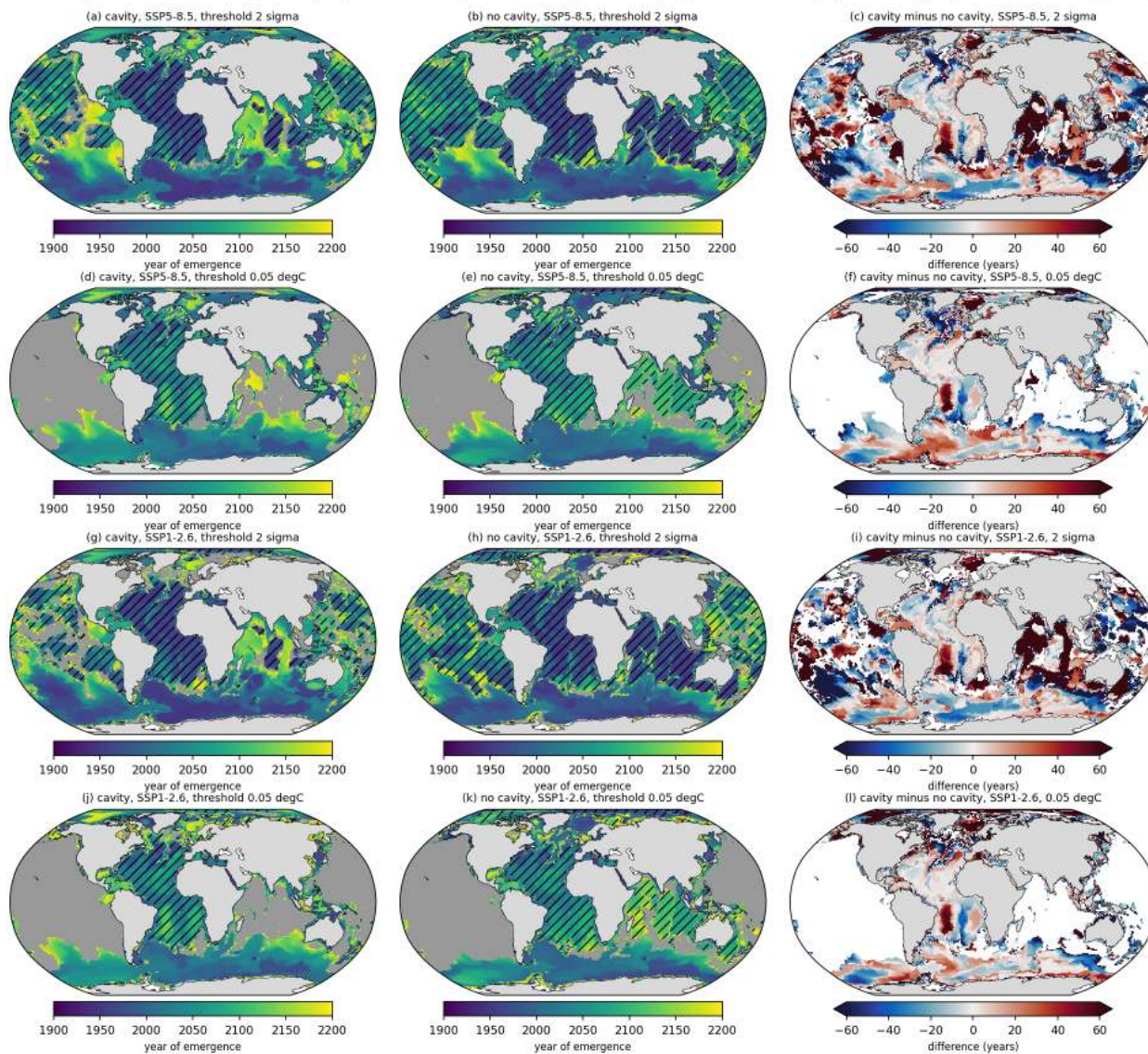
Figure 171: fig08_toe_btemp_maps (propagation). Time of emergence of the bottom temperature signal, defined as the first year from which the 11-yr running mean of the drift-corrected anomaly stays permanently beyond a threshold until 2195. Rows are SSP5-8.5 with a 2 sigma threshold (sigma = std of the detrended 1851-1950 annual values per node), SSP5-8.5 with an absolute threshold of 0.05 degC, and the same two for SSP1-2.6. Columns are cavity, no cavity and cavity minus no cavity (years). Grey means not emerged by 2195 and hatching marks emergence with a negative sign (cooling). Take-away. Abyssal interannual noise is tiny (median sigma 0.003 degC below 3000 m), so with the 2 sigma criterion 44 to 53 percent of the deep sea floor has emerged by 2014 and 92 to 97 percent by 2200. With the 0.05 degC criterion the Southern Ocean south of 45S emerges between 2005 and 2060, the Atlantic abyss (cooling) between 2020 and 2080, and the Pacific and Indian abyss north of 40S never emerge. The cavity and no-cavity emergence years differ by less than 20 years over most of the deep ocean.
