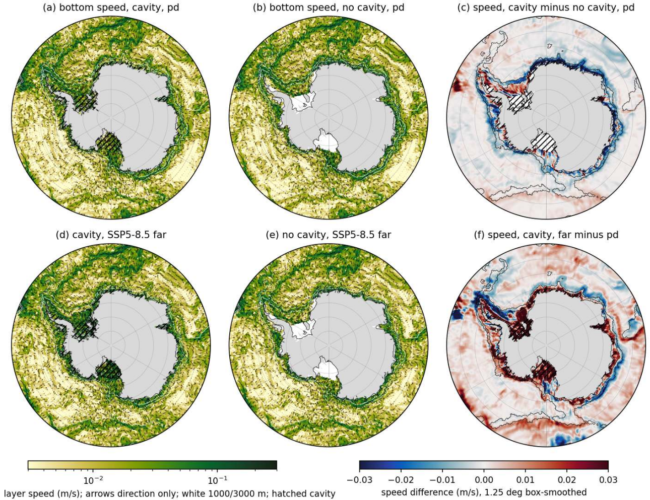
Figure 119: circ_bottom_velocity (circ). Bottom-layer (deepest wet layer of each element) speed (log colour) with direction arrows south of 55S; white contours 1000 and 3000 m isobaths, hatched = ice-shelf cavities. (a) cavity pd, (b) no cavity pd, (c) speed difference cavity minus no cavity (1.25 degree box smoothed), (d) cavity SSP5-8.5 far, (e) no cavity SSP5-8.5 far, (f) cavity far minus pd. Take-away: the strongest bottom flow (0.05-0.3 m/s) is the westward Antarctic Slope Current over the 1000-3000 m band and the cyclonic rims of the Weddell and Ross gyres; there is no distinct down-slope dense plume signature at the Filchner, Ross or Adelie sills. Mean bottom speed over the circumpolar slope band (1000-3000 m, S of 60S) is 0.024 m/s (cavity) versus 0.032 m/s (no cavity), the westward component -0.012 versus -0.019 m/s, so the slope current is about 35 percent weaker in the cavity run (the shelf geometry differs, see caveats). Under SSP5-8.5 the slope current weakens further in the no-cavity run (-0.015 m/s) and is unchanged in the cavity run, while under-ice-shelf currents in the FRIS and Ross cavities accelerate by 0.01-0.03 m/s.
