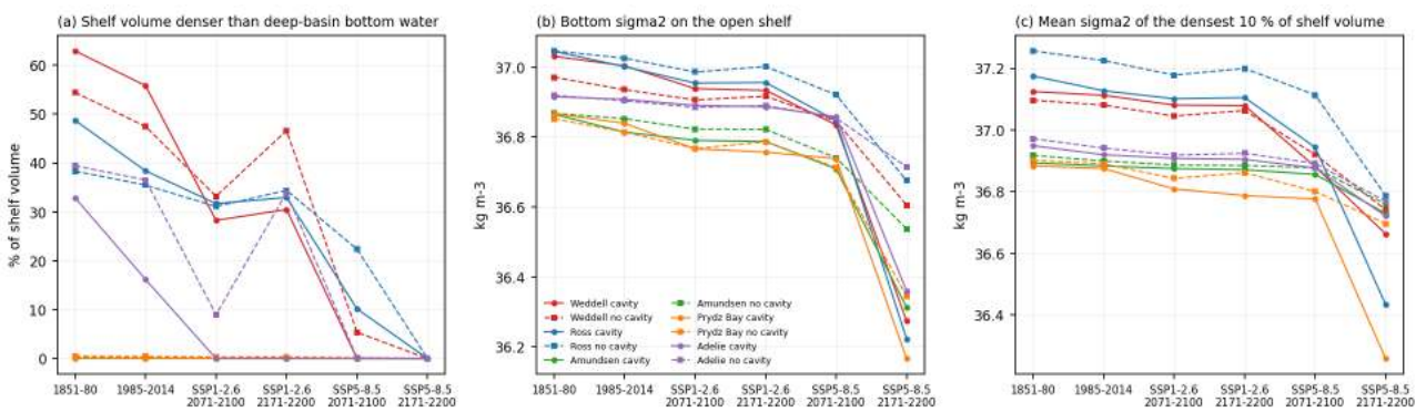
Figure 97: shelf_dense_water (bottom). Dense shelf water summary per shelf region (colours) for the periods 1851-1880, 1985-2014 and the SSP1-2.6 and SSP5-8.5 end and far periods: (a) percent of the open-shelf volume denser than the area-mean bottom sigma2 of the adjacent deep basin, (b) area-mean bottom sigma2 on the shelf, (c) mean sigma2 of the densest 10 percent of the shelf volume. Circles cavity, squares no cavity. Half of the Weddell shelf volume and 35 to 40 percent of the Ross shelf volume is denser than the deep bottom water at present; these fractions drop to 20 to 30 percent under SSP1-2.6 and to zero under SSP5-8.5 by 2100 to 2200.
