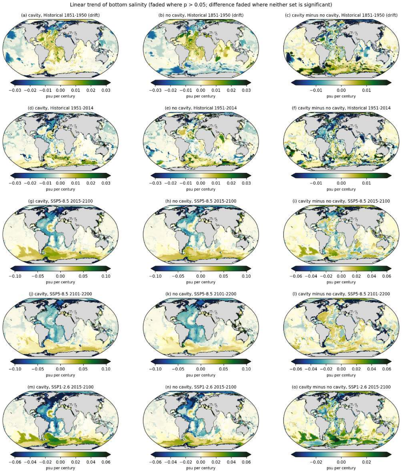
Figure 166: fig03_trend_bsalt_global (propagation). Same layout as fig01 for bottom salinity (psu per century). Take-away. The Southern Ocean bottom salinifies by 0.02 to 0.03 psu per century under SSP5-8.5 2015-2100 (shelf waters and the deep Weddell both), while the Atlantic abyss north of 30S freshens by 0.01 to 0.05 psu per century. The combination of Atlantic abyssal cooling and freshening is the signature of a weakening and lightening NADW source, not of AABW. The cavity minus no-cavity difference is small (below 0.01 psu per century) over the open ocean.
