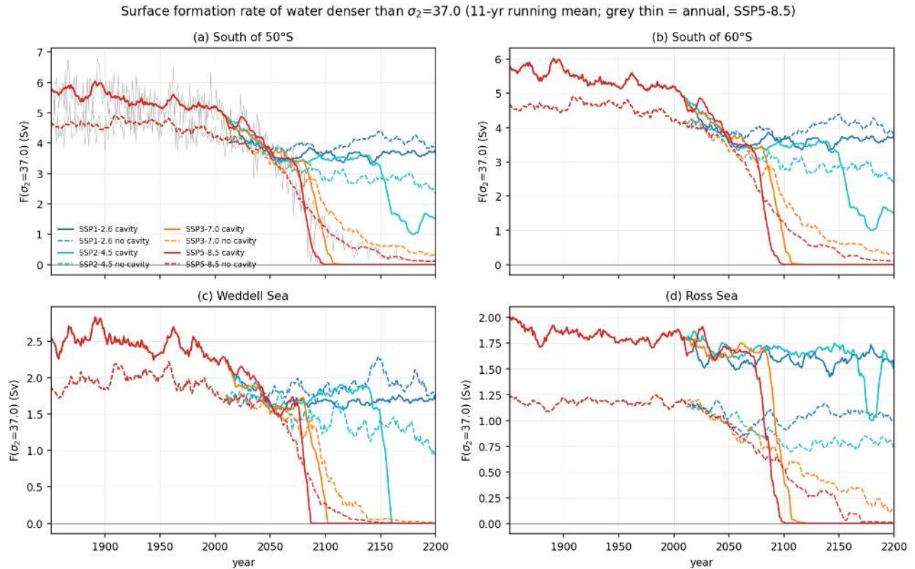
Figure 105: wmt_fig05_ts_dense_formation (wmt). Time series 1851-2200 of the surface formation rate of water denser than \sigma_2=37.0 ( F at 37.0, 11-yr running mean; thin grey shows annual values of the cavity SSP5-8.5 chain) south of 50S (a), south of 60S (b), Weddell Sea (c) and Ross Sea (d) for the four scenarios and both sets. Present-day values are 5.1 (cavity) and 4.3 Sv (no cavity) south of 50S, 2.3 and 1.8 Sv in the Weddell Sea, 1.8 and 1.2 Sv in the Ross Sea. A slow decline from 5.7 Sv in 1851-1880 to 5.1 Sv at present occurs only in the cavity run. Under SSP5-8.5 the formation falls below 25 percent of the present value in 2084 (cavity) and 2103 (no cavity) and is zero (cavity, from about 2090) or 0.1 Sv (no cavity) in 2171-2200. Under SSP3-7.0 it vanishes in the cavity run around 2100 and drops to 0.4 Sv in the no-cavity run. Under SSP2-4.5 the cavity run loses the Weddell formation in 2157 while the no-cavity run keeps 1.2 Sv there. Under SSP1-2.6 formation stabilises at 3.7 (cavity) and 4.0 Sv (no cavity).
