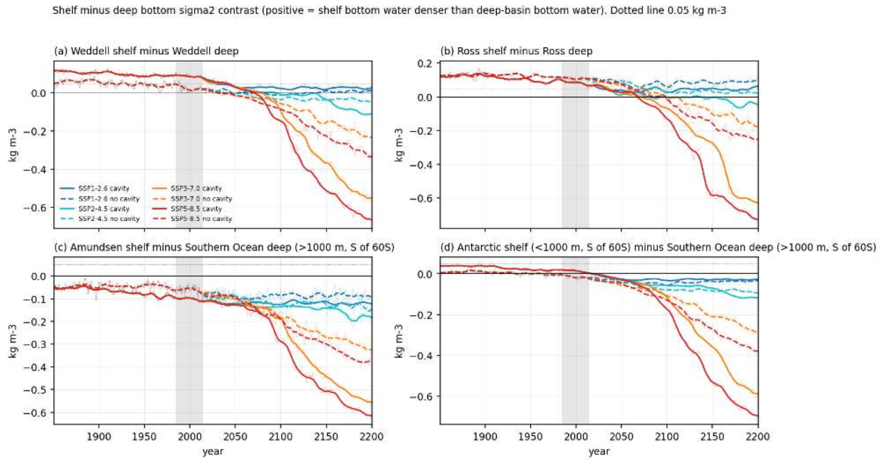
Figure 91: bottom_ts_contrast (bottom). Shelf minus deep bottom sigma2 contrast (kg m -3 ): Weddell shelf minus deep Weddell (a), Ross shelf minus deep Ross (b), Amundsen shelf minus deep Southern Ocean (c) and all Antarctic shelf minus deep Southern Ocean (d), 1851-2200, 11-yr running means over annual values. Positive values mean the shelf bottom water is on average denser than the deep bottom water and can in principle sink. Dotted line 0.05 kg m -3 . The Weddell and Ross contrasts are 0.08 to 0.12 kg m -3 in 1851-1880, have already halved by 2014 in the no-cavity Weddell, and reach zero around 2070 (Weddell cavity run SSP5-8.5 in 2072, Ross in 2068). Under SSP1-2.6 they level off at 0.02 to 0.05 kg m -3 and never vanish. The Amundsen shelf is always lighter than the deep ocean.
