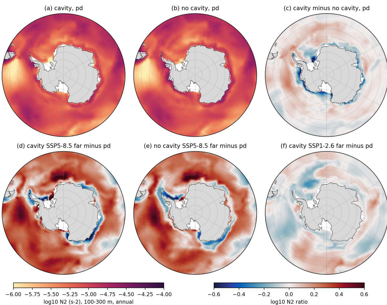
Figure 128: circ_N2_maps (circ). Maps south of 50S of \log_{10} N_2 averaged over 100-300 m (annual), same panel layout as above (cavity nodes excluded). Take-away: at pd the weakest 100-300 m stratification ( N_2 about 5e-6 s-2) is found over the Ross shelf in the cavity run ( 5.1e-6 versus 8.1e-6 in the no-cavity run) and near Maud Rise in the no-cavity run ( 4.7e-6 versus 5.3e-6 ), matching where each set convects. Under SSP5-8.5 N_2 south of 60S increases by 60-70 percent (ssa mean 7.7e-6 to 1.28e-5 cavity, 7.9e-6 to 1.18e-5 no cavity), except on the East Antarctic and Ross shelves where it decreases (blue rings) as the winter halocline erodes.
