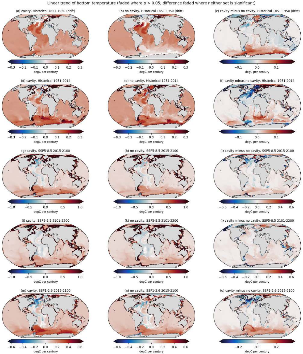
Figure 164: fig01_trend_btemp_global (propagation). Linear trends of bottom temperature (degC per century) on a Robinson projection. Rows are the periods 1851-1950 (historical drift), 1951-2014, SSP5-8.5 2015-2100, SSP5-8.5 2101-2200 and SSP1-2.6 2015-2100. Columns are cavity, no cavity and cavity minus no cavity. Colours are faded where the trend is not significant ( p > 0.05 , two-sided t test on the OLS slope); the difference is faded where neither set is significant. Take-away. The deep ocean warms by 0.08 to 0.09 degC per century almost everywhere already in 1851-1950, which is spin-up drift. The forced signal in 2015-2100 is a Southern Ocean warming of 0.2 to 0.4 degC per century south of 40S (strongest in the Indian sector) and an abyssal cooling of the Atlantic north of 30S of -0.05 to -0.2 degC per century that reverses the drift. The cavity run warms 0.05 degC per century faster in the Southern Ocean than the no-cavity run.
