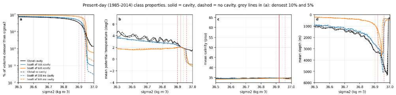
Figure 148: census_class_properties (census). Present-day class properties as a function of sigma2 for the global ocean (black), south of 30S (blue) and south of 60S (orange), cavity solid and no cavity dashed. (a) Percentage of the volume denser than a given sigma2 (log scale, grey lines at 10 and 5 percent). (b) Volume-weighted mean potential temperature, (c) salinity and (d) mean depth of each 0.005 class. The abyssal mode (36.90-36.96) has 1.8-2.0 degC and 34.67-34.69 psu at 3000-4500 m in both runs, i.e. the model AABW class is CDW-like. The cavity run has its densest classes 0.1-0.15 degC colder than the no-cavity run, which is why its mode is 0.01-0.02 kg m -3 denser.
