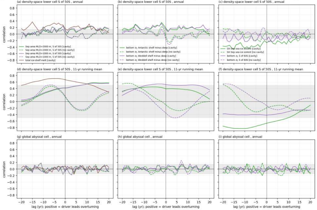
Figure 146: moc_lagcorr_hist (moc). Lagged correlations between detrended historical (1851-2014) driver series and the density-space lower cell south of 50S (a-c annual, d-f 11-yr running means) and the global abyssal cell (g-i annual). Positive lag means the driver leads. Drivers are the September convection area (MLD > 2000 m and > 1000 m), the total ice-shelf melt (cavity only), the shelf minus deep bottom density contrast (all Antarctica and Weddell), the September SH sea-ice extent and the bottom sigma2 south of 60S. Since the lower-cell index is negative, r < 0 means that a larger driver value goes with a stronger cell. On annual scales no driver explains more than 15 percent of the variance in either set. On decadal scales the cavity lower cell co-varies with sea-ice extent ( r = -0.67 at lag 0, more ice with a stronger cell) and with ice-shelf melt ( r = +0.67 , more melt with a weaker cell) but these series have only about 15 degrees of freedom and share the historical trend structure. No driver shows a consistent decadal relation in the no-cavity run.
