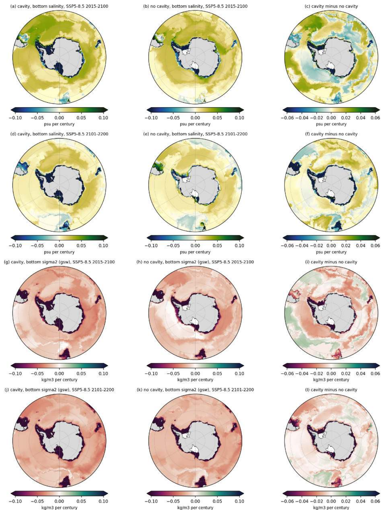
Figure 168: fig05_trend_salt_sig2_south (propagation). South polar view of the bottom salinity (rows 1 and 2) and gsw bottom sigma2 (rows 3 and 4) trends for SSP5-8.5 2015-2100 and 2101-2200, cavity, no cavity and difference. Take-away. The deep Weddell and Ross bottom waters become saltier by 0.02 to 0.04 psu per century and lighter by 0.04 to 0.08 kg/m3 per century. The cavity run shows a stronger coastal salinification in 2015-2100 in the Weddell and Amundsen sectors, consistent with CDW intrusion replacing shelf water, and a weaker one around Dronning Maud Land where PI_CTRL has open ocean and PI_ICEv2 has cavities.
