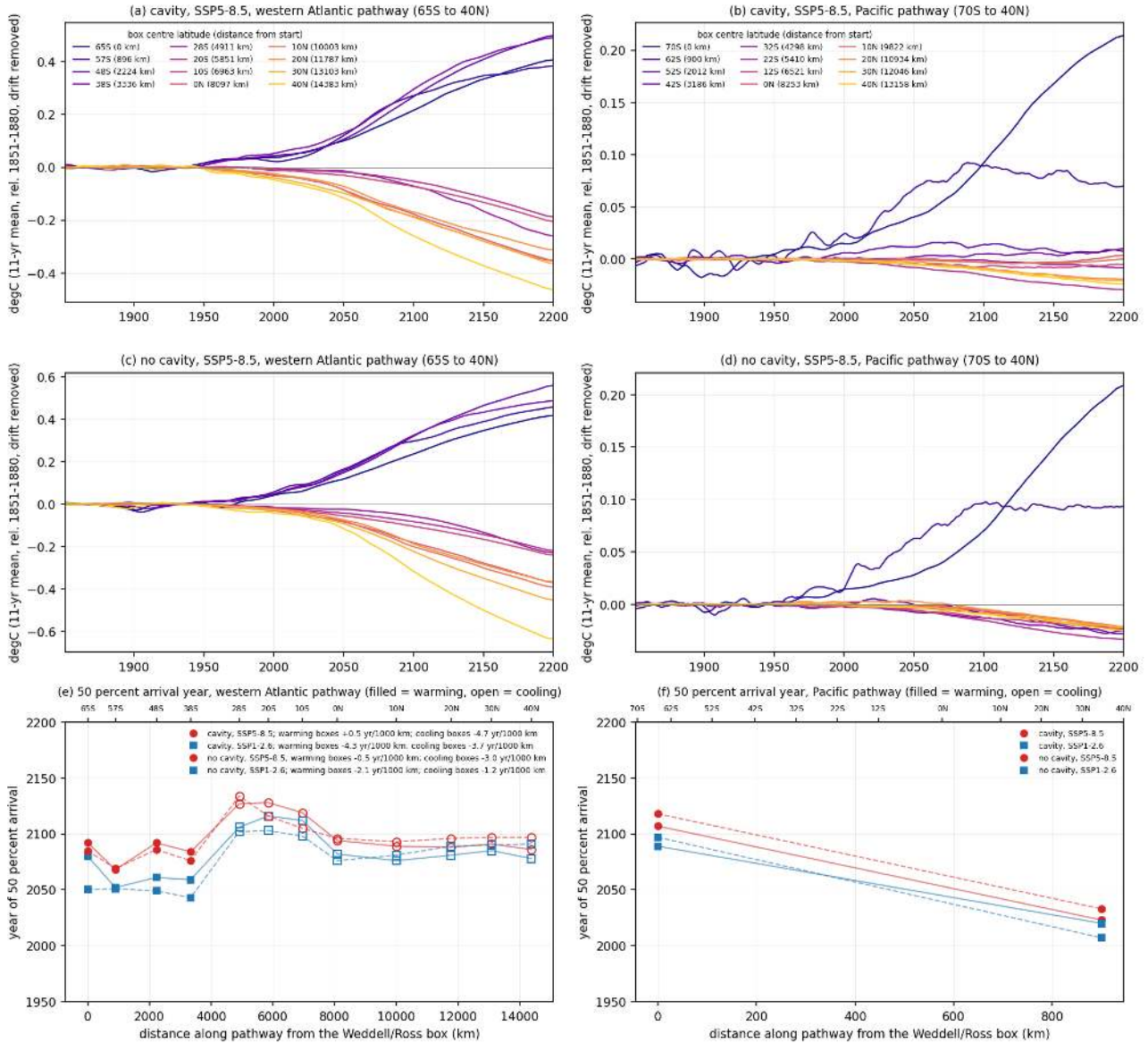
Figure 174: fig11_propagation_lag (propagation). Panels (a) to (d) show the 11-yr running mean drift-corrected bottom temperature anomaly (SSP5-8.5) in 10 deg by 8 deg boxes deeper than 3500 m along the western Atlantic pathway (65S, 30W to 40N, 55W; 12 boxes, 14400 km) and along a Pacific pathway (70S, 178W to 40N, 170W; 12 boxes, 13200 km), colour coded by distance from the first box. Panels (e) and (f) show for each box the year in which the anomaly reaches 50 percent of its 2171-2200 value (boxes with a final anomaly smaller than 0.05 degC are omitted), filled markers for warming and open markers for cooling boxes, SSP5-8.5 in red and SSP1-2.6 in blue, cavity solid and no cavity dashed. The legend gives the least-squares slope of arrival year versus distance in years per 1000 km for warming and for cooling boxes separately. Take-away. Along the Atlantic pathway the four southern boxes (65S to 38S) warm by 0.37 to 0.53 degC by 2200 with 50 percent arrival between 2068 and 2092 and no systematic delay with distance (slope between -4 and +1 yr per 1000 km, i.e. faster than can be resolved, consistent with a basin-wide adjustment rather than an advective front). The eight northern boxes (28S to 40N) cool by 0.17 to 0.6 degC with 50 percent arrival between 2086 and 2134, the cooling arriving first in the north (40N, 2086 to 2097) and last at 20 to 28S (2116 to 2134), so the cooling spreads southward from the North Atlantic at roughly 3 to 5 yr per 1000 km. In the Pacific only the Ross Sea box (70S) and the 62S box change by more than 0.05 degC (0.2 and 0.07 to 0.09 degC); the abyssal Pacific north of 52S changes by less than 0.03 degC by 2200 in both sets. The lag of maximum correlation (stored in stats_propagation.json) is 0 to 6 years within the warming domain and ill defined (100 to 150 years) between the warming and cooling domains.
