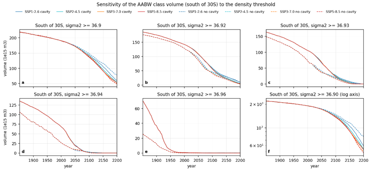
Figure 150: aabw_volume_threshold_sensitivity (census). As the previous figure for the volume south of 30S with thresholds 36.90, 36.92, 36.93, 36.94 and 36.96 (panel f repeats 36.90 on a log axis). The timing of the collapse moves with the threshold because the abyssal mode drifts to lower density at about 0.02 \text{ kg m}^{-3} per century and crosses each threshold in turn, but the statements above (scenario independence, earlier loss without cavities, larger dense volume with cavities) hold for all thresholds. Water above 36.96 disappears before 1950 in both sets.
