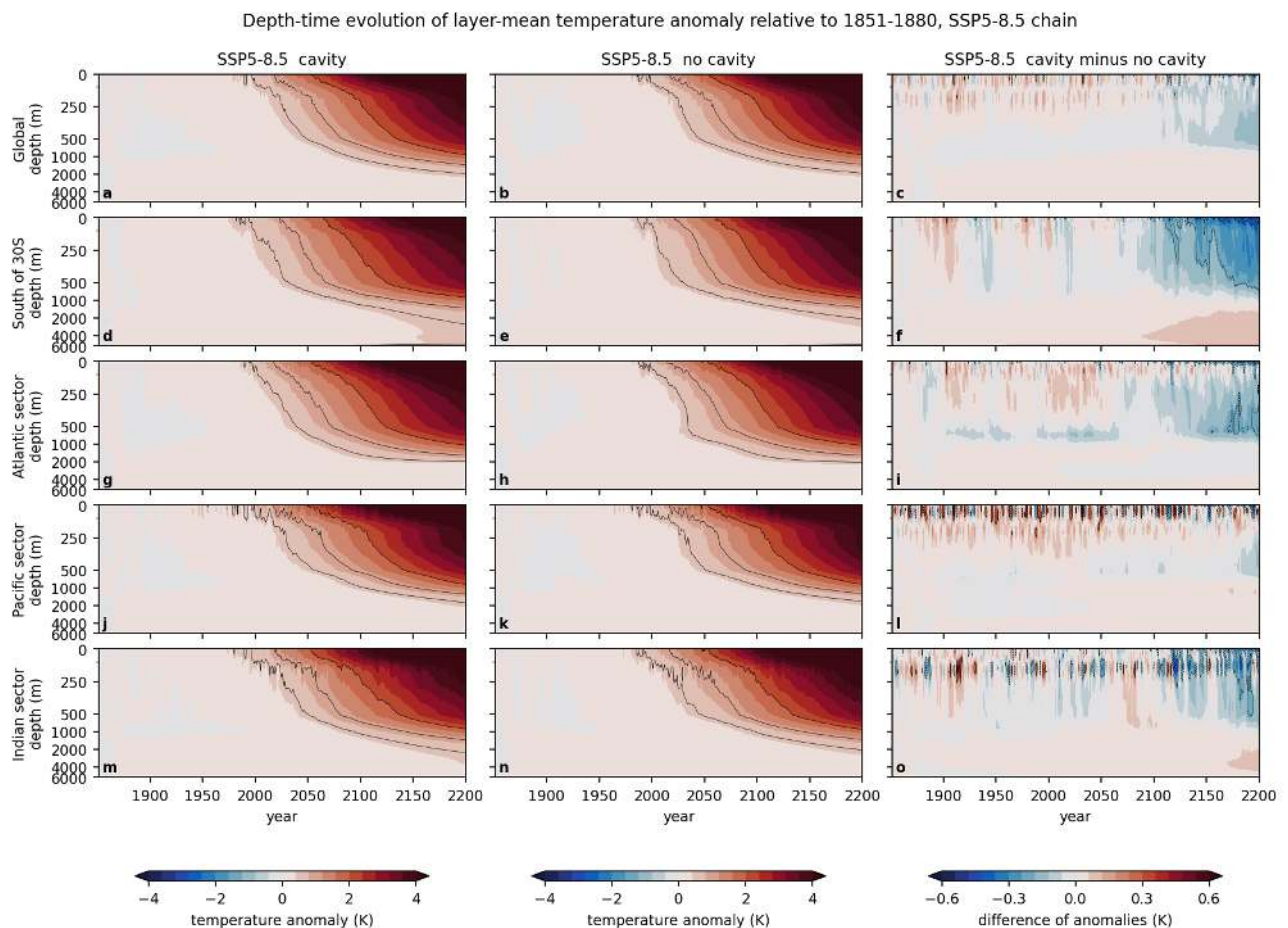
Figure 158: hov_depth_temp_ssp585 (census). Depth-time Hovmoeller of the layer-mean temperature anomaly relative to 1851-1880 for the SSP5-8.5 chain, global, south of 30S, Atlantic, Pacific and Indian sectors (rows), cavity (left), no cavity (middle) and cavity minus no cavity (right, note the smaller colour range). The depth axis is stretched above 500 m. Warming of more than 0.5 K reaches 1000 m globally by 2100 and 2000 m by 2200, the abyss warms by 0.1-0.3 K through drift. The cavity run warms less in the upper 500 m south of 30S after 2100 (by up to 0.6 K, the sea-ice and surface feedback discussed by the atmos theme) but slightly more below 2000 m (0.05-0.1 K).
