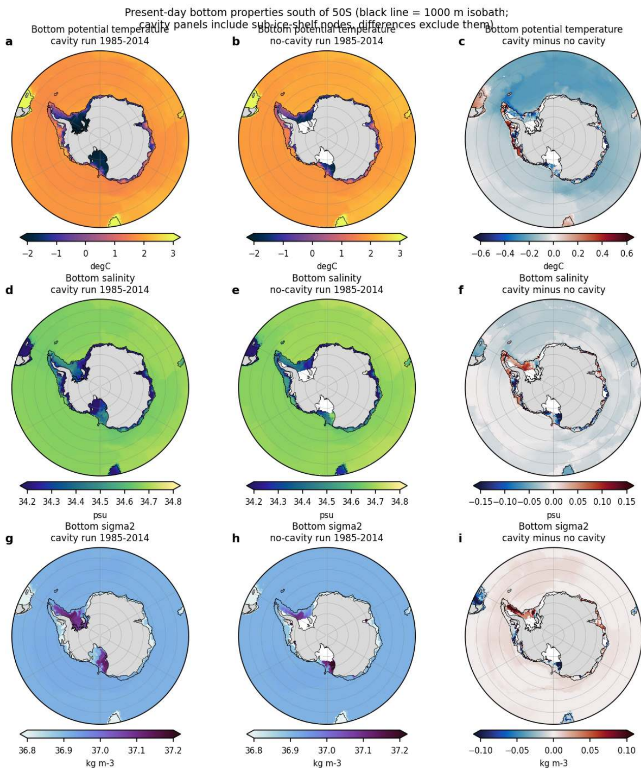
Figure 84: bottom_pd_maps (bottom). Present-day (1985-2014) bottom potential temperature (a-c), salinity (d-f) and sigma2 (g-i) south of 50S on a 0.25 degree grid. Left column cavity run including the sub-ice-shelf nodes, middle column no-cavity run, right column cavity minus no cavity on the common open-ocean grid. Black line is the 1000 m isobath. Units degC, psu, kg m-3. The abyss is 1.7 to 2.0 degC and 36.9 kg m-3 in both runs, so there is no cold AABW layer. Cold (below -1.5 degC) and dense (above 37.0 kg m-3) bottom water exists only on the Weddell and Ross shelves and under the Filchner-Ronne and Ross ice shelves. The cavity run is 0.1 to 0.3 degC cooler over the whole deep Southern Ocean, and its western Weddell shelf is 0.05 to 0.1 psu saltier and 0.05 to 0.1 kg m-3 denser, whereas its Ross shelf is fresher and lighter by a similar amount.
