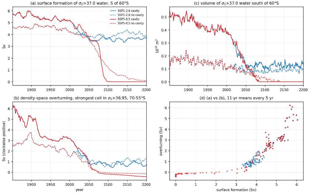
Figure 108: wmt_fig08_consistency_moc_census (wmt). Consistency of the surface formation with the interior. (a) surface formation of \sigma_2 above 37.0 water south of 60S, (b) strength of the densest overturning cell in density space (minimum of the global density-space stream function for \sigma_2 above 36.95 between 70S and 55S, sign reversed so that the clockwise AABW-type cell is positive), (c) volume of \sigma_2 above 37.0 water south of 60S from the census, (d) scatter of (a) against (b). SSP1-2.6 and SSP5-8.5 shown for both sets. The present-day dense cell is 3.1 Sv (cavity) and 1.8 Sv (no cavity), far smaller than the 5.1 and 4.3 Sv surface formation, and the dense volume is only 0.38 and 0.12 times 10^{15} \text{ m}^3 (0.5 and 0.2 percent of the volume south of 60S), so the residence time of surface-formed dense water is 1 to 2 years. Most of the surface densification is eroded by mixing before it reaches the deep ocean. The 11-yr smoothed surface formation and dense cell are correlated at 0.86 to 0.96 along the scenario chains. Under SSP5-8.5 the dense cell and the dense volume vanish in 2071-2100 in both sets.
