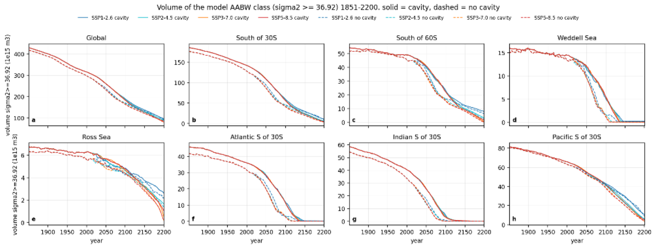
Figure 149: aabw_volume_timeseries (census). Volume of the AABW class ( \sigma_2 \geq 36.92 ) 1851-2200 for the global ocean, south of 30S, south of 60S, Weddell Sea, Ross Sea and the three sectors south of 30S, all four scenario chains and both sets. Present-day volumes are 315 (cavity) and 297 (no cavity) \times 10^{15} \text{ m}^3 globally and 142 and 129 \times 10^{15} \text{ m}^3 south of 30S. The class shrinks by 25 (cavity) and 27 (no cavity) percent already between early and pd, and by 49 (cavity) and 58-61 (no cavity) percent between pd and end south of 30S. The decline is almost identical in all four scenarios (far minus pd south of 30S is -89 to -93 percent cavity, -87 to -94 percent no cavity), so it is a drift of the abyss, not a scenario response. The no-cavity class empties 10-25 years earlier in the Atlantic and Indian sectors and in the Weddell Sea, the Pacific sector and the Ross Sea keep dense water longest.
