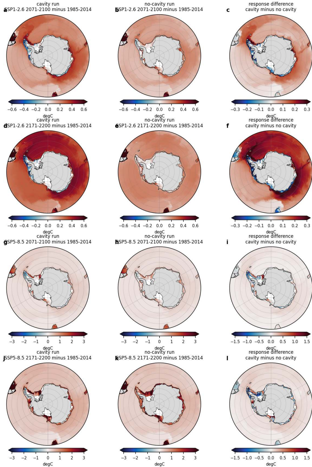
Figure 85: bottom_resp_T (bottom). Change of bottom potential temperature (degC) relative to 1985-2014 for SSP1-2.6 (rows 1 and 2) and SSP5-8.5 (rows 3 and 4) at 2071-2100 and 2171-2200. Left cavity run, middle no-cavity run, right the difference of the two responses (cavity response minus no-cavity response, colour range halved). Cavity nodes excluded. Colour range 0.6 degC for SSP1-2.6 and 3 degC for SSP5-8.5. In SSP1-2.6 the deep Southern Ocean bottom warms 0.2 to 0.4 degC, twice as much in the cavity run because of a persisting spin-up drift of its deep water, while the Weddell shelf stays near its present temperature. In SSP5-8.5 the shelves warm by 1.5 to 2.5 degC by 2171-2200 and the warming is largest where the shelf water was coldest.
