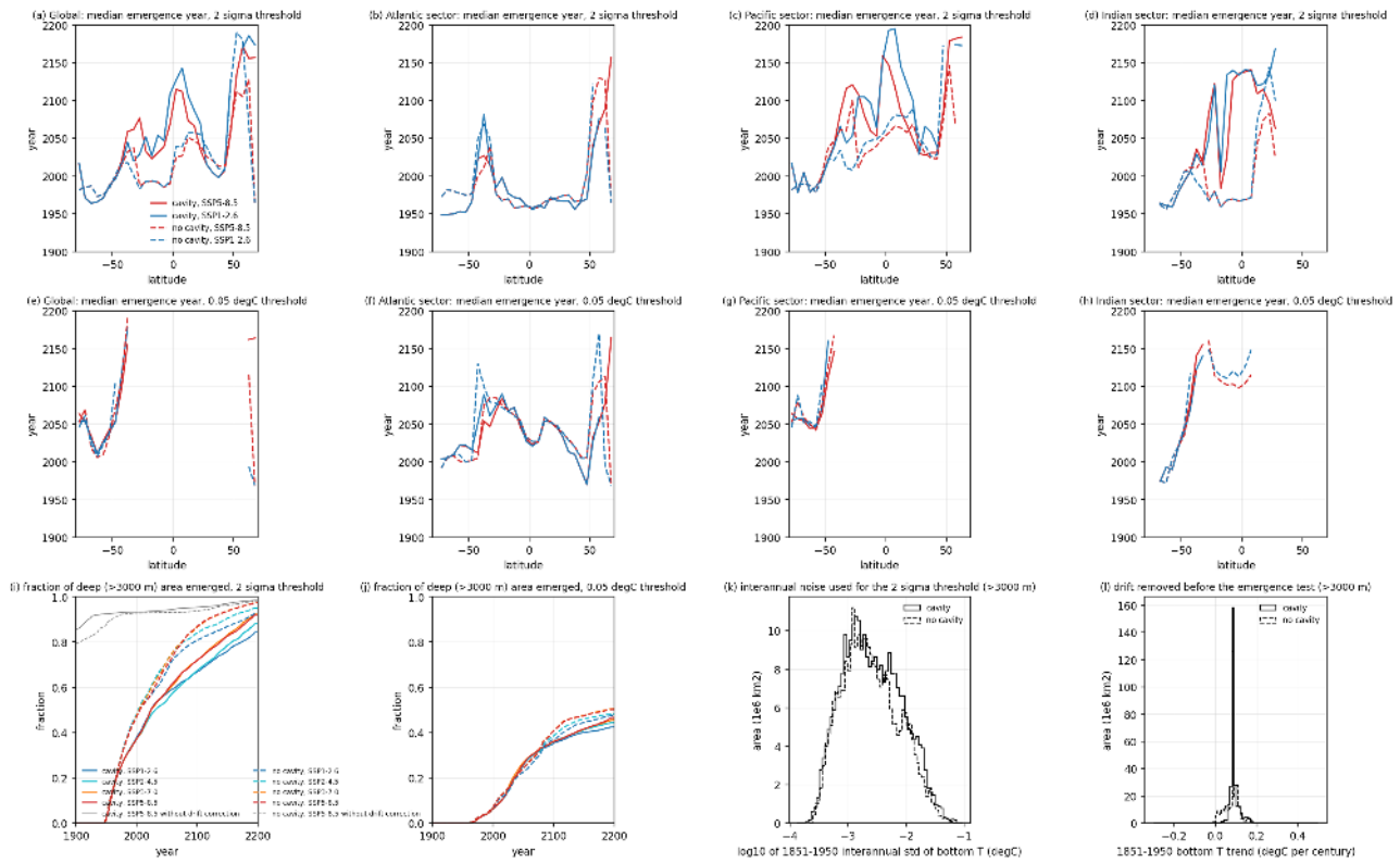
Figure 172: fig09_toe_latitude_summary (propagation). Panels (a) to (d) give the area-weighted median emergence year of bottom temperature (2 sigma threshold) per 5 deg latitude band for nodes deeper than 3000 m, globally and per sector, for SSP5-8.5 (red) and SSP1-2.6 (blue), cavity (solid) and no cavity (dashed). Panels (e) to (h) repeat this for the 0.05 degC threshold. Panel (i) shows the fraction of deep (>3000 m) sea floor area emerged as a function of time for all four scenarios and both sets with the 2 sigma threshold, plus the SSP5-8.5 result without drift correction in grey. Panel (j) is the same for the 0.05 degC threshold. Panels (k) and (l) are area-weighted histograms of the interannual noise and of the removed 1851-1950 drift for the deep nodes. Take-away. Without drift correction 80 to 85 percent of the deep sea floor has "emerged" by 1900, which shows that the raw emergence is drift, not forcing. With the 0.05 degC threshold the emerged fraction is 10 percent in 2014, 36 to 41 percent in 2100 and 42 to 50 percent in 2200, with little dependence on scenario (the emerged area in SSP1-2.6 is only 3 to 5 percent smaller than in SSP5-8.5). Median emergence (0.05 degC) is 2005 to 2030 at 55 to 70S and 2045 to 2085 in the Atlantic between 30S and 40N.
