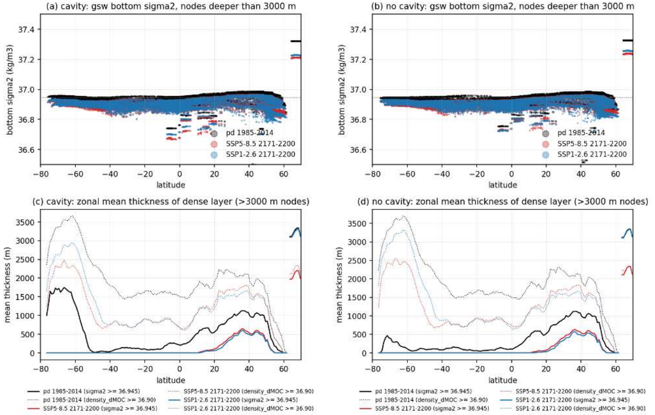
Figure 177: fig13_bottom_sigma2_latitude (propagation). Panels (a) and (b) give the gsw bottom sigma2 of a random subset of nodes deeper than 3000 m versus latitude for pd (black), SSP5-8.5 2171-2200 (red) and SSP1-2.6 2171-2200 (blue), cavity and no cavity; the dotted line is the 36.945 threshold. Panels (c) and (d) give the zonal mean thickness of the dense layer for both definitions (solid gsw sigma2 \geq 36.945 , dotted density_dMOC \geq 36.90 as used by the census theme). Take-away. The abyss has a remarkably uniform bottom sigma2 of 36.94 to 36.98 at present day with the densest values in the North Pacific and North Atlantic (36.97 to 36.98) and the lightest in the deep Southern Ocean (36.94 to 36.95); there is no dense southern end member. By 2200 bottom sigma2 drops to 36.85 to 36.92 everywhere. The density_dMOC layer definition gives thicknesses two to three times larger and does not reproduce the cavity minus no-cavity contrast, because density_dMOC is nearly constant (36.91 to 36.92) below 700 m.
