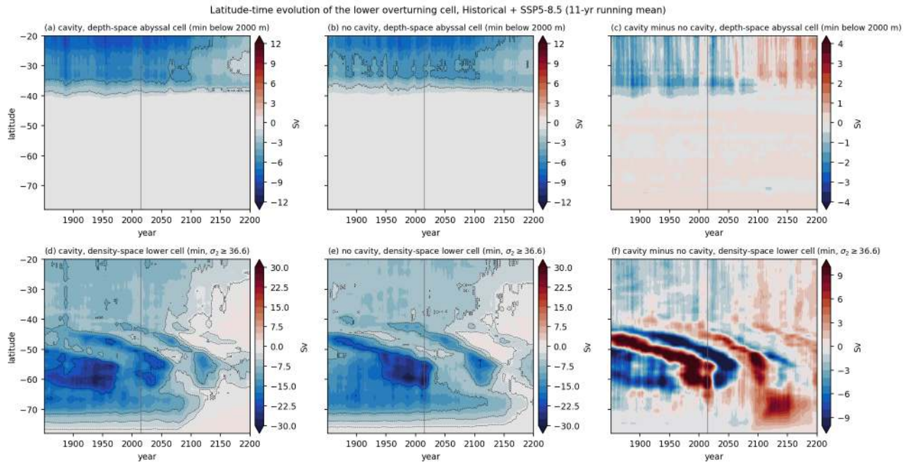
Figure 142: moc_hovmoeller_ssp585 (moc). Latitude-time evolution (11-yr running means) of the lower overturning cell for the historical plus SSP5-8.5 chain. Top row, depth-space abyssal cell strength per latitude (minimum below 2000 m); bottom row, density-space lower cell per latitude (minimum over \sigma_2 \geq 36.6 ); cavity (a, d), no cavity (b, e) and difference (c, f). In depth space the abyssal cell exists only north of 38S (south of that the Eulerian Deacon cell dominates). In density space the cell is strongest at 55S-65S. Diagonal stripes in the density-space panels come from the slow drift of the lower-cell core to lighter classes with the coarse class resolution, so the difference panel (f) should be read with care. The density-space cell south of 55S collapses within two decades after 2020 in the no-cavity run (from -30 to -15 Sv) and more gradually in the cavity run, and both sets reach 5-8 Sv by 2170. The depth-space cell north of 38S weakens after 2100.
