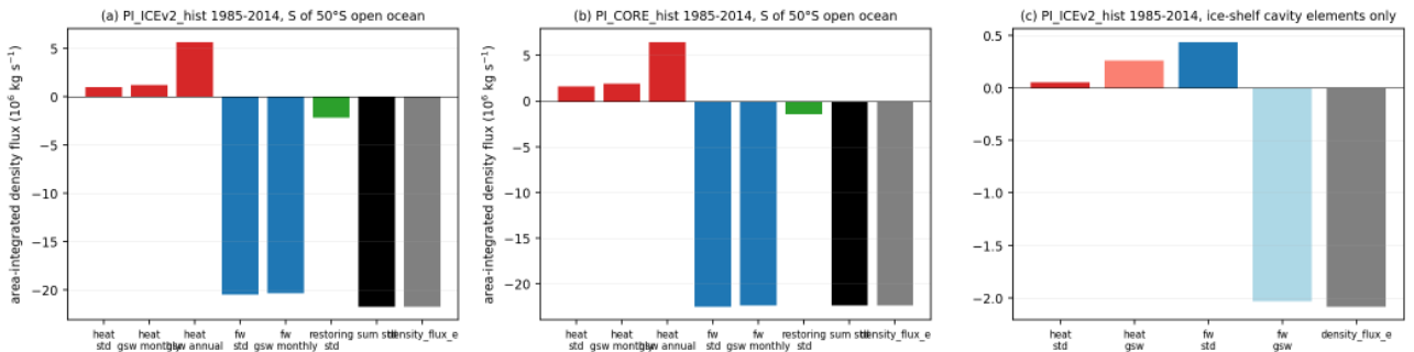
Figure 104: wmt_fig04_validation_density_flux (wmt). Validation of the diagnostic for 1985-2014. Panels a and b show the area-integrated surface density flux south of 50S (open ocean) for the two historical runs: the class-summed heat and freshwater terms from the FESOM diagnostic (std), independent estimates from the monthly fh, fw, SST and SSS climatologies with gsw alpha and beta (gsw monthly), the same estimate with annual means (gsw annual), the restoring term, the sum of the three std terms and the separately stored density_flux_e. Panel c shows the cavity elements of the cavity run only. The freshwater term agrees to 1 percent (-20.5 versus -20.4 and -22.5 versus -22.4 million kg/s), the heat term to 25 percent when the seasonal cycle is resolved (0.9 versus 1.2 and 1.6 versus 1.9 million kg/s) but is six times too large when annual means are used. The sum of the three std terms equals density_flux_e exactly (-21.7 million kg/s). Under the ice shelves the class-binned freshwater term has the wrong sign (+0.4 instead of -2.0 million kg/s), while density_flux_e (-2.1) agrees with the melt water input of 2360 Gt/yr. This is why cavity elements are excluded from F .
