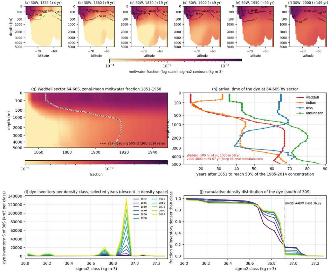
Figure 83: mw_fig18_descent (meltwater). Downward spreading of ice-shelf meltwater after the dye release in 1851 (cavity run PI_ICEv2_hist). (a-f) Meridional sections of the meltwater fraction along 30W (log scale) 4, 9, 19, 49, 99 and 149 years after the release, with model sigma2 contours. (g) Depth-time diagram of the zonal-mean fraction in the Weddell sector at 64-66S for 1851-1950; the dashed line marks, for each depth, the year in which the 11-yr smoothed concentration first reaches half of its 1985-2014 value. (h) The same arrival time versus depth for the Weddell, Indian, Ross and Amundsen sectors. (i) Dye inventory south of 30S per 0.05 kg m -3 sigma2 class for selected years and (j) the fraction of the inventory denser than each class. Take-away. The dye leaves the shelf in the upper 100 to 500 m and reaches the deep slope at 60 to 65S within two decades (panel c), but the abyss is not filled by a plume descending step by step. In the Weddell sector 500 m is reached after 34 years, 1000 m after 59 years and the whole 2000 to 4000 m column within 63 to 67 years, so below 1000 m the arrival is nearly simultaneous. The other sectors reach the abyss later (Ross 45 to 73 years, Amundsen 73 to 87 years). In density space the dye is transferred from the light shelf and surface classes into the single abyssal mode near sigma2 36.9 within 50 years, the fraction denser than 36.92 rising from 27 percent in 1852 to 60 percent by 1900 and staying there. The descent is therefore a diapycnal transfer into the homogeneous deep water mass within a few decades rather than a dense-plume pathway.
