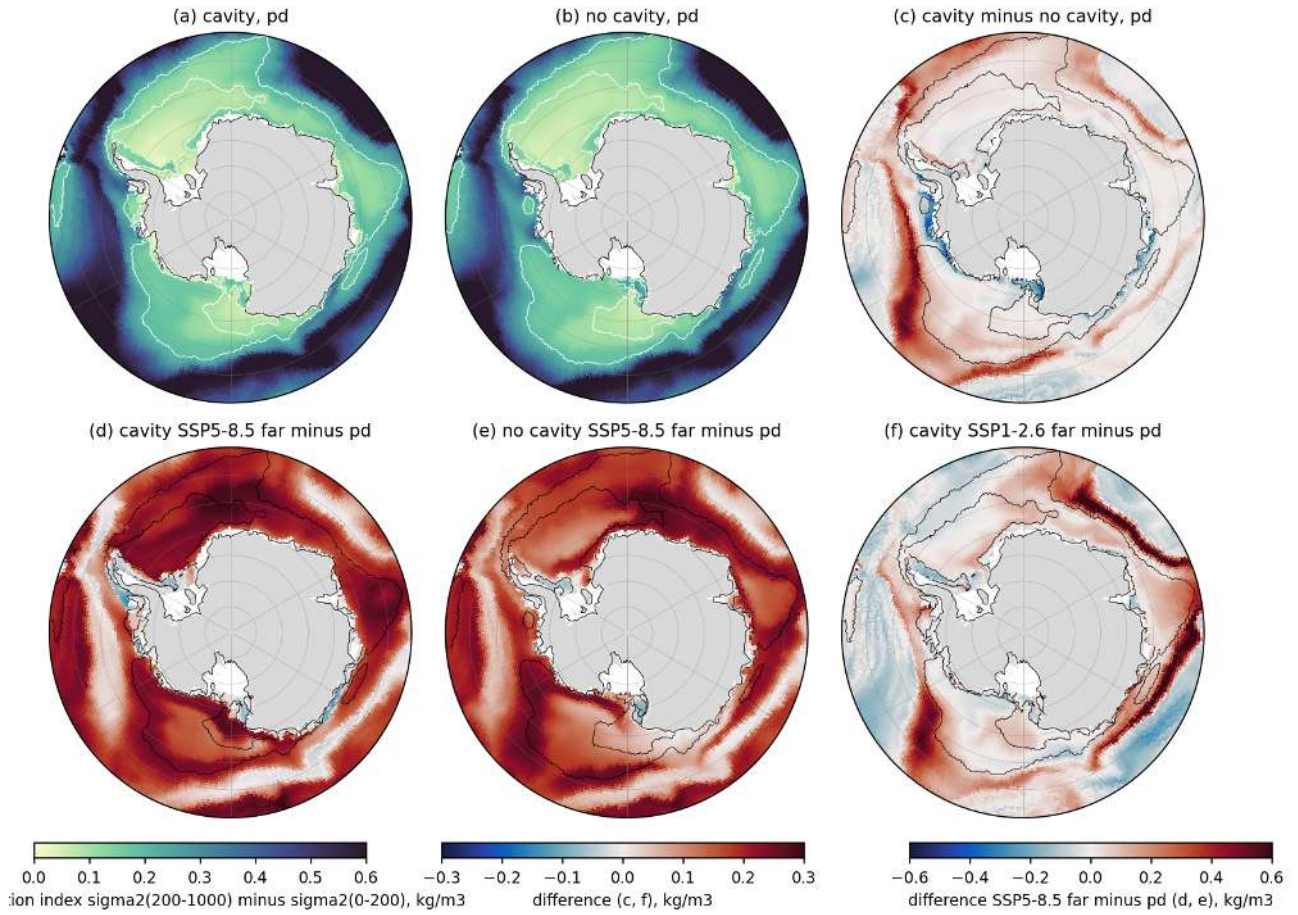
Figure 129: circ_strat_maps (circ). Upper-ocean stratification index \sigma_2(200-1000 \text{ m}) minus \sigma_2(0-200 \text{ m}) ( \text{kg/m}^3 ) south of 55°S, cavity nodes excluded. (a) cavity pd, (b) no cavity pd, (c) cavity minus no cavity, (d, e) SSP5-8.5 far minus pd for cavity and no cavity (scale \pm 0.6 ), (f) cavity SSP1-2.6 far minus pd. White/black contours 0.1 and 0.2 \text{kg/m}^3 of the reference. Take-away: the weakly stratified ( < 0.15 \text{ kg/m}^3 ) deep Weddell and Ross gyre interiors are the convection-prone areas; at Maud Rise the index is 0.119 (cavity) versus 0.107 \text{kg/m}^3 (no cavity), consistent with the no-cavity run convecting every winter and the cavity run only intermittently; on the Ross shelf it is 0.10 versus 0.15. Under SSP5-8.5 the index rises to 0.55 (cavity) and 0.51 \text{kg/m}^3 (no cavity) south of 60°S, a fourfold increase that shuts down open-ocean convection; under SSP1-2.6 it rises only by 0.03-0.04 \text{kg/m}^3 .
