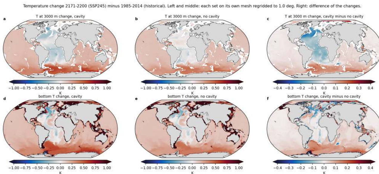
Figure 162: map_deepT_change_ssp245 (census). As the previous figure for SSP2-4.5. The pattern is the same with about half the amplitude at the bottom (global 0.33 and 0.31 K, south of 30S 0.35 and 0.29 K) and nearly the same amplitude at 3000 m (0.16 and 0.15 K globally), which confirms that the 3000 m change is largely drift.
