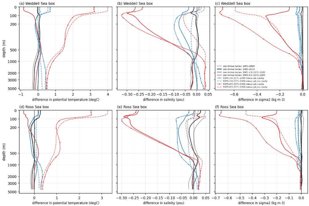
Figure 93: bottom_profiles_diff (bottom). Profile differences for the same boxes: cavity minus no cavity (plain lines for 1851-1880 grey, 1985-2014 black, SSP1-2.6 2171-2200 blue, SSP5-8.5 2171-2200 red) and 2171-2200 minus 1985-2014 (dotted markers cavity, dashed no cavity; blue SSP1-2.6, red SSP5-8.5). The cavity run is 0.2 to 0.3 degC cooler than the no-cavity run below 1000 m in the Weddell box and 0.15 degC cooler in the Ross box in 1851-1880, and the difference shrinks to 0.1 to 0.2 degC by 1985-2014 and to zero by 2200 under SSP1-2.6, which is the signature of the cavity run's deep drift. Density differences between the two runs are below 0.01 kg m -3 below 500 m at all times.
