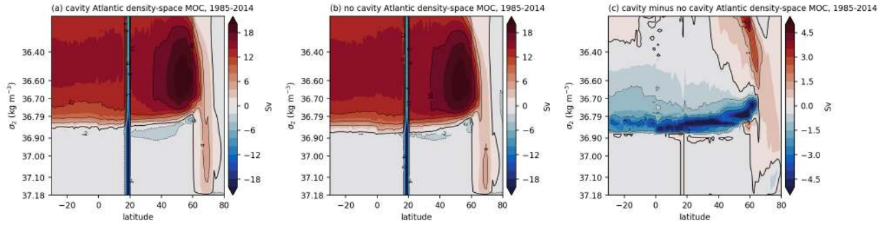
Figure 135: moc_dens_atl_pd (moc). As moc_dens_global_pd for the Atlantic sector north of 30S. The density-space AMOC at 26N is 14.7 Sv (cavity) and 15.1 Sv (no cavity) in classes lighter than \sigma_2 36.8. The dense return flow below the NADW class is under 2 Sv. Differences between the two sets are below 1 Sv except at the class boundaries.
