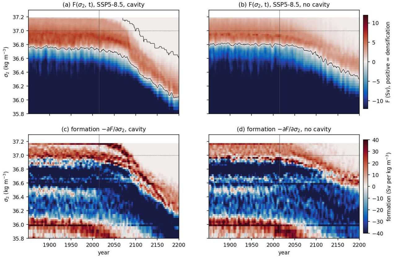
Figure 109: wmt_fig09_hovmoeller_ssp585 (wmt). Density-time Hovmoeller of the total transformation rate F(\sigma_2, t) south of 50S for the SSP5-8.5 chain (5-yr running mean), cavity run (a) and no-cavity run (b), and the corresponding formation rate minus dF/d\sigma_2 (c, d). Red is densification, blue is lightening, the black contour marks F = 0 , the dotted line \sigma_2 37.0 and the vertical line the 2014/2015 transition. The zero crossing, which separates the lightening of subpolar water from the densification of coastal water, moves from \sigma_2 36.7 at present to 36.0 by 2200 in both sets, and the densest transformed class moves from 37.18 to about 36.6. The shift starts around 2040 and is similar in both sets, the cavity run being slightly faster in the densest classes after 2080.
