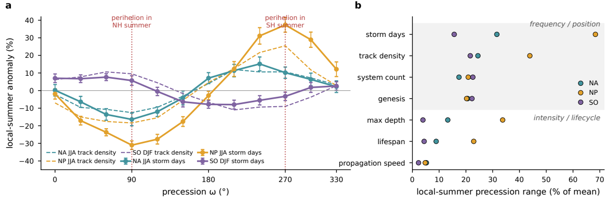
FIG. 7. (a) Local-summer storm activity across the precession cycle, shown as the percent anomaly of basin-mean storm days from the phase mean (solid, with 95% confidence intervals of the 30-year mean) and of track density (dashed), for the North Atlantic and the North Pacific in JJA and for the Southern Ocean in DJF; dotted vertical lines mark the phases with perihelion in NH and SH summer. (b) Local-summer across-phase range for frequency and position metrics and for intensity and lifecycle metrics in each basin.
