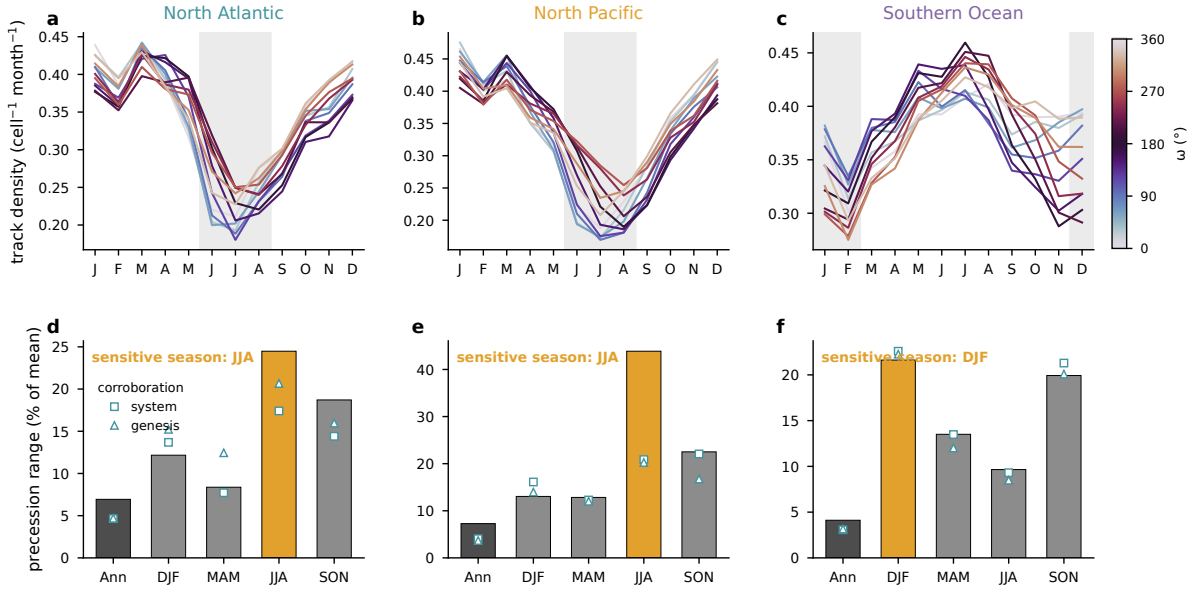
Figure 4: Seasonal concentration of the precessional storm response, from the Lagrangian tracks. (a)–(c) Basin-mean track density (cell -1 month -1 ) by calendar month for the North Atlantic, the North Pacific, and the Southern Ocean, one line per phase colored by \omega , with local summer shaded. (d)–(f) Across-phase range of track density (maximum minus minimum, percent of the phase mean) for the annual mean and the four seasons, with the local-summer bar highlighted; open symbols give the corresponding ranges of system and genesis densities.
