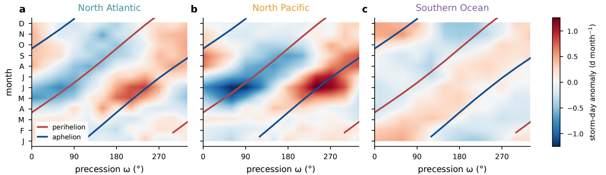
FIG. A7. Basin-mean storm-day anomaly (d month -1 ) relative to the phase mean as a function of calendar month and precession phase for (a) the North Atlantic, (b) the North Pacific, and (c) the Southern Ocean, with the perihelion (red) and aphelion (blue) calendar months of each phase overlaid.
