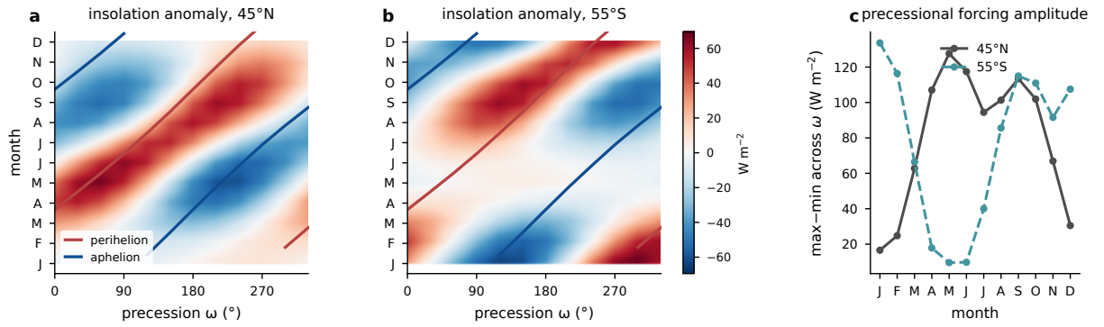
FIG. A3. Precessional insolation forcing from orbital geometry with eccentricity 0.058 and obliquity 24.5^\circ . (a) Monthly insolation anomaly relative to the phase mean at 45^\circ\text{N} as a function of calendar month and precession phase \omega , with the perihelion (red) and aphelion (blue) calendar months of each phase overlaid. (b) As in (a), but for 55^\circ\text{S} . (c) Precessional forcing amplitude by calendar month, the maximum minus minimum monthly insolation across the twelve phases, at both latitudes. Units: \text{W m}^{-2} .
