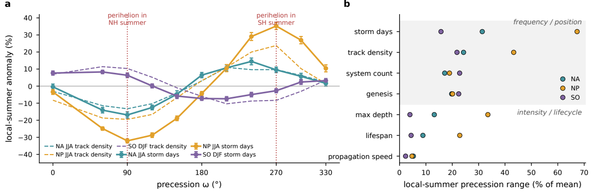
FIG. A10. (a) Local-summer storm activity across the precession cycle, shown as the percent anomaly of basin-mean storm days from the phase mean (solid, with interannual standard errors) and of track density (dashed), for the North Atlantic and the North Pacific in JJA and for the Southern Ocean in DJF; dotted vertical lines mark the phases with perihelion in NH and SH summer. (b) Local-summer across-phase range for frequency and position metrics and for intensity and lifecycle metrics in each basin.
