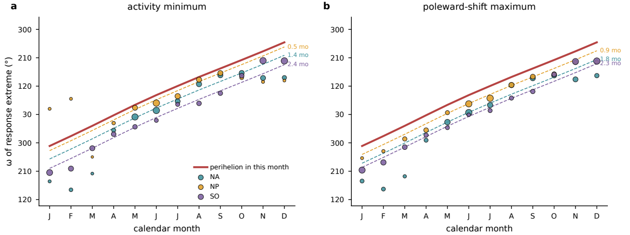
FIG. A11. Phase locking of the storm response to the perihelion calendar. For each calendar month and basin, the phase of the first harmonic across the eleven precession phases of (a) basin-mean storm days, shown as the \omega of the activity minimum, and (b) the storm-day-weighted track latitude, shown as the \omega of the poleward maximum. Marker size scales with the harmonic amplitude. The red line gives the \omega that places perihelion in that calendar month, and dashed lines repeat it delayed by each basin's median lag over the amplitude-strong months (annotated in months).
