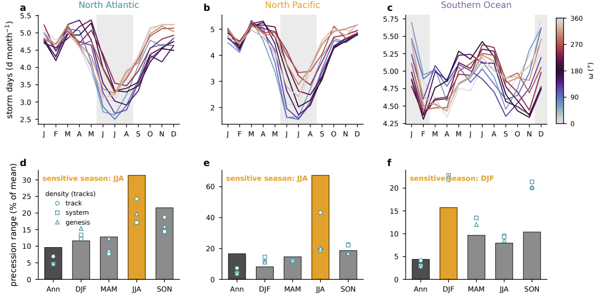
FIG. A6. Seasonal concentration of the precessional storm response. (a)–(c) Basin-mean storm days (d month -1 ) by calendar month for the North Atlantic, the North Pacific, and the Southern Ocean, one line per phase colored by \omega , with local summer shaded. (d)–(f) Across-phase range of storm days (maximum minus minimum, percent of the phase mean) for the annual mean and the four seasons, with the local-summer bar highlighted; open symbols give the corresponding ranges of track, system, and genesis densities from the Lagrangian tracks.
