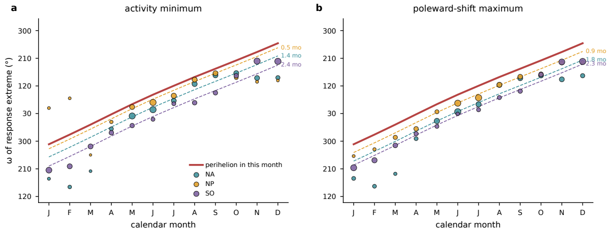
FIG. 9. Phase locking of the storm response to the perihelion calendar. For each calendar month and basin, the phase of the first harmonic across the eleven precession phases of (a) basin-mean storm days, shown as the \omega of the activity minimum, and (b) the storm-day-weighted track latitude, shown as the \omega of the poleward maximum. Marker size scales with the harmonic amplitude. The red line gives the \omega that places perihelion in that calendar month, and dashed lines repeat it delayed by each basin's median lag over the amplitude-strong months (annotated in months).
