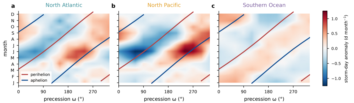
FIG. 5. Basin-mean storm-day anomaly ( \text{d month}^{-1} ) relative to the phase mean as a function of calendar month and precession phase for (a) the North Atlantic, (b) the North Pacific, and (c) the Southern Ocean, with the perihelion (red) and aphelion (blue) calendar months of each phase overlaid.
