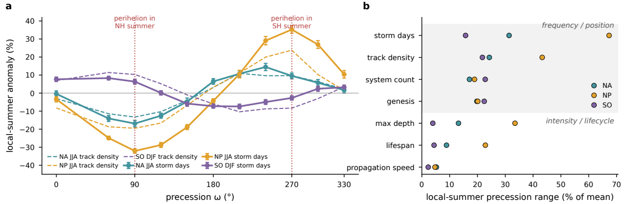
FIG. 8. (a) Local-summer storm activity across the precession cycle, shown as the percent anomaly of basin-mean storm days from the phase mean (solid, with interannual standard errors) and of track density (dashed), for the North Atlantic and the North Pacific in JJA and for the Southern Ocean in DJF; dotted vertical lines mark the phases with perihelion in NH and SH summer. (b) Local-summer across-phase range for frequency and position metrics and for intensity and lifecycle metrics in each basin.
