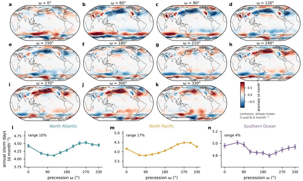
FIG. 3. Annual-mean storm days across the precession cycle. (a)–(k) Annual storm-day anomaly of each phase relative to the eleven-phase mean (shading), with the phase-mean climatology outlined at 5 and 8 \text{d month}^{-1} (contours). (l)–(n) Basin-mean annual storm days against \omega with interannual standard errors; the across-phase range as a percentage of the phase mean is annotated in each panel.
