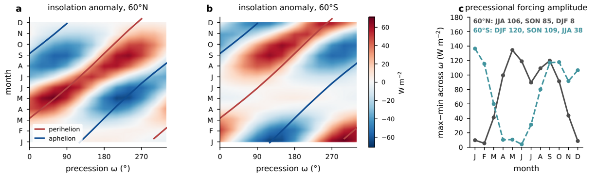
FIG. 1. Precessional insolation forcing from orbital geometry with eccentricity 0.058 and obliquity 24.5^\circ . (a) Monthly insolation anomaly relative to the phase mean at 60^\circ\text{N} as a function of calendar month and precession phase \omega , with the perihelion (red) and aphelion (blue) calendar months of each phase overlaid. (b) As in (a), but for 60^\circ\text{S} . (c) Precessional forcing amplitude by calendar month, the maximum minus minimum monthly insolation across the twelve phases, at both latitudes. Units: \text{W m}^{-2} .
