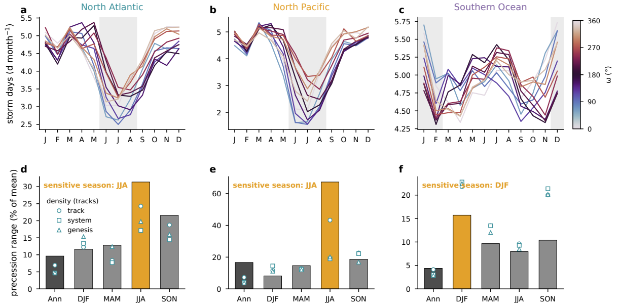
FIG. 4. Seasonal concentration of the precessional storm response. (a)–(c) Basin-mean storm days ( \text{d month}^{-1} ) by calendar month for the North Atlantic, the North Pacific, and the Southern Ocean, one line per phase colored by \omega , with local summer shaded. (d)–(f) Across-phase range of storm days (maximum minus minimum, percent of the phase mean) for the annual mean and the four seasons, with the local-summer bar highlighted; open symbols give the corresponding ranges of track, system, and genesis densities from the Lagrangian tracks.
