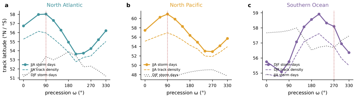
Figure A2: Storm-track latitude across the precession cycle, the storm-day-weighted mean latitude over each basin sector, for (a) the North Atlantic, (b) the North Pacific, and (c) the Southern Ocean. Solid lines with markers give the local-summer track latitude, thin dashed lines the corresponding track-density-weighted latitude, and dotted gray lines the local-winter track latitude. Vertical dotted lines mark the phase with perihelion in the local summer of each basin.
