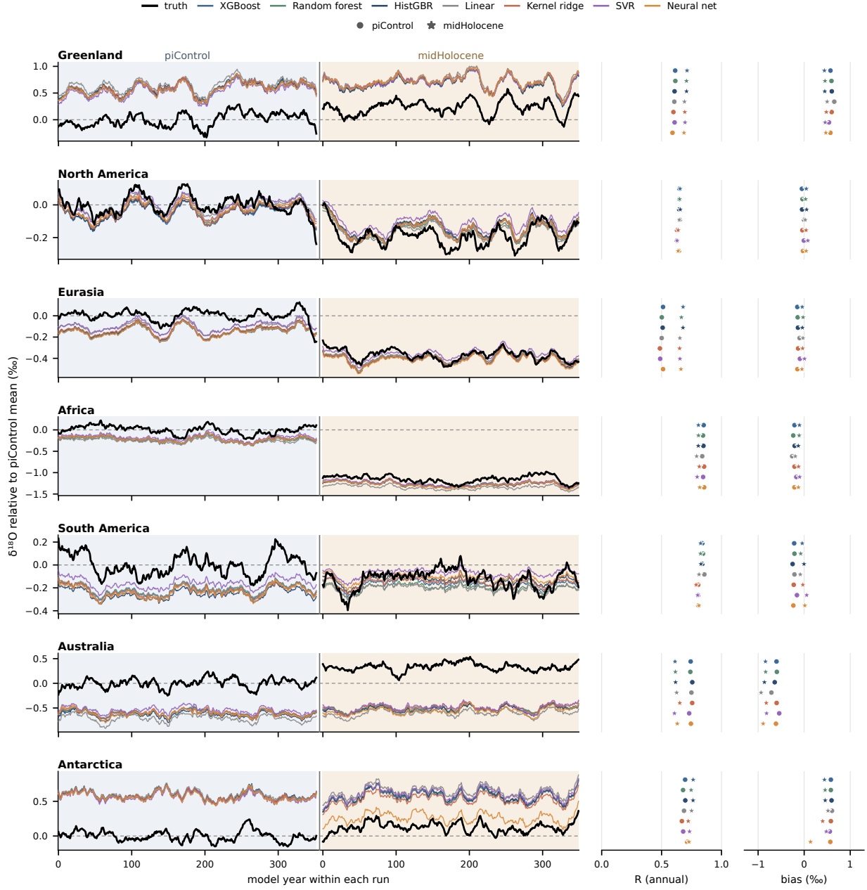
Figure 3: MPI-ESM-wiso piControl and mid-Holocene drawn as one continuous series per region, with \delta^{18}\text{O} expressed relative to the piControl mean state so that the piControl segment sits near zero by construction and the mid-Holocene segment is a directly readable departure. Shaded blocks separate the two states, which are independent simulations rather than one time axis, and the model year restarts at zero for the mid-Holocene block. Black is the simulation and the coloured lines are the seven learners. The strips on the right give the per-region correlation and mean bias, with circles for the piControl and stars for the mid-Holocene.
