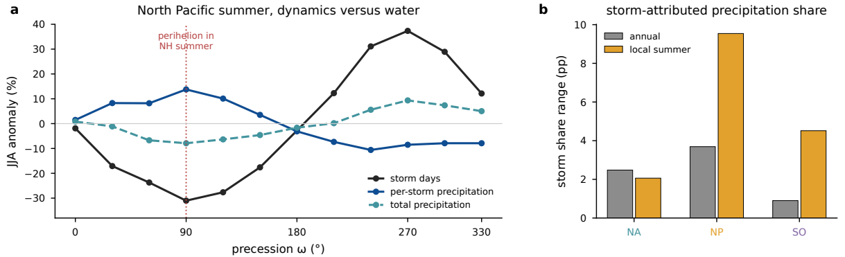
FIG. 11. Storm-attributed precipitation across the precession cycle. (a) North Pacific JJA percent anomalies from the phase mean of basin-mean storm days, per-storm precipitation, and total precipitation; the dotted line marks the phase with perihelion in NH summer. (b) Across-phase range of the storm-attributed share of precipitation, accumulated precipitation inside storm footprints divided by total accumulated precipitation (percentage points), for the annual mean and local summer in each basin.
