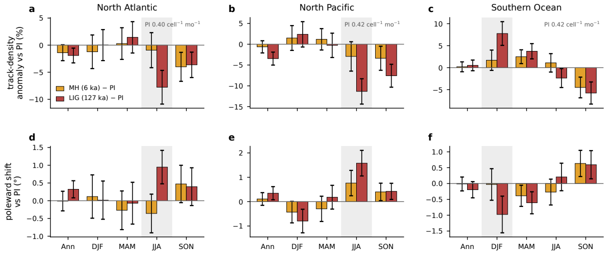
FIG. 9. Seasonal storm response of the real-orbit experiments, tracked with the same pipeline as the main ensemble and referenced to the preindustrial control. (a)–(c) Anomalies of basin-mean track density for the mid-Holocene (gold) and the Last Interglacial (red), as percentages of the preindustrial mean, for the annual mean and the four seasons, with error bars giving twice the standard error of the 30-year difference and the local summer shaded. Track density is normalized per T63 grid cell, and the annotated preindustrial values give the absolute scale in the units of Fig. 4. (d)–(f) The corresponding change in the track-point mean latitude, positive poleward.
