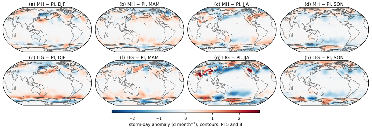
FIG. 10. Storm-day anomalies of the real-orbit experiments relative to the preindustrial control, from the same storm-day product as the main ensemble. (a)–(d) Mid-Holocene minus preindustrial for DJF, MAM, JJA, and SON. (e)–(h) Last Interglacial minus preindustrial. Contours outline the preindustrial climatology at 5 and 8 d month -1 . The isolated warm-season maxima over subtropical continental interiors reflect stationary surface heat lows rather than traveling cyclones.
