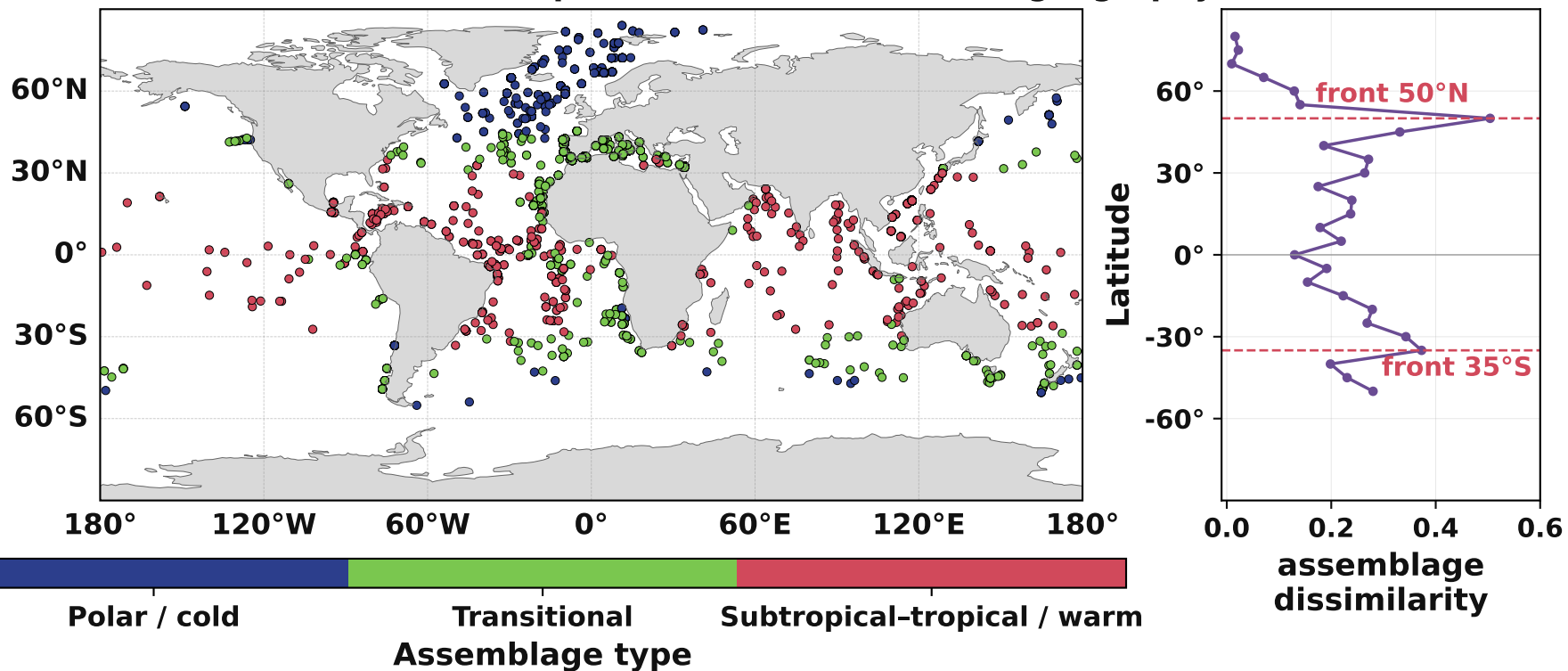
(b) Last Glacial Maximum planktonic foraminifera biogeography
