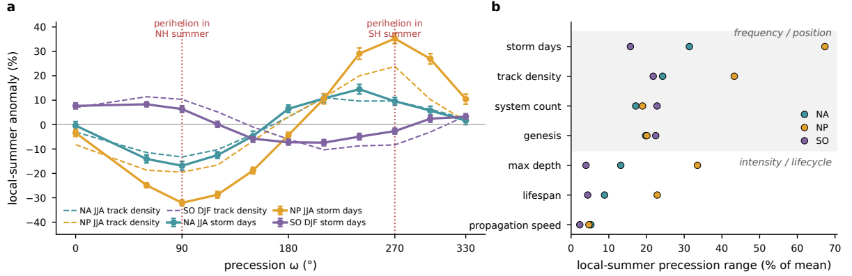
FIG. 7. (a) Local-summer storm activity across the precession cycle, shown as the percent anomaly of basin-mean storm days from the phase mean (solid, with interannual standard errors) and of track density (dashed), for the North Atlantic and the North Pacific in JJA and for the Southern Ocean in DJF; dotted vertical lines mark the phases with perihelion in NH and SH summer. (b) Local-summer across-phase range for frequency and position metrics and for intensity and lifecycle metrics in each basin.
