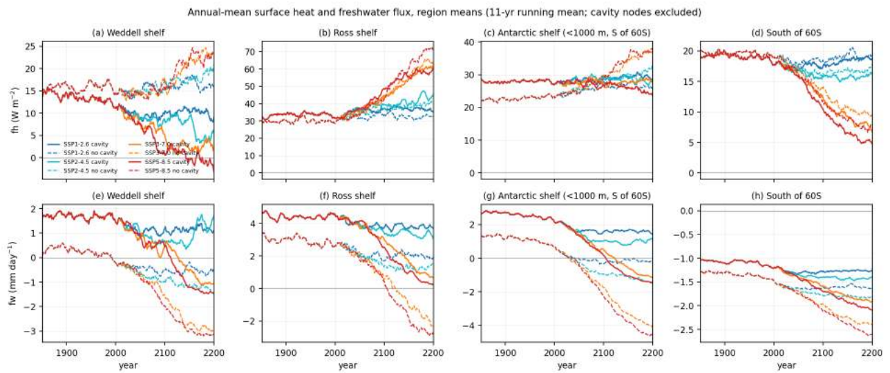
Figure 112: wmt_fig12_flux_timeseries (wmt). Annual-mean fh (top) and fw (bottom) region means 1851-2200 (11-yr running mean) for the same four regions, all scenarios, both sets, cavity nodes excluded. Under SSP5-8.5 the heat loss south of 60S falls from 18 to 5 (cavity) and from 19 to 7 \text{W m}^{-2} (no cavity) by 2171-2200, while on the Ross and Antarctic shelves the heat loss increases (Ross shelf 32 to 58 and 30 to 70 \text{W m}^{-2} ) as the winter ice cover retreats and exposes warmer water. fw becomes more negative everywhere (shelf mean 2.3 to -1.4 and 0.6 to -4.5 \text{mm/day} ) because of more precipitation and less sea-ice formation, and it is this freshening, not the heat flux change, that removes the dense-water formation. Under SSP1-2.6 both fluxes are stable after 2050.
