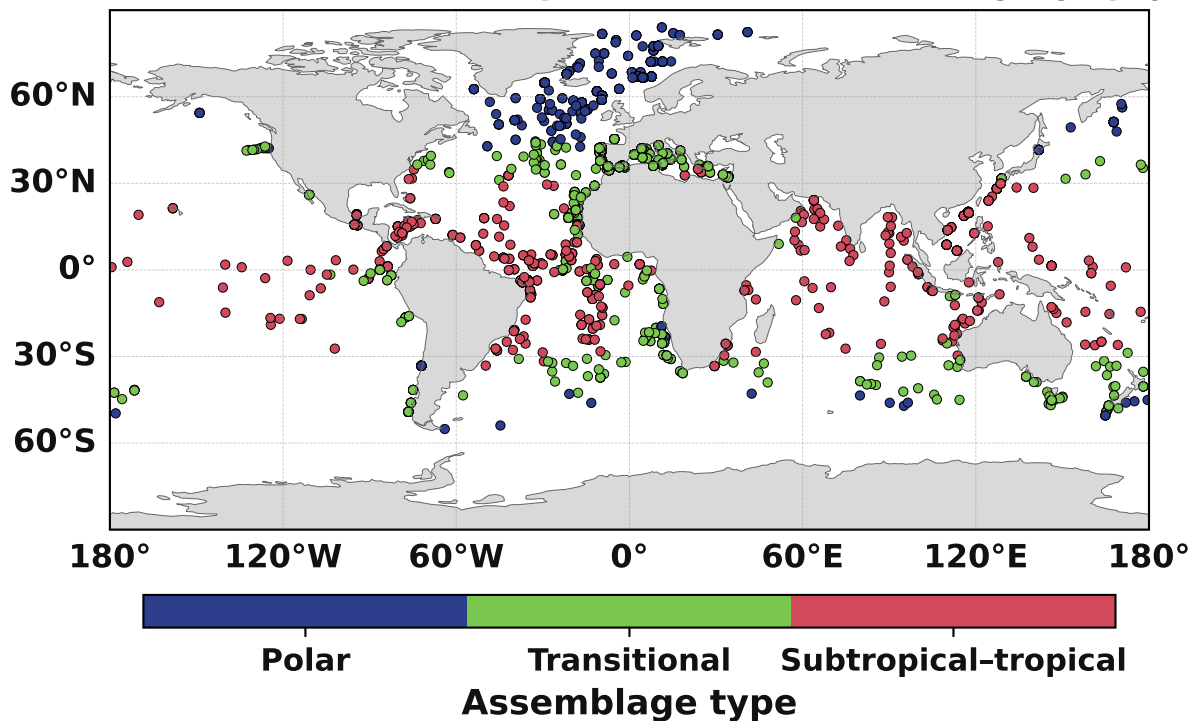
(b) Last Glacial Maximum planktonic foraminifera biogeography
