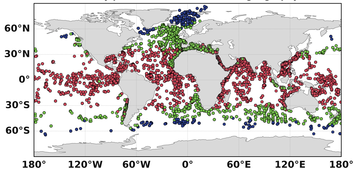
(a) Present-day planktonic foraminifera biogeography
