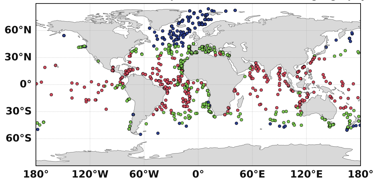
(b) Last Glacial Maximum planktonic foraminifera biogeography
