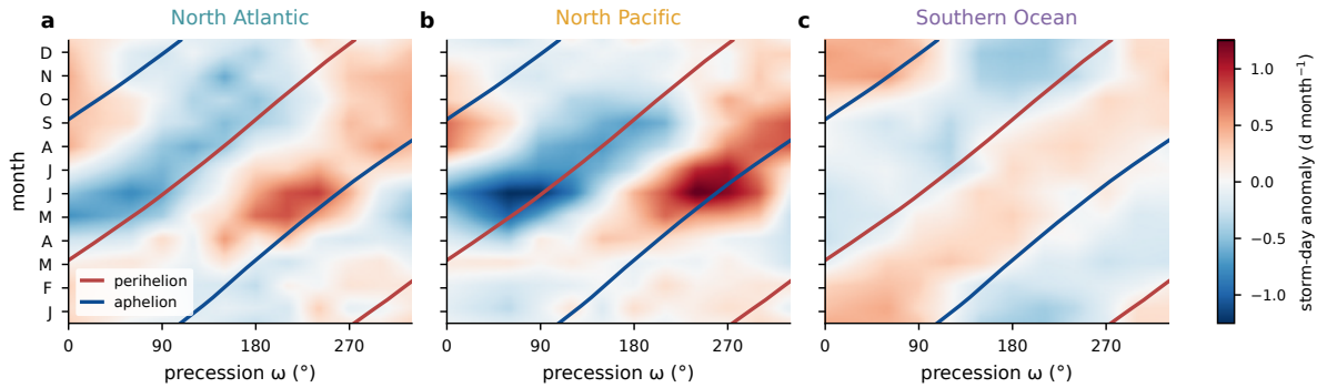
Figure 5: Basin-mean storm-day anomaly (d month -1 ) relative to the phase mean as a function of calendar month and precession phase for (a) the North Atlantic, (b) the North Pacific, and (c) the Southern Ocean, with the perihelion (red) and aphelion (blue) calendar months of each phase overlaid.
