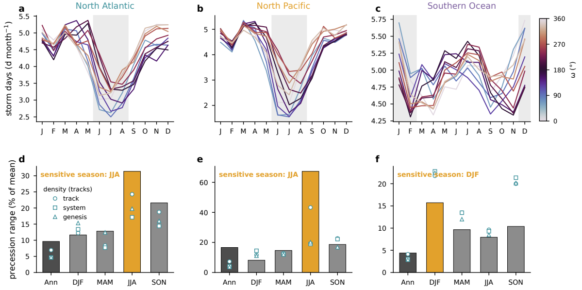
Figure 4: Seasonal concentration of the precessional storm response. (a)–(c) Basin-mean storm days (d month -1 ) by calendar month for the North Atlantic, the North Pacific, and the Southern Ocean, one line per phase colored by \omega , with local summer shaded. (d)–(f) Across-phase range of storm days (maximum minus minimum, percent of the phase mean) for the annual mean and the four seasons, with the local-summer bar highlighted; open symbols give the corresponding ranges of track, system, and genesis densities from the Lagrangian tracks.
