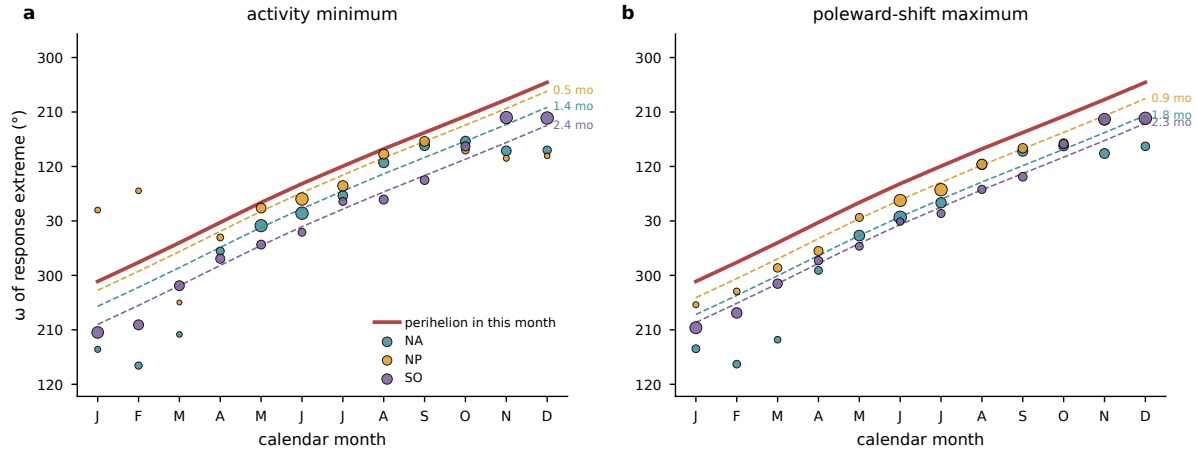
Figure A3: Phase locking of the storm response to the perihelion calendar. For each calendar month and basin, the phase of the first harmonic across the eleven precession phases of (a) basin-mean storm days, shown as the \omega of the activity minimum, and (b) the storm-day-weighted track latitude, shown as the \omega of the poleward maximum. Marker size scales with the harmonic amplitude. The red line gives the \omega that places perihelion in that calendar month, and dashed lines repeat it delayed by each basin's median lag over the amplitude-strong months (annotated in months).
