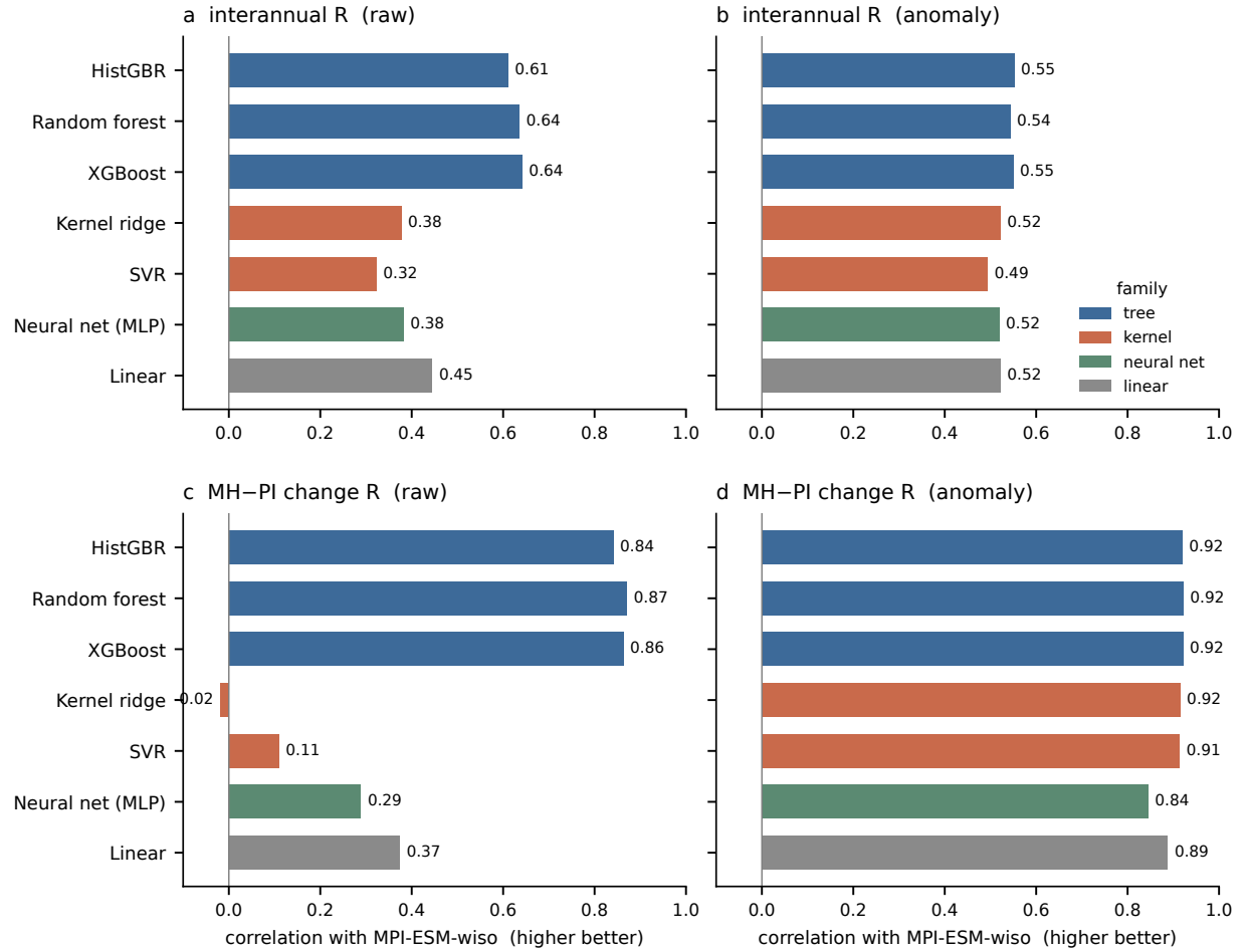
Figure 3: Cross-model skill of seven learners from four families, gradient boosting, random forest and histogram gradient boosting (tree), kernel ridge and support vector regression (kernel), a feed-forward neural network, and ridge regression (linear). (a, b) Precipitation-weighted temporal correlation on MPI-ESM-wiso for the raw and the anomaly framing. (c, d) As in (a)–(b), but for the spatial correlation of the mid-Holocene minus pre-industrial change.
