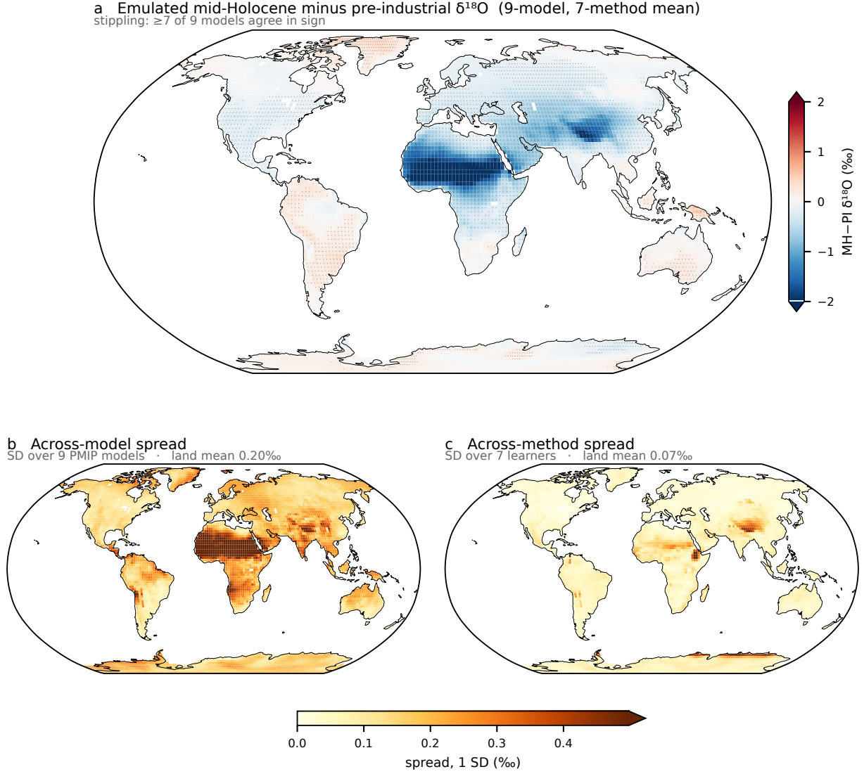
Figure 6: Emulated mid-Holocene minus pre-industrial precipitation \delta^{18}\text{O} across nine PMIP4 models, anomaly framing. (a) Mean over the nine models and the seven learners, with stippling where at least seven of the nine models agree in the sign of the change. (b) Standard deviation across the nine models. (c) As in (b), but across the seven learners. Panels (b) and (c) share one colour scale. Units: ‰.
