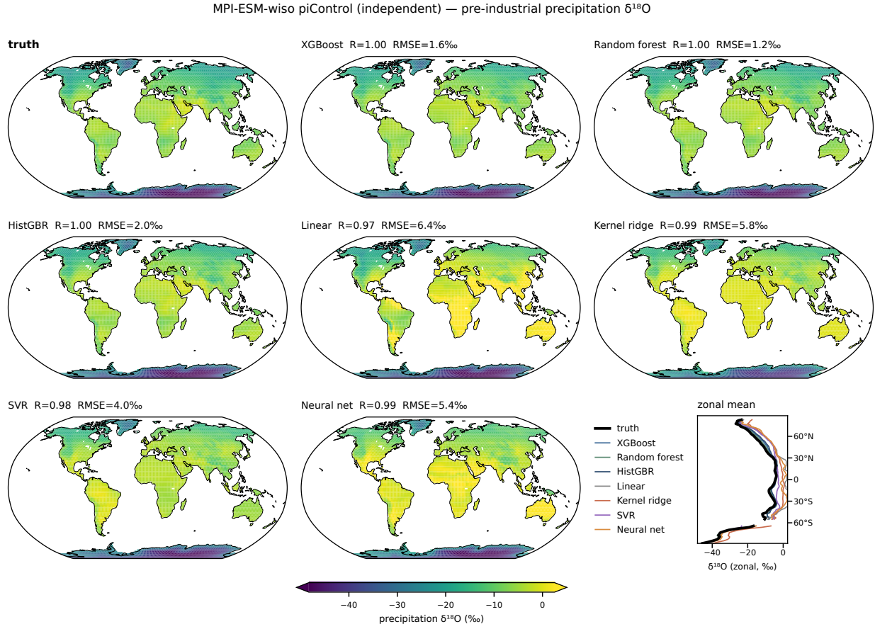
Figure 5: Pre-industrial precipitation \delta^{18}\text{O} of MPI-ESM-wiso. (a) Simulated field. (b)–(h) Emulated field for the seven learners, with the spatial correlation and the root-mean-square error against (a) given in each panel. (i) Zonal mean. Units: ‰.
