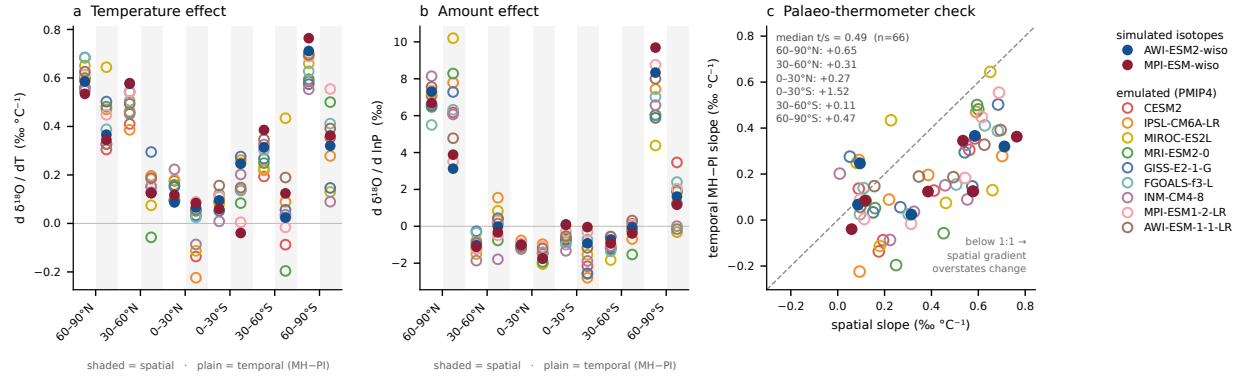
Figure 7: Isotope-climate relations by latitude band. (a) Slope of precipitation \delta^{18}\text{O} against surface temperature, shaded columns for the spatial gradient across grid points and plain columns for the temporal mid-Holocene minus pre-industrial slope. (b) As in (a), but for the slope against the logarithm of precipitation. (c) Temporal against spatial temperature slope, one symbol per model and band, with the 1:1 line and the median ratio per band. Filled symbols mark the two models that simulate water isotopes explicitly and open symbols the nine emulated PMIP4 models.
