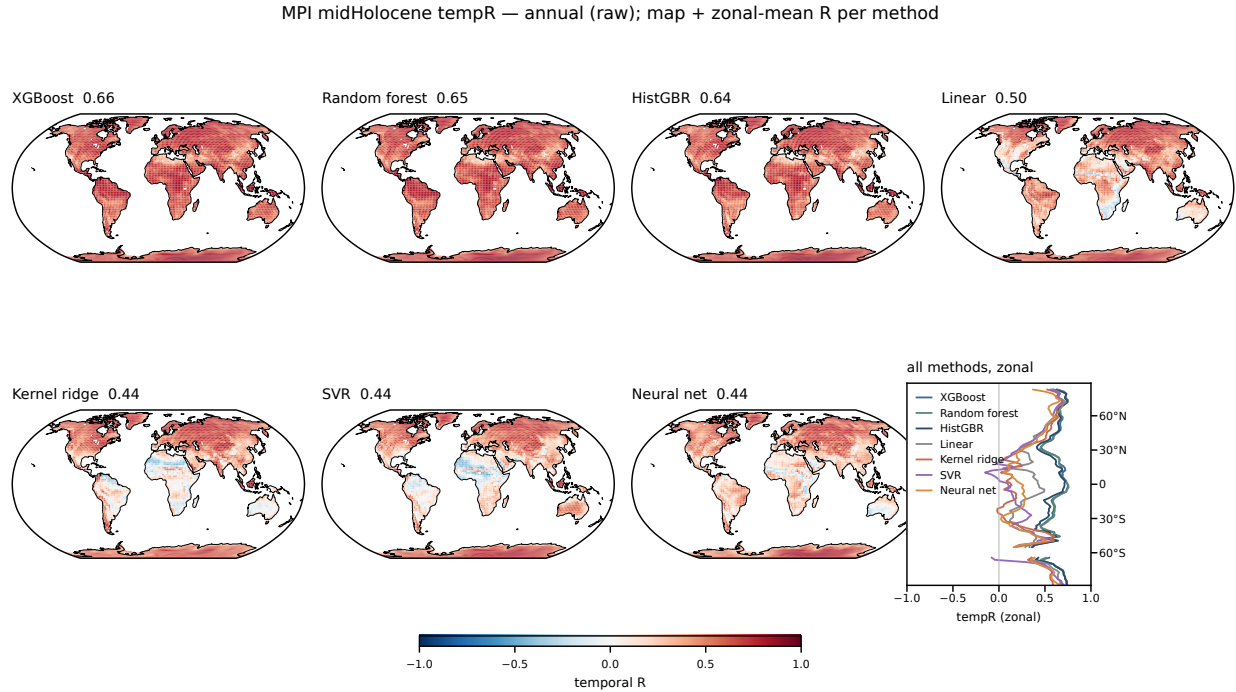
Figure 2: As in Fig. 1, but for the mid-Holocene simulation of MPI-ESM-wiso, a model not used in training.
