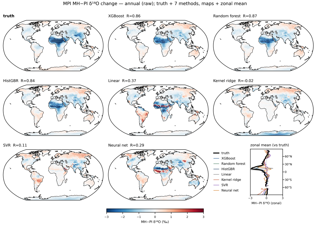
Figure 4: Mid-Holocene minus pre-industrial precipitation \delta^{18}\text{O} in MPI-ESM-wiso, raw framing. (a) Simulated change. (b)–(h) Emulated change for the seven learners, with the spatial correlation against (a) given in each panel. (i) Zonal mean of the change. Units: ‰.
