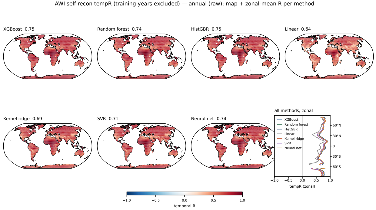
Figure 1: Per-grid-point temporal correlation between the emulated and the simulated annual precipitation-weighted \delta^{18}\text{O} of the AWIESM2-wiso transient, for (a) gradient boosting, (b) random forest, (c) histogram gradient boosting, (d) ridge regression, (e) kernel ridge, (f) support vector regression and (g) a feed-forward neural network. Training years are excluded, leaving 7174 years. Land-mean correlation given in each panel. (h) Zonal mean of the correlation for all seven methods.
