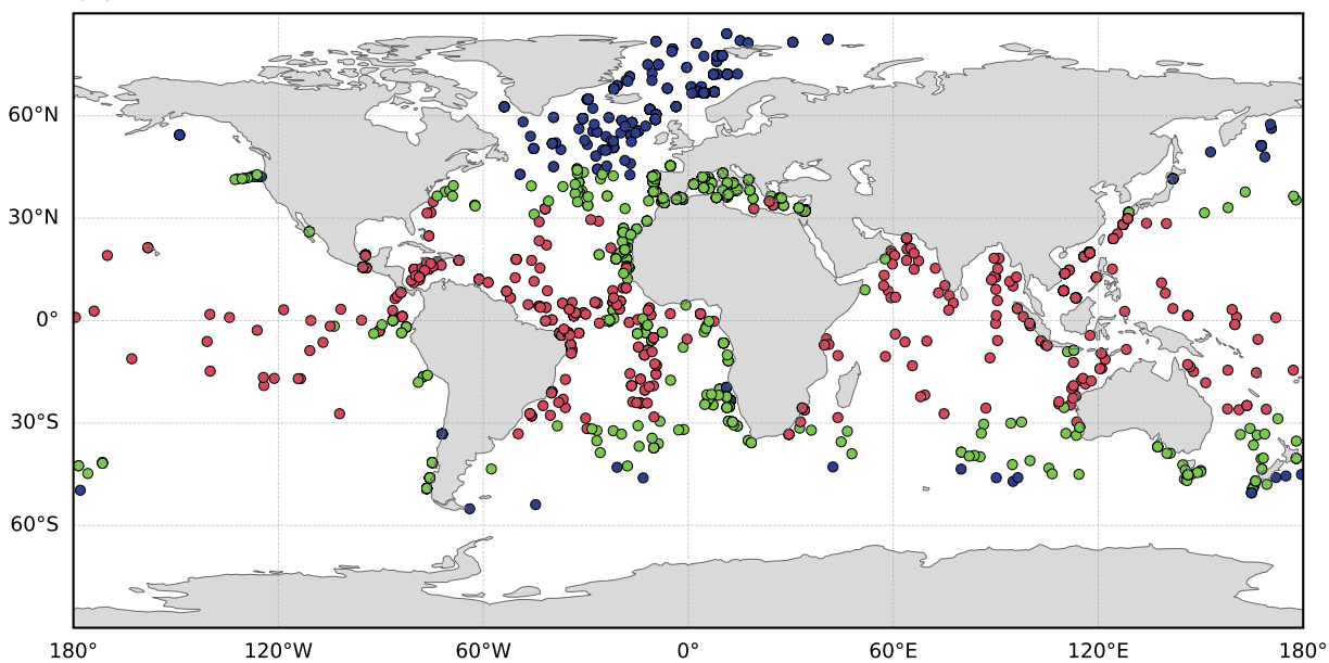
(c) Last Glacial Maximum
