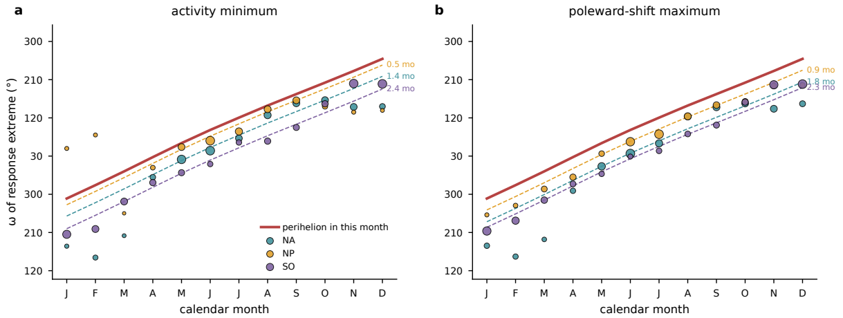
FIG. 8. Phase locking of the storm response to the perihelion calendar. For each calendar month and basin, the phase of the first harmonic across the 12 precession phases of (a) basin-mean storm days, shown as the \omega of the activity minimum, and (b) the storm-day-weighted track latitude, shown as the \omega of the poleward maximum. Marker size scales with the harmonic amplitude. The red line gives the \omega that places perihelion in that calendar month, and dashed lines repeat it delayed by each basin's median lag over the amplitude-strong months (annotated in months).
