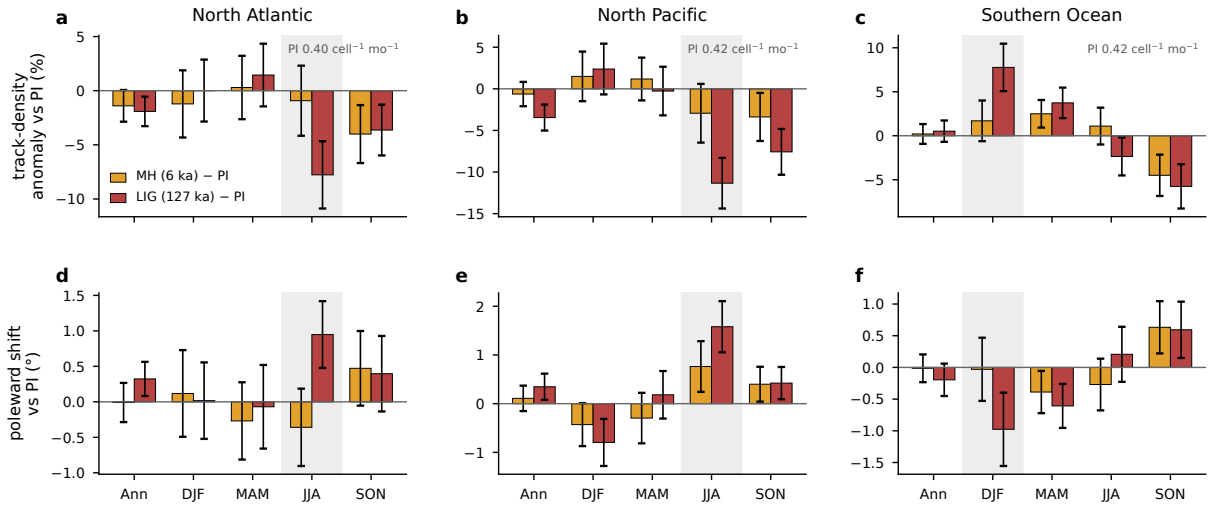
FIG. 9. Seasonal storm response of the real-orbit experiments, tracked with the same pipeline as the main ensemble and referenced to the preindustrial control. (a)–(c) Anomalies of basin-mean track density for the mid-Holocene (gold) and the Last Interglacial (red), as percentages of the preindustrial mean, for the annual mean and the four seasons, with error bars giving twice the standard error of the 30-year difference and the local summer shaded. Track density is normalized per T63 grid cell, and the annotated preindustrial values give the absolute scale in the units of Fig. 4. (d)–(f) The corresponding change in the track-point mean latitude, positive poleward.
