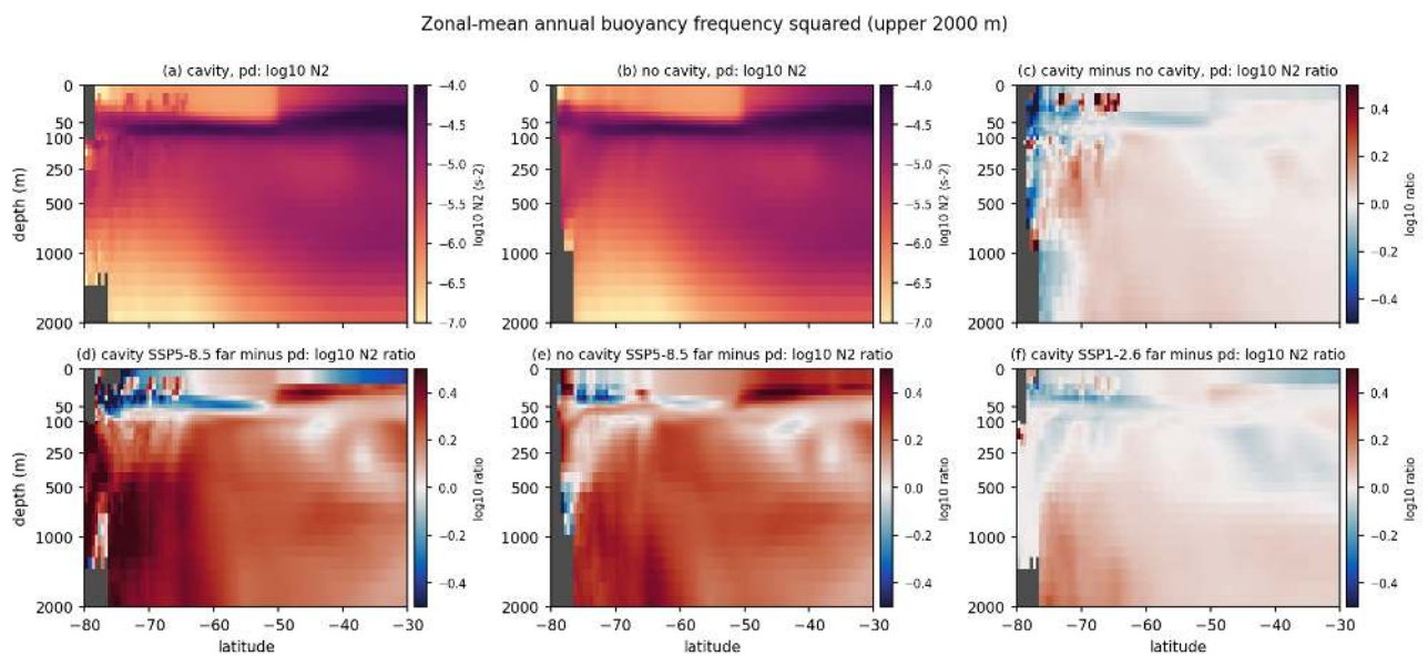
Figure 126: circ_N2_zonal (circ). Zonal-mean annual buoyancy frequency squared (log10 N2, interfaces) in the upper 2000 m. (a) cavity pd, (b) no cavity pd, (c) log10 ratio cavity/no cavity, (d, e) log10 ratio far SSP5-8.5 over pd, (f) far SSP1-2.6 over pd. Take-away: the pycnocline ( N2 > 1e-5 s-2) sits at 50-150 m south of 60S and deepens to 500-1000 m north of 50S. The cavity run is slightly more stratified in the upper 300 m of the 70S-60S band (ratio 1.1-1.3); under SSP5-8.5 N2 in the upper 300 m south of 55S increases by a factor of 1.6-2.0 in both sets.
