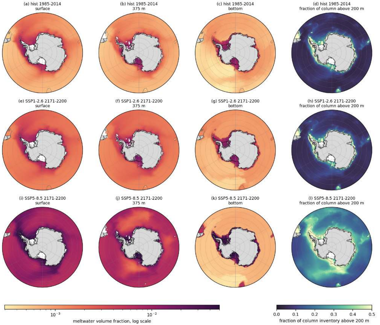
Figure 72: mw_fig07_level_maps (meltwater). Meltwater fraction at the surface (first wet layer, cavity nodes masked), at 375 m, and at the bottom, and the fraction of the column inventory above 200 m, for hist 1985-2014, SSP1-2.6 2171-2200 and SSP5-8.5 2171-2200. Log colour scale for the concentrations. Take-away. At present day the open shelf holds 6.7 permil at the surface and 5.0 permil at the bottom, so the shelf water column is almost uniformly dyed. Over the deep ocean south of 60S the surface has 1.9 permil and the bottom 0.7 permil. Under SSP5-8.5 the far-future surface reaches 37 permil on the shelf and 13 permil over the deep ocean while the deep-ocean bottom stays at 0.7 permil. The fraction above 200 m over the deep ocean rises from 10 to 29 percent. The additional meltwater is trapped in the upper ocean.
