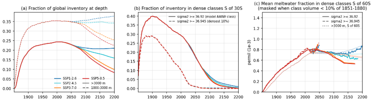
Figure 76: mw_fig11_abyss (meltwater). Does meltwater reach the abyss. (a) Fraction of the global inventory below 3000 m (solid) and between 1000 and 3000 m (dashed). (b) Fraction of the inventory south of 30S found in the model-relative AABW class sigma2 at or above 36.92 and in the densest class at or above 36.945 (TEOS-10). (c) Mean meltwater fraction inside those classes south of 60S, masked once the class volume drops below 10 percent of its 1851-1880 volume, with the mean below 3000 m south of 60S dotted. Take-away. The share below 3000 m peaks at 24 percent around 2000 and falls to 9 percent by 2171-2200 under SSP5-8.5 and 21 percent under SSP1-2.6. The dense classes hold 29 percent (36.92) and 10 percent (36.945) of the inventory at present day at a concentration of 0.76 and 0.79 permil, the same as the deep mean, so the meltwater is mixed into the deep water rather than concentrated in the densest water. The classes themselves vanish after 2100 because of the deep drift and warming, not because the dye leaves them. The deep concentration below 3000 m south of 60S stays at 0.67 permil (pd) to 0.66 permil (SSP5-8.5 far) and rises only to 0.85 permil under SSP1-2.6.
