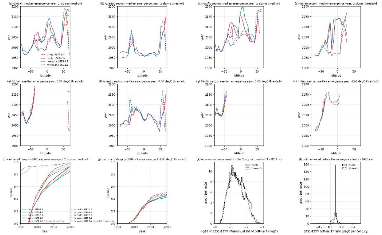
Figure 171: fig09_toe_latitude_summary (propagation). Panels (a) to (d) give the area-weighted median emergence year of bottom temperature (2 sigma threshold) per 5 deg latitude band for nodes deeper than 3000 m, globally and per sector, for SSP5-8.5 (red) and SSP1-2.6 (blue), cavity (solid) and no cavity (dashed). Panels (e) to (h) repeat this for the 0.05 degC threshold. Panel (i) shows the fraction of deep (>3000 m) sea floor area emerged as a function of time for all four scenarios and both sets with the 2 sigma threshold, plus the SSP5-8.5 result without drift correction in grey. Panel (j) is the same for the 0.05 degC threshold. Panels (k) and (l) are area-weighted histograms of the interannual noise and of the removed 1851-1950 drift for the deep nodes. Take-away. Without drift correction 80 to 85 percent of the deep sea floor has "emerged" by 1900, which shows that the raw emergence is drift, not forcing. With the 0.05 degC threshold the emerged fraction is 10 percent in 2014, 36 to 41 percent in 2100 and 42 to 50 percent in 2200, with little dependence on scenario (the emerged area in SSP1-2.6 is only 3 to 5 percent smaller than in SSP5-8.5). Median emergence (0.05 degC) is 2005 to 2030 at 55 to 70S and 2045 to 2085 in the Atlantic between 30S and 40N.
