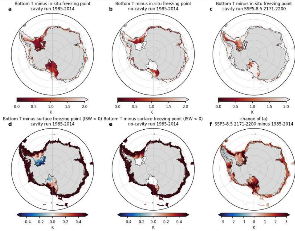
Figure 97: bottom_freezing (bottom). Bottom potential temperature minus the in-situ freezing point (a-c, K, gsw, using bottom salinity and depth) and minus the surface freezing point (d,e, negative = Ice Shelf Water) for the shelf and slope shallower than 2500 m, 1985-2014 cavity run (a,d, cavity nodes included), no-cavity run (b,e) and cavity run SSP5-8.5 2171-2200 (c), with the change (f). Black line 1000 m isobath. Bottom water within 0.5 K of the in-situ freezing point covers 19 percent of the Weddell shelf in the cavity run (9 percent without cavities) and 5 to 6 percent of the Ross shelf. Water below the surface freezing point exists only under and in front of the Filchner-Ronne and Ross ice shelves in the cavity run. By 2171-2200 under SSP5-8.5 the shelf bottom is 1.5 to 3 K further from freezing, except under the Filchner-Ronne cavity where the water cools slightly.
