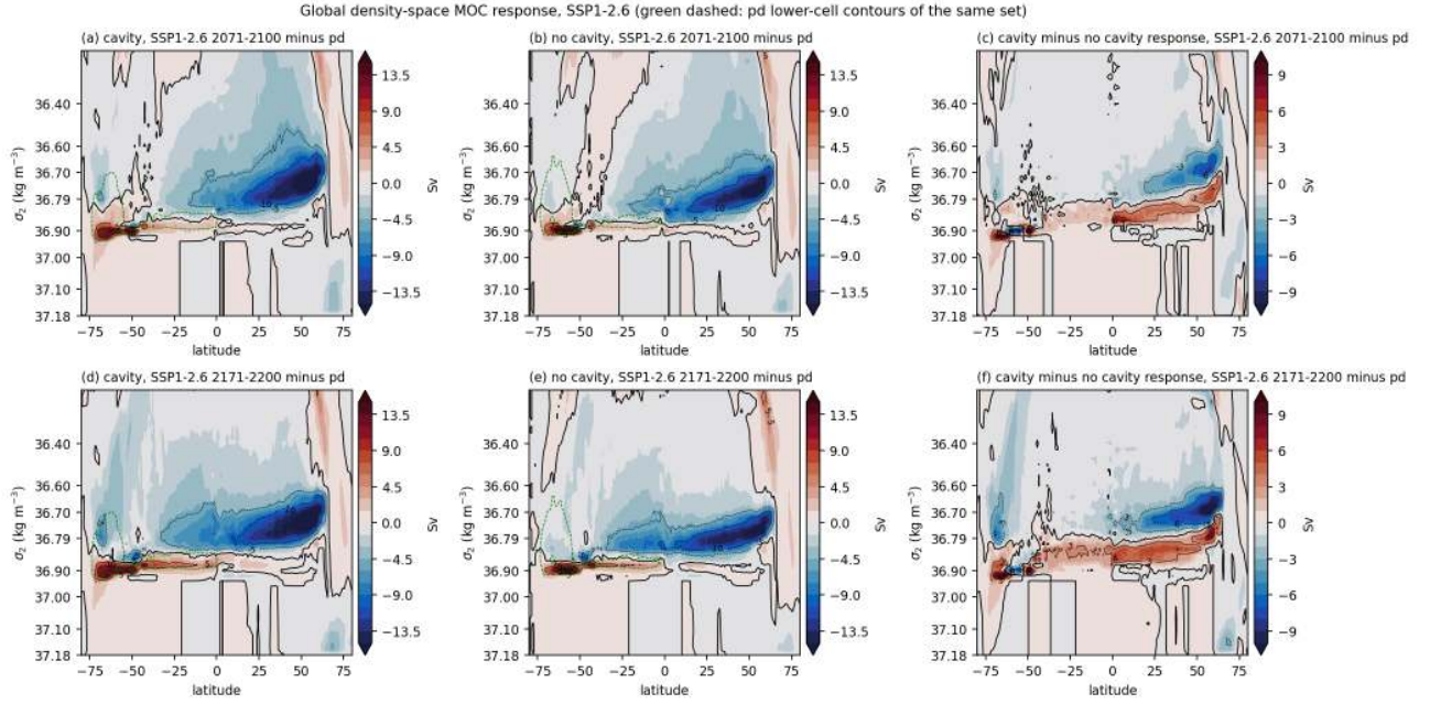
Figure 140: moc_dens_response_ssp126 (moc). As moc_dens_response_ssp585 for SSP1-2.6. The dense lower cell south of 50S still weakens by 5-15 Sv in both sets by 2071-2100 and only partly recovers by 2171-2200. The NADW-class weakening is 10 Sv at 2071-2100 and smaller afterwards.
