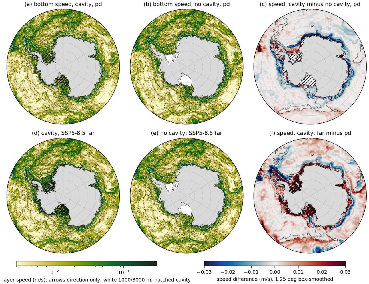
Figure 118: circ_bottom_velocity (circ). Bottom-layer (deepest wet layer of each element) speed (log colour) with direction arrows south of 55S; white contours 1000 and 3000 m isobaths, hatched = ice-shelf cavities. (a) cavity pd, (b) no cavity pd, (c) speed difference cavity minus no cavity (1.25 degree box smoothed), (d) cavity SSP5-8.5 far, (e) no cavity SSP5-8.5 far, (f) cavity far minus pd. Take-away: the strongest bottom flow (0.05-0.3 m/s) is the westward Antarctic Slope Current over the 1000-3000 m band and the cyclonic rims of the Weddell and Ross gyres; there is no distinct down-slope dense plume signature at the Filchner, Ross or Adelie sills. Mean bottom speed over the circumpolar slope band (1000-3000 m, S of 60S) is 0.024 m/s (cavity) versus 0.032 m/s (no cavity), the westward component -0.012 versus -0.019 m/s, so the slope current is about 35 percent weaker in the cavity run (the shelf geometry differs, see caveats). Under SSP5-8.5 the slope current weakens further in the no-cavity run (-0.015 m/s) and is unchanged in the cavity run, while under-ice-shelf currents in the FRIS and Ross cavities accelerate by 0.01-0.03 m/s.
