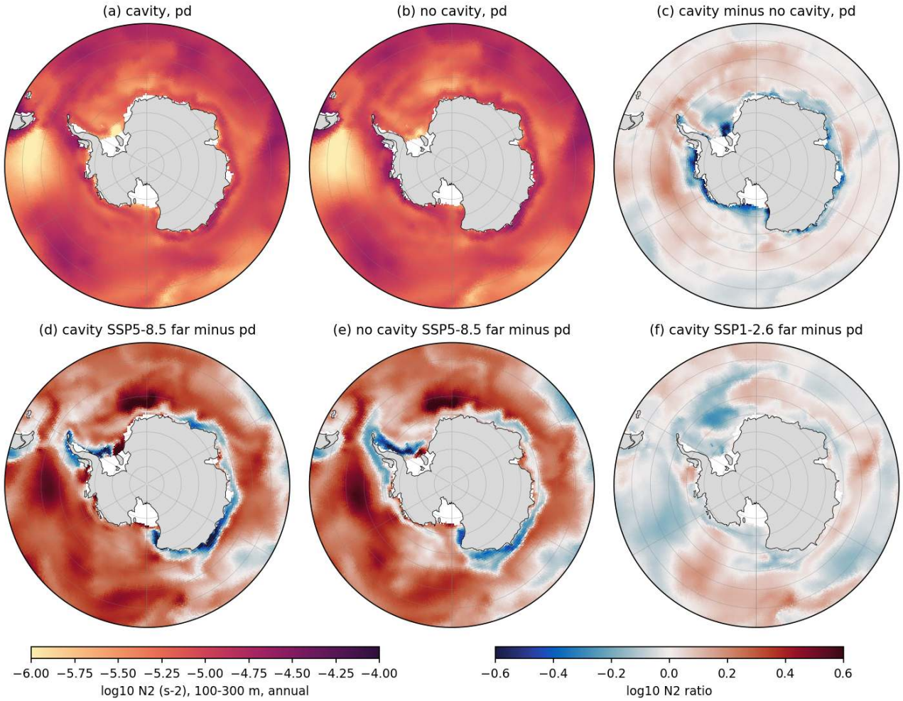
Figure 127: circ_N2_maps (circ). Maps south of 50S of \log_{10} N_2 averaged over 100-300 m (annual), same panel layout as above (cavity nodes excluded). Take-away: at pd the weakest 100-300 m stratification ( N_2 about 5e-6 s-2) is found over the Ross shelf in the cavity run ( 5.1e-6 versus 8.1e-6 in the no-cavity run) and near Maud Rise in the no-cavity run ( 4.7e-6 versus 5.3e-6 ), matching where each set convects. Under SSP5-8.5 N_2 south of 60S increases by 60-70 percent (ssa mean 7.7e-6 to 1.28e-5 cavity, 7.9e-6 to 1.18e-5 no cavity), except on the East Antarctic and Ross shelves where it decreases (blue rings) as the winter halocline erodes.
