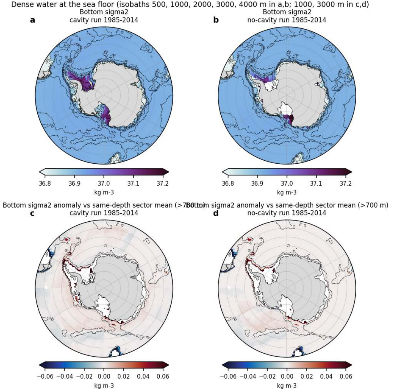
Figure 98: bottom_pathways (bottom). Bottom sigma2 (a,b; isobaths 500, 1000, 2000, 3000, 4000 m) and bottom sigma2 anomaly relative to the area mean of all nodes in the same 30 degree longitude sector and 250 m bottom-depth bin, shown for depths greater than 700 m (c,d; isobaths 1000 and 3000 m), 1985-2014, cavity run (a,c) and no-cavity run (b,d). Dense shelf water (above 37.0 kg m -3 ) is confined to the western Weddell and Ross shelves and does not reach below the 1000 m isobath as a coherent dense layer in either run. Positive anomalies on the slope mark the Filchner trough mouth, the western Ross slope and the Adelie and Prydz Bay shelf breaks, with amplitudes of only 0.02 to 0.05 kg m -3 .
