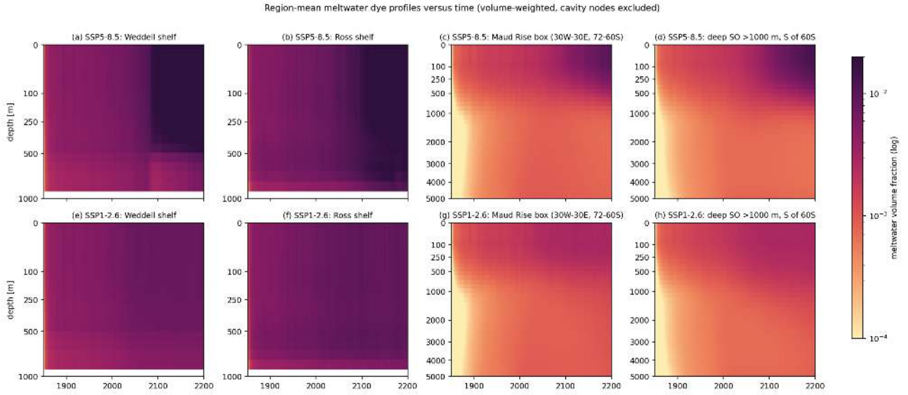
Figure 81: mw_fig16_hovmoeller_regions (meltwater). Region-mean meltwater profiles versus time for the Weddell shelf, Ross shelf, Maud Rise box and the deep Southern Ocean south of 60S, SSP5-8.5 (top) and SSP1-2.6 (bottom). Take-away. Both shelves are dyed through the whole column at present day (surface 6 to 7 permil, bottom 4 to 5 permil). On the Ross shelf the present-day maximum is at 535 m, a deep outflow of cavity water, and under SSP5-8.5 the maximum moves to 35 m and the shelf surface reaches 40 permil. The deep Southern Ocean below 1000 m shows no scenario dependence.
