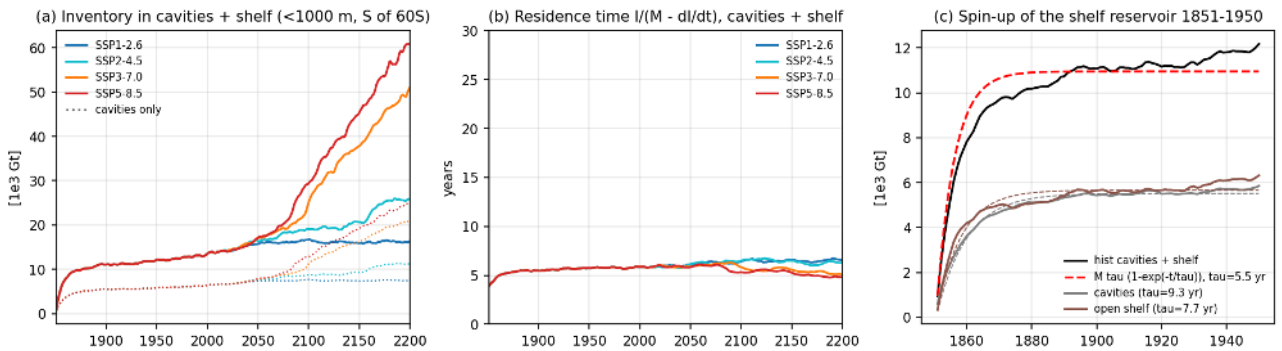
Figure 70: mw_fig05_shelf_residence (meltwater). Shelf reservoir. (a) Inventory in the cavities plus the open shelf south of 60S, with the cavity part dotted. (b) Residence time estimated as inventory divided by melt input minus inventory growth, with 11 yr smoothing. (c) Build-up of the reservoir 1851-1950 and exponential fits of the form M \tau (1 - \exp(-t/\tau)) with the mean melt M of 1851-1950, and separate fits for cavities and open shelf. Take-away. The cavity plus shelf reservoir equilibrates within a few decades at 11e3 Gt ( 13.4e3 Gt at present day, 57e3 Gt in 2171-2200 under SSP5-8.5). The residence time is 5 to 6 years at present day and 5 to 6.5 years in all scenarios. The single-exponential fit gives 5.5 yr for the combined reservoir. The cavity-only reservoir is 6.4e3 Gt at present day, about 3 years of melt.
