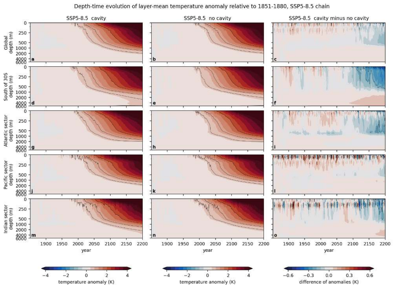
Figure 157: hov_depth_temp_ssp585 (census). Depth-time Hovmoeller of the layer-mean temperature anomaly relative to 1851-1880 for the SSP5-8.5 chain, global, south of 30S, Atlantic, Pacific and Indian sectors (rows), cavity (left), no cavity (middle) and cavity minus no cavity (right, note the smaller colour range). The depth axis is stretched above 500 m. Warming of more than 0.5 K reaches 1000 m globally by 2100 and 2000 m by 2200, the abyss warms by 0.1-0.3 K through drift. The cavity run warms less in the upper 500 m south of 30S after 2100 (by up to 0.6 K, the sea-ice and surface feedback discussed by the atmos theme) but slightly more below 2000 m (0.05-0.1 K).
