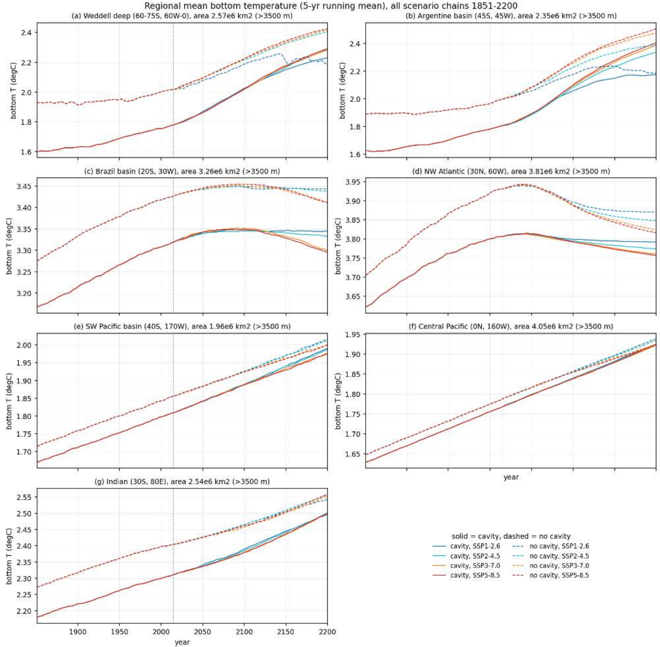
Figure 177: fig14_regional_btemp_timeseries (propagation). Area-weighted bottom temperature (5-yr running mean) of seven regional boxes restricted to depths below 3500 m for all four scenario chains 1851-2200, cavity solid and no cavity dashed, scenario colours. Boxes are the deep Weddell Sea (60-75S, 60W-0E), the Argentine basin (38-52S, 58-35W), the Brazil basin (12-28S, 38-20W), the NW Atlantic (24-36N, 75-45W), the SW Pacific basin (34-46S, 180-160W), the central Pacific (7S-7N, 172-148W) and the Indian Ocean (23-37S, 70-92E). Take-away. Deep Weddell bottom water is 1.76 degC (cavity) and 2.00 degC (no cavity) at present day and warms to 2.26 and 2.41 degC by 2171-2200 under SSP5-8.5 (0.29 and 0.25 degC per century in 2015-2100). The Southern Ocean boxes warm almost identically in all four scenarios; the spread between SSP1-2.6 and SSP5-8.5 at 2200 is only 0.05 degC in the Weddell and 0.2 degC in the Argentine basin. The Brazil basin and NW Atlantic warm until 2050-2090 (drift) and then cool under the stronger scenarios (-0.05 degC per century in 2101-2200 for SSP5-8.5). The Pacific boxes follow the drift line (0.08 to 0.09 degC per century) with no visible scenario response.
