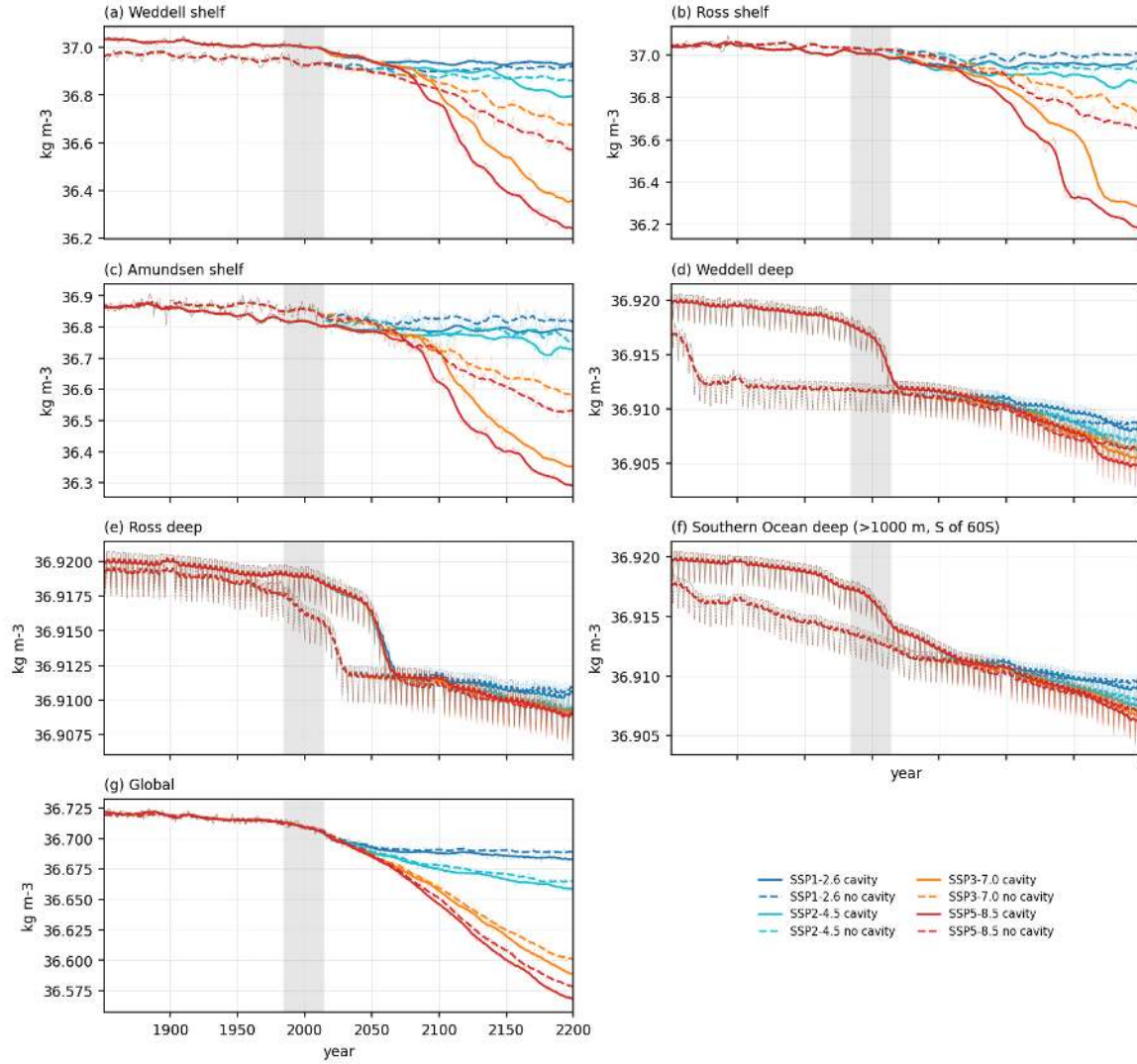
Figure 89: bottom_ts_Sig (bottom). Same as bottom_ts_T for bottom sigma2 (kg m -3 ). Shelf bottom density decreases in all scenarios, deep-basin density is almost constant (changes below 0.01 kg m -3 ) because the deep warming and salinification compensate.
