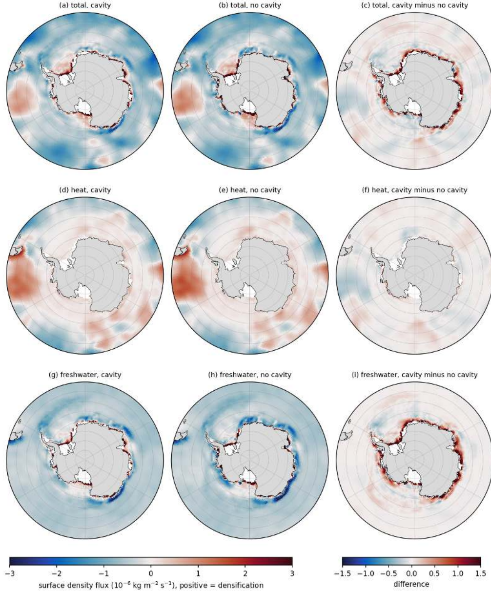
Figure 112: wmt_fig13_map_density_flux_pd (wmt). Present-day annual-mean surface density flux ( 10^{-6} \text{ kg m}^{-2} \text{ s}^{-1} , positive is densification) south of 50S from the FESOM class diagnostics summed over classes (heat plus freshwater, restoring not included in the maps), for the cavity run (left), the no-cavity run (middle) and the difference (right) for the total (a-c), the heat part (d-f) and the freshwater part (g-i). Densification is confined to a narrow coastal band (coastal polynyas and the shelves, shelf mean +0.82 and +0.46 units) and to the Drake Passage/Agulhas sector of the ACC (heat loss), while the gyres and the open Southern Ocean are lightened (south of 50S mean -0.48 and -0.49 , freshwater part -0.45 and -0.49 ). The cavity run densifies the coastal band more strongly (difference up to +1.5 at the coast) because it has no coastal runoff; away from the coast the two sets differ by less than 0.2 units.
