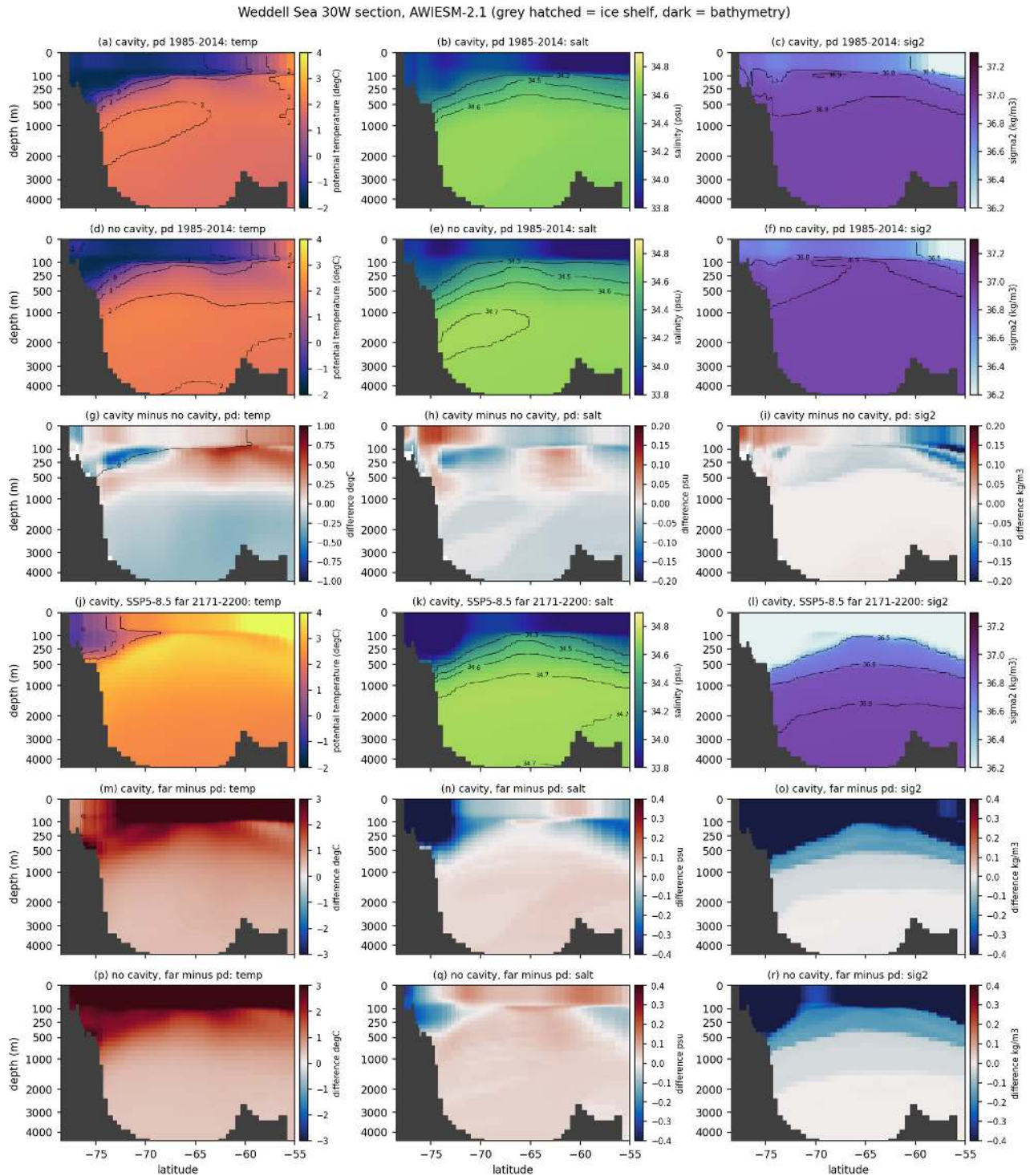
Figure 120: circ_sec_weddell30W (circ). As above for 30W, 78.5S-55S across the southern Weddell Sea (Filchner/Ronne shelf to the gyre centre). Take-away: shelf bottom water at pd is -1.1 degC, 34.16 psu (cavity) and -1.0 degC, 34.18 psu (no cavity), about 0.3 psu too fresh for HSSW, and the deep basin bottom is 1.75 and 1.98 degC. The densest shelf water (sigma2 36.9) is lighter than the 36.9 water filling the basin below 1000 m, so shelf water cannot sink to the bottom. In 2171-2200 the shelf bottom warms to 1.3 degC (cavity) and 1.7 degC (no cavity) and the shelf freshens by 0.45 and 0.16 psu.
