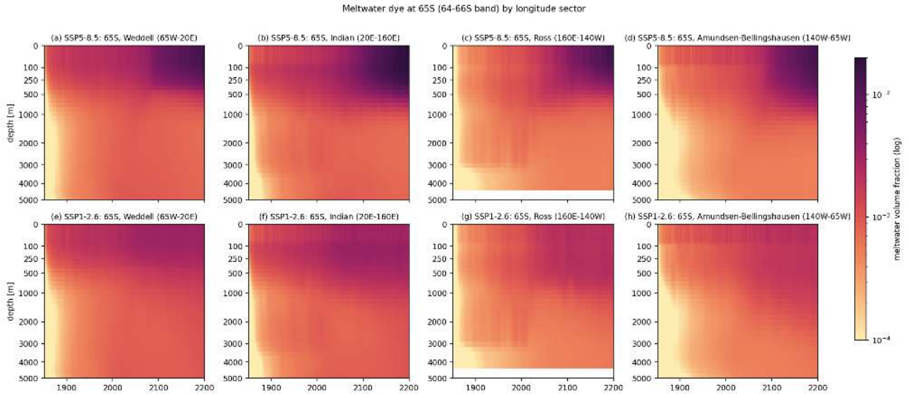
Figure 82: mw_fig17_hovmoeller_sectors (meltwater). Meltwater fraction versus depth and time in the 64-66S band for the four longitude sectors, SSP5-8.5 (top) and SSP1-2.6 (bottom). Take-away. The Weddell sector is the only one where the dye reaches the bottom at 65S within decades (0.85 permil below 3000 m at present day against 0.38 in the Ross and 0.44 in the Amundsen sector). It is the route of meltwater into the abyss in this model. Under SSP5-8.5 the Weddell deep concentration decreases to 0.79 permil by 2171-2200 while the surface reaches 13 permil, so the deep route weakens when melt increases.
