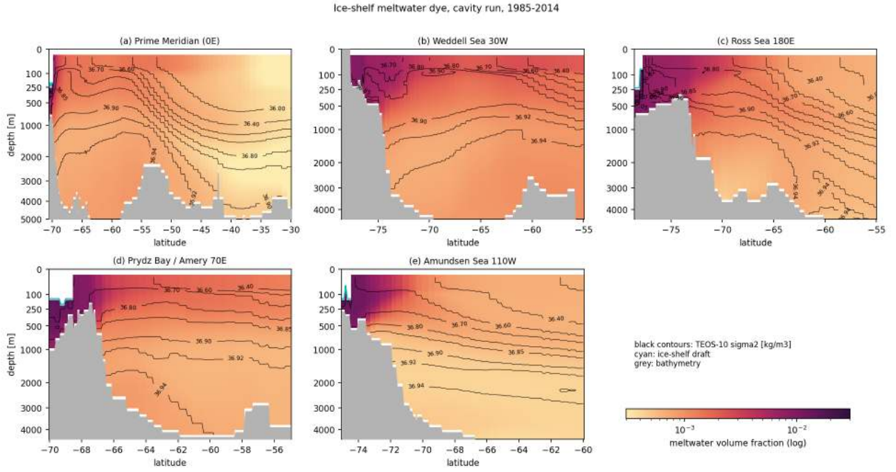
Figure 73: mw_fig08_sections_pd (meltwater). Meridional sections of the meltwater fraction (log scale) with TEOS-10 sigma2 contours for hist 1985-2014 along the prime meridian, 30W (Weddell), 180E (Ross), 70E (Prydz Bay) and 110W (Amundsen), the lines used by the circ theme. Cyan marks the ice-shelf draft, grey the bathymetry. Take-away. The dye maximum on the continental slope sits in the upper 50 to 210 m (4 permil at 30W and 180E). On the slope the bottom concentration is 0.8 to 0.9 permil at 0E, 30W and 180E and 1.7 permil at 70E where the Amery outflow leaves the shelf at depth. At 180E the 60S column has its maximum at 735 m, a mid-depth tongue along the slope. There is no dense bottom plume carrying meltwater down the slope at high concentration.
