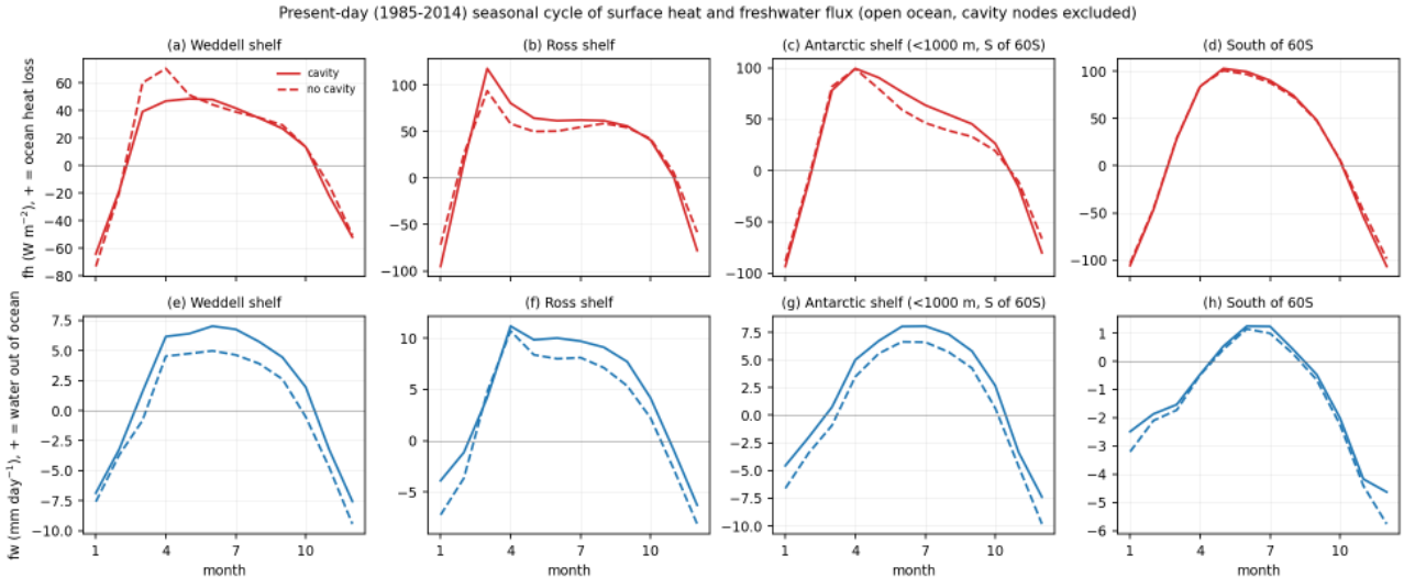
Figure 110: wmt_fig11_flux_seasonal_cycle (wmt). Present-day (1985-2014) seasonal cycles of the region-mean surface heat flux fh (top, W m -2 , positive is ocean heat loss) and freshwater flux fw (bottom, mm/day, positive is water leaving the ocean, that is the sum of evaporation minus precipitation, sea-ice freezing minus melting and minus runoff) for the Weddell shelf, Ross shelf, the whole Antarctic shelf (depth below 1000 m, south of 60S) and the region south of 60S, both sets, cavity nodes excluded. Winter (JJA) heat loss is 41 and 39 W m -2 on the Weddell shelf, 62 and 55 on the Ross shelf, 65 and 48 on the whole shelf and 88 and 86 south of 60S (cavity, no cavity). Winter fw is 6.5 and 4.5 mm/day on the Weddell shelf, 9.6 and 7.7 on the Ross shelf, meaning that net brine release in the cavity run is larger. A large part of this difference is not sea ice: in the no-cavity run 1.1 to 1.8 mm/day of runoff enters at the coast (ice-sheet discharge routed by the HD model) and is included in fw , in the cavity run this water enters as melt under the ice shelves (2360 Gt/yr) at the excluded cavity nodes and runoff south of 60S is zero. Sea-ice brine and precipitation minus evaporation cannot be separated in the fw output.
