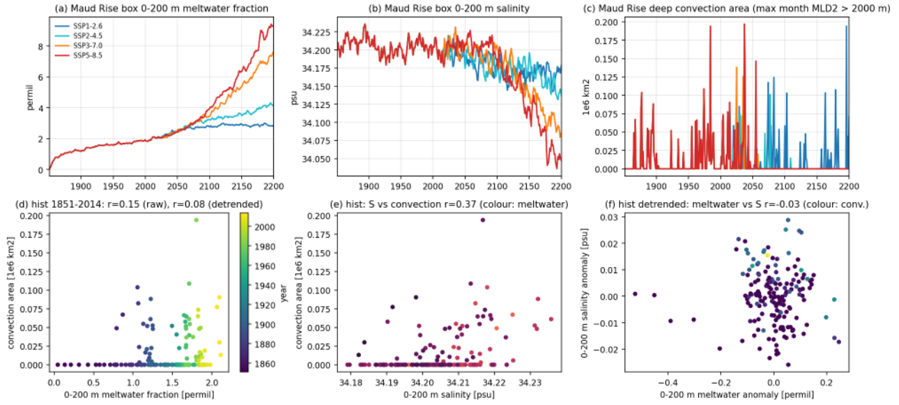
Figure 77: mw_fig12_maud (meltwater). Maud Rise (30W-30E, 72-60S, depth over 1000 m, cavity nodes excluded). (a) 0-200 m meltwater fraction, (b) 0-200 m salinity, (c) deep convection area (maximum monthly area with MLD2 over 2000 m in the box, from cache/seaice), (d) scatter of meltwater fraction versus convection area in 1851-2014 with correlations raw and with a quadratic trend removed, (e) salinity versus convection area, (f) detrended meltwater versus detrended salinity. Take-away. The present-day upper-ocean meltwater fraction is 1.9 permil (0.8 permil in 1851-1880), a dilution equivalent to 0.065 psu. Its interannual anomalies are 0.1 permil (0.003 psu), far smaller than the 0.02 psu salinity variability. The correlation of meltwater with convection is 0.15 (0.08 detrended) and salinity versus convection 0.37, so interannual meltwater variability does not control convection events. The mean meltwater freshening sets the background. Under SSP5-8.5 the fraction reaches 8.7 permil (0.3 psu equivalent) by 2171-2200 and convection stops after 2050.
