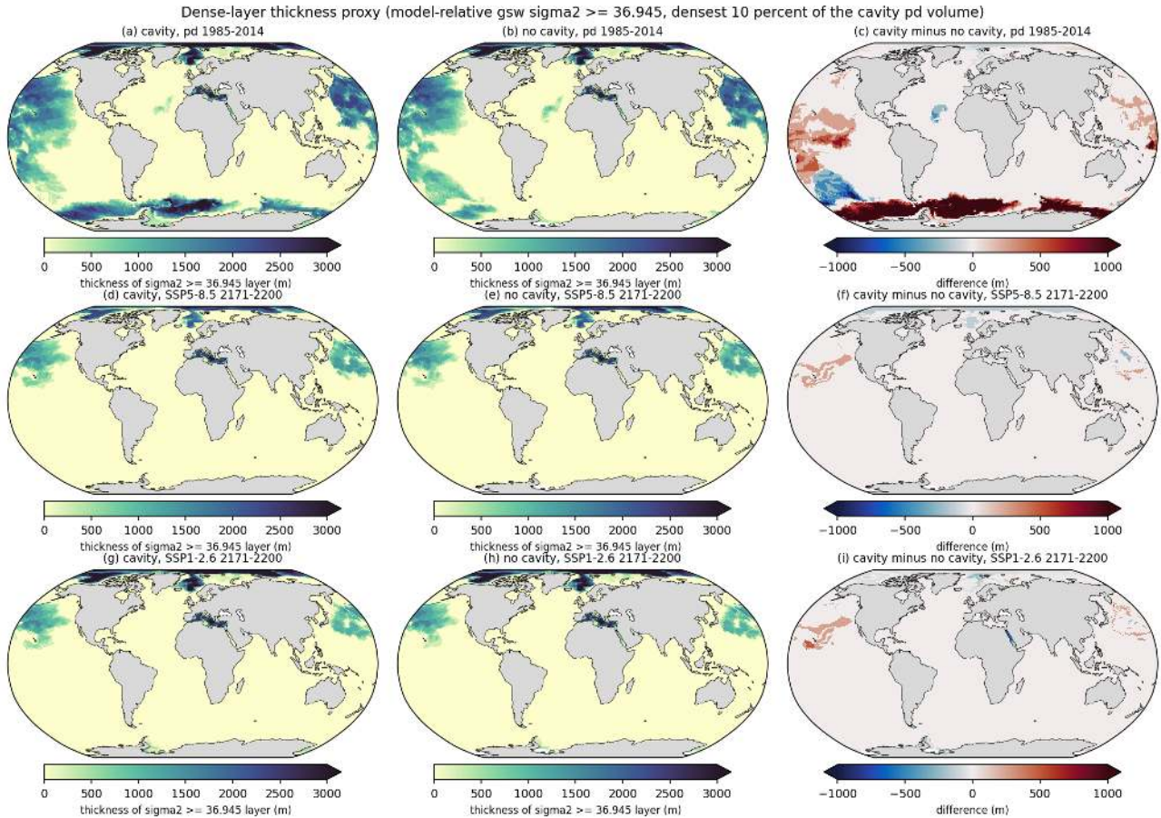
Figure 174: fig12_aabw_thickness_maps (propagation). Thickness (m) of the water column with gsw sigma2 \geq 36.945 , computed from the period-mean temperature and salinity ('cache/pmean') with the wet mask applied. The threshold is the volume-weighted 90th percentile of the cavity-run 1985-2014 sigma2 (densest 10 percent of the ocean volume), a model-relative definition of the densest class. Rows are pd 1985-2014, SSP5-8.5 2171-2200 and SSP1-2.6 2171-2200; columns cavity, no cavity, cavity minus no cavity. Take-away. At present day the densest class fills the abyssal Southern Ocean south of 55S (1200 m mean thickness south of 60S in the cavity run, 175 m in the no-cavity run, where only the Weddell abyss is dense enough) but it is also present in the North Pacific, the Arctic and the Mediterranean, because the model abyss has a nearly uniform sigma2 of 36.94 to 36.98 from 70S to 60N (fig13) and the North Pacific is marginally denser than the Weddell abyss. By 2171-2200 the dense class has disappeared completely from the Southern Ocean in both scenarios and both sets (mean thickness south of 60S 0 to 14 m); globally the dense volume drops from 1.32 (cavity) and 0.94 (no cavity) to 0.30 to 0.34 \times 10^{17} m 3 .
