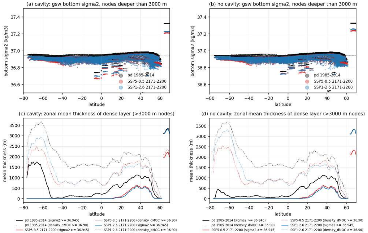
Figure 176: fig13_bottom_sigma2_latitude (propagation). Panels (a) and (b) give the gsw bottom sigma2 of a random subset of nodes deeper than 3000 m versus latitude for pd (black), SSP5-8.5 2171-2200 (red) and SSP1-2.6 2171-2200 (blue), cavity and no cavity; the dotted line is the 36.945 threshold. Panels (c) and (d) give the zonal mean thickness of the dense layer for both definitions (solid gsw sigma2 \geq 36.945 , dotted density_dMOC \geq 36.90 as used by the census theme). Take-away. The abyss has a remarkably uniform bottom sigma2 of 36.94 to 36.98 at present day with the densest values in the North Pacific and North Atlantic (36.97 to 36.98) and the lightest in the deep Southern Ocean (36.94 to 36.95); there is no dense southern end member. By 2200 bottom sigma2 drops to 36.85 to 36.92 everywhere. The density_dMOC layer definition gives thicknesses two to three times larger and does not reproduce the cavity minus no-cavity contrast, because density_dMOC is nearly constant (36.91 to 36.92) below 700 m.
