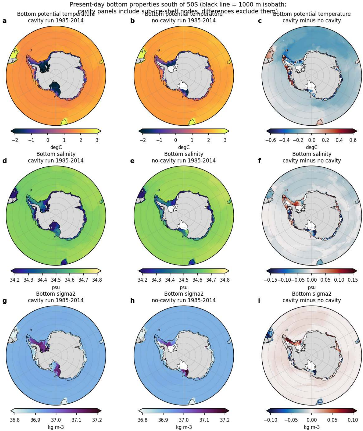
Figure 83: bottom_pd_maps (bottom). Present-day (1985-2014) bottom potential temperature (a-c), salinity (d-f) and sigma2 (g-i) south of 50S on a 0.25 degree grid. Left column cavity run including the sub-ice-shelf nodes, middle column no-cavity run, right column cavity minus no cavity on the common open-ocean grid. Black line is the 1000 m isobath. Units degC, psu, kg m -3 . The abyss is 1.7 to 2.0 degC and 36.9 kg m -3 in both runs, so there is no cold AABW layer. Cold (below -1.5 degC) and dense (above 37.0 kg m -3 ) bottom water exists only on the Weddell and Ross shelves and under the Filchner-Ronne and Ross ice shelves. The cavity run is 0.1 to 0.3 degC cooler over the whole deep Southern Ocean, and its western Weddell shelf is 0.05 to 0.1 psu saltier and 0.05 to 0.1 kg m -3 denser, whereas its Ross shelf is fresher and lighter by a similar amount.
