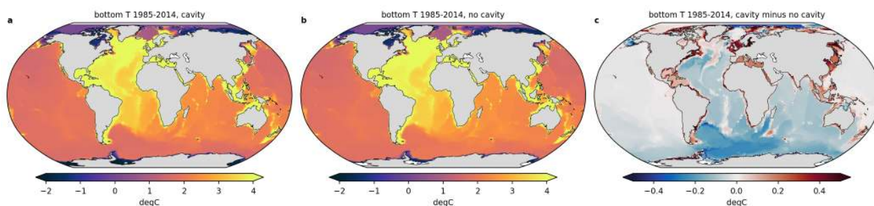
Figure 162: map_bottomT_pd (census). Present-day (1985-2014) bottom potential temperature for the cavity run (a), the no-cavity run (b) and the difference (c, regridded to 1 degree). The abyss is 1.5-2.5 degC almost everywhere south of 30S. The cavity run is 0.1-0.3 K colder in the deep Weddell and Ross Seas and along the Antarctic slope, and warmer only on parts of the shelf where the cavity mesh replaces open ocean by ice shelf.
