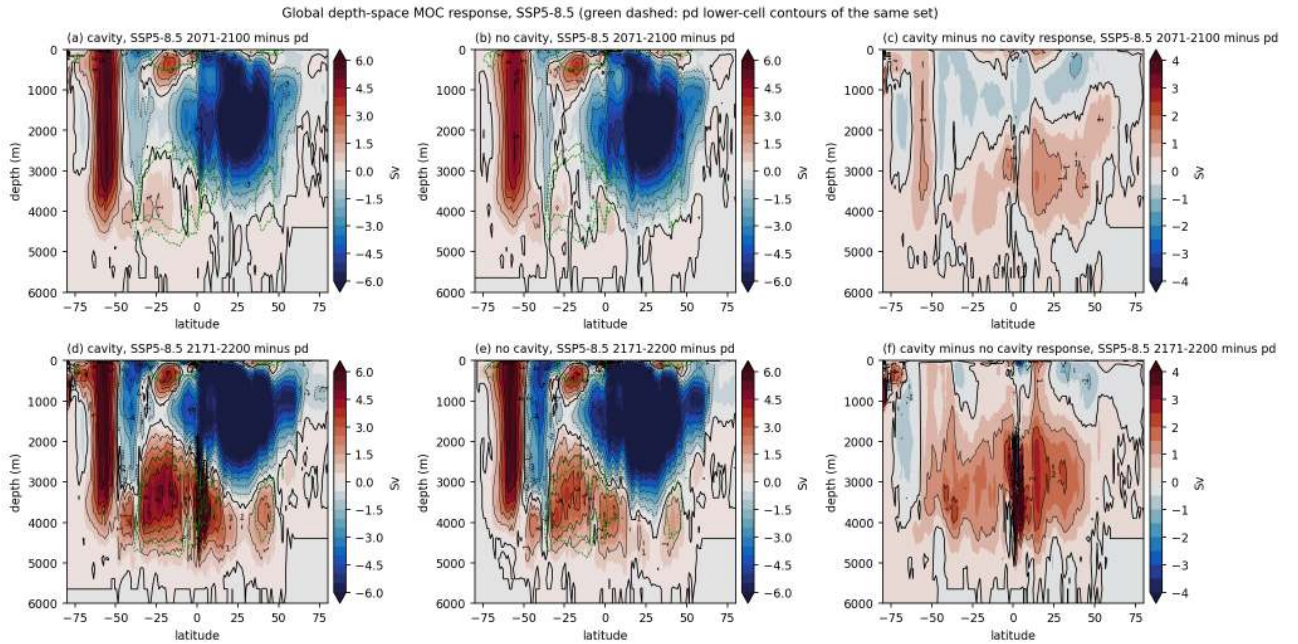
Figure 137: moc_z_response_ssp585 (moc). Change of the global depth-space streamfunction (Sv) under SSP5-8.5 for 2071-2100 minus pd (a-c) and 2171-2200 minus pd (d-f), cavity (a, d), no cavity (b, e) and cavity minus no cavity response (c, f). Green dashed lines show the -2 and -4 Sv pd contours of the lower cell of the same set. The NADW cell weakens by more than 6 Sv throughout the Atlantic depth range, the Deacon cell strengthens by 2-4 Sv in its core, and the abyssal cell weakens (positive anomaly) by 3-5 Sv between 40S and 10N below 2500 m by 2171-2200. The two sets respond alike. The cavity run loses 1-3 Sv more of the abyssal cell between 40S and 40N by 2171-2200 (panel f) because its pd cell was stronger, so both sets end at the same weak state.
