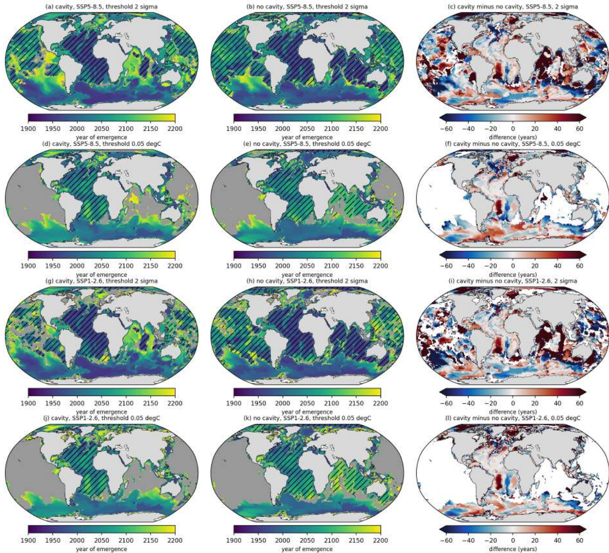
Figure 170: fig08_toe_btemp_maps (propagation). Time of emergence of the bottom temperature signal, defined as the first year from which the 11-yr running mean of the drift-corrected anomaly stays permanently beyond a threshold until 2195. Rows are SSP5-8.5 with a 2 sigma threshold (sigma = std of the detrended 1851-1950 annual values per node), SSP5-8.5 with an absolute threshold of 0.05 degC, and the same two for SSP1-2.6. Columns are cavity, no cavity and cavity minus no cavity (years). Grey means not emerged by 2195 and hatching marks emergence with a negative sign (cooling). Take-away. Abyssal interannual noise is tiny (median sigma 0.003 degC below 3000 m), so with the 2 sigma criterion 44 to 53 percent of the deep sea floor has emerged by 2014 and 92 to 97 percent by 2200. With the 0.05 degC criterion the Southern Ocean south of 45S emerges between 2005 and 2060, the Atlantic abyss (cooling) between 2020 and 2080, and the Pacific and Indian abyss north of 40S never emerge. The cavity and no-cavity emergence years differ by less than 20 years over most of the deep ocean.
