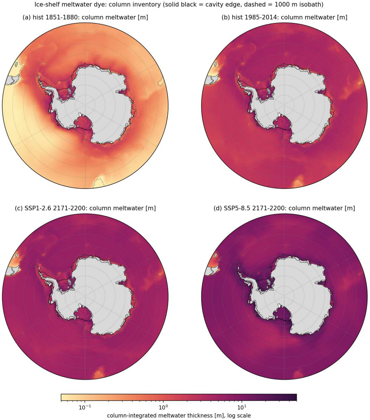
Figure 71: mw_fig06_column_maps (meltwater). Column-integrated meltwater thickness (metres of meltwater per square metre, log scale) south of 50S for hist 1851-1880, hist 1985-2014, SSP1-2.6 2171-2200 and SSP5-8.5 2171-2200. Black line is the cavity edge, dashed grey the 1000 m isobath. Cavity columns are included. Take-away. At present day the area-mean column holds 3.1 m on the open shelf, 3.3 m in the deep ocean south of 60S, 4.2 m under the ice shelves and 2.7 m in 60-50S, with maxima of 12 m in the Ross and Weddell coastal currents. In 2171-2200 under SSP5-8.5 the shelf holds 14.6 m (maxima 39 m) and the deep ocean south of 60S 7.4 m, against 3.9 and 5.2 m under SSP1-2.6.
