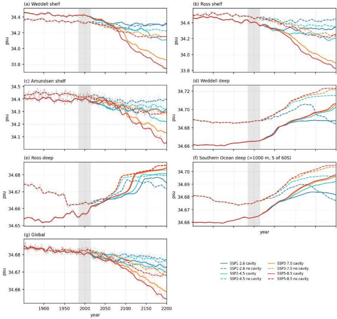
Figure 88: bottom_ts_S (bottom). Same as bottom_ts_T for bottom salinity (psu). Weddell and Ross shelf bottom salinities fall by 0.1 psu (SSP1-2.6) and 0.5 to 0.6 psu (SSP5-8.5) in the cavity run, while the deep basins become 0.02 to 0.04 psu saltier.
