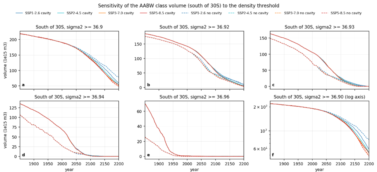
Figure 149: aabw_volume_threshold_sensitivity (census). As the previous figure for the volume south of 30S with thresholds 36.90, 36.92, 36.93, 36.94 and 36.96 (panel f repeats 36.90 on a log axis). The timing of the collapse moves with the threshold because the abyssal mode drifts to lower density at about 0.02 \text{ kg m}^{-3} per century and crosses each threshold in turn, but the statements above (scenario independence, earlier loss without cavities, larger dense volume with cavities) hold for all thresholds. Water above 36.96 disappears before 1950 in both sets.
