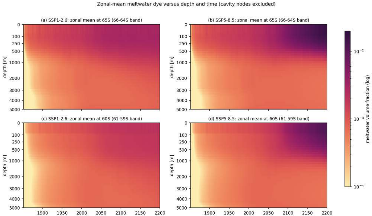
Figure 80: mw_fig15_hovmoeller_65S_60S (meltwater). Hovmoeller diagrams of the zonal-mean meltwater fraction versus depth and time in the 64-66S and 59-61S bands for SSP1-2.6 and SSP5-8.5 (cavity nodes excluded, log colour scale, square-root depth axis). Take-away. The abyss at 65S fills within 50 years after 1851 and reaches 0.69 permil below 3000 m at present day. Under SSP5-8.5 the surface at 65S rises from 1.9 to 15 permil by 2171-2200 while the concentration below 3000 m stays at 0.69 permil, and the 1000 m value rises only from 0.84 to 1.1 permil. The warm-scenario signal is confined to the upper 500 m.
