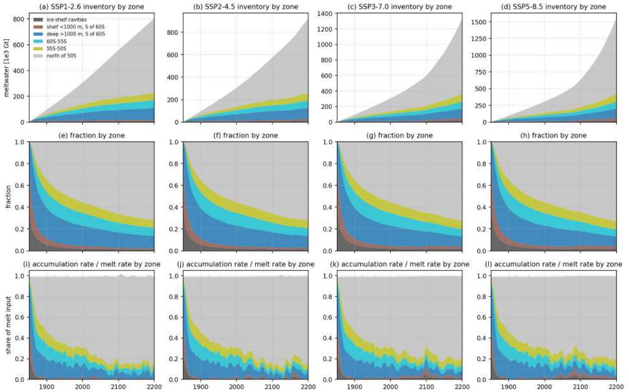
Figure 68: mw_fig03_zones (meltwater). Inventory by zone (ice-shelf cavities, open shelf shallower than 1000 m south of 60S, deep ocean south of 60S, 60-55S, 55-50S, north of 50S) as stacked inventories (a-d), fractions (e-h) and as the yearly accumulation rate of each zone divided by the melt rate, 11 yr smoothed (i-l). The last row shows where the meltwater released in a given year ends up on a net basis. Take-away. At present day the cavities hold 2.1 percent, the open shelf 2.3 percent, the deep Southern Ocean south of 60S 19 percent and the ocean north of 50S 55 percent of the inventory. Of the present-day melt input, 69 percent accumulates north of 50S, 17 percent in 60-50S, 12 percent in the deep ocean south of 60S and under 2 percent on the shelf and in the cavities. In 2171-2200 under SSP5-8.5 80 percent of the input accumulates north of 50S and only 5 percent in the deep ocean south of 60S.
