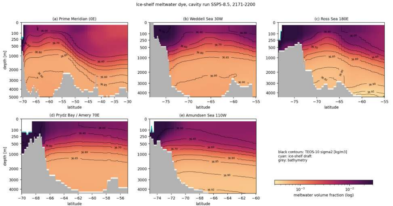
Figure 74: mw_fig09_sections_far585 (meltwater). As mw_fig08 for SSP5-8.5 2171-2200. Take-away. The slope maximum moves to the surface with 11 to 19 permil, the bottom of the slope keeps 0.6 to 0.85 permil (4.2 permil at 70E) and the sigma2 36.9 surface has retreated to below 2000 m. The five-fold larger melt input spreads as a surface plume and does not reach the slope bottom.
