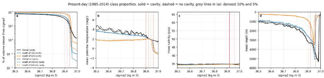
Figure 147: census_class_properties (census). Present-day class properties as a function of sigma2 for the global ocean (black), south of 30S (blue) and south of 60S (orange), cavity solid and no cavity dashed. (a) Percentage of the volume denser than a given sigma2 (log scale, grey lines at 10 and 5 percent). (b) Volume-weighted mean potential temperature, (c) salinity and (d) mean depth of each 0.005 class. The abyssal mode (36.90-36.96) has 1.8-2.0 degC and 34.67-34.69 psu at 3000-4500 m in both runs, i.e. the model AABW class is CDW-like. The cavity run has its densest classes 0.1-0.15 degC colder than the no-cavity run, which is why its mode is 0.01-0.02 kg m -3 denser.
