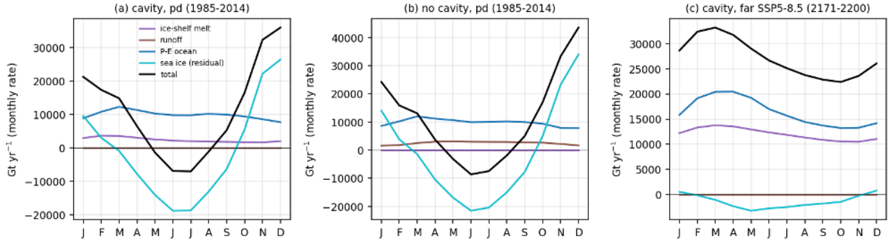
Figure 64: fw_budget_seasonal (melt). Seasonal cycle of the freshwater components south of 60S (monthly rates in Gt/yr) for (a) cavity pd, (b) no cavity pd and (c) cavity far SSP5-8.5. Ice-shelf melt has almost no seasonal cycle (2000 to 3500 Gt/yr). The Antarctic runoff in the no-cavity run peaks in winter (3000 Gt/yr in May to September, 1500 in January) following the accumulation season. Sea ice dominates the seasonal cycle (about -20000 Gt/yr freezing in June and July, +25000 to +35000 Gt/yr melt in November and December). In far SSP5-8.5 the sea-ice cycle nearly disappears and melt plus P-E supply 22000 to 33000 Gt/yr all year.
