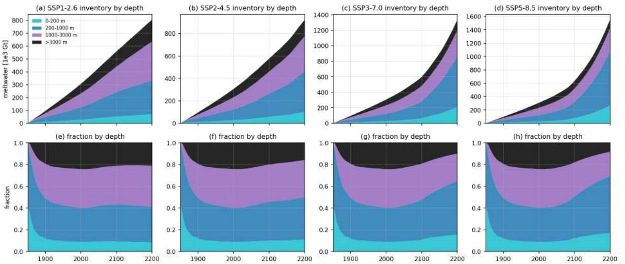
Figure 67: mw_fig02_layers (meltwater). Inventory by depth layer (0-200, 200-1000, 1000-3000, below 3000 m) for the four scenarios as stacked absolute inventories (a-d) and as fractions (e-h). Take-away. At present day 9, 31, 35 and 24 percent of all meltwater ever released sits in the four layers. Under SSP5-8.5 the upper ocean share grows to 17 plus 51 percent by 2171-2200 and the share below 3000 m shrinks to 9 percent, while SSP1-2.6 keeps 21 percent below 3000 m. New meltwater in the warm scenarios stays in the upper 1000 m.
