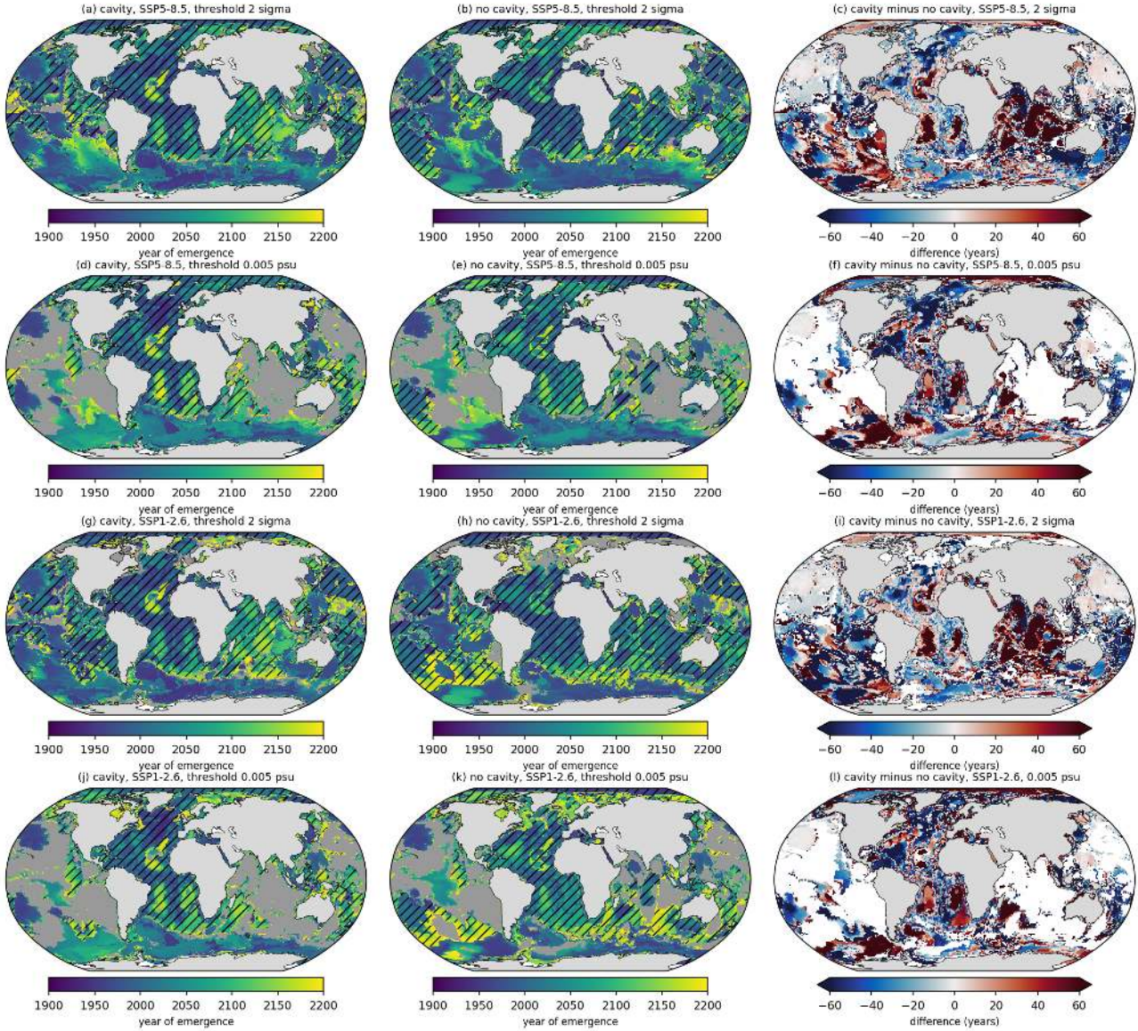
Figure 172: fig10_toe_bsalt_maps (propagation). As fig08 for bottom salinity, with 2 sigma and 0.005 psu thresholds. Take-away. Bottom salinity emerges with a positive sign (salinification) in the Southern Ocean and with a negative sign (freshening) in the Atlantic and Arctic abyss. With the 0.005 psu threshold the Southern Ocean south of 50S emerges between 2000 and 2060, the North Atlantic abyss between 2040 and 2120, and the abyssal Pacific does not emerge by 2195.
