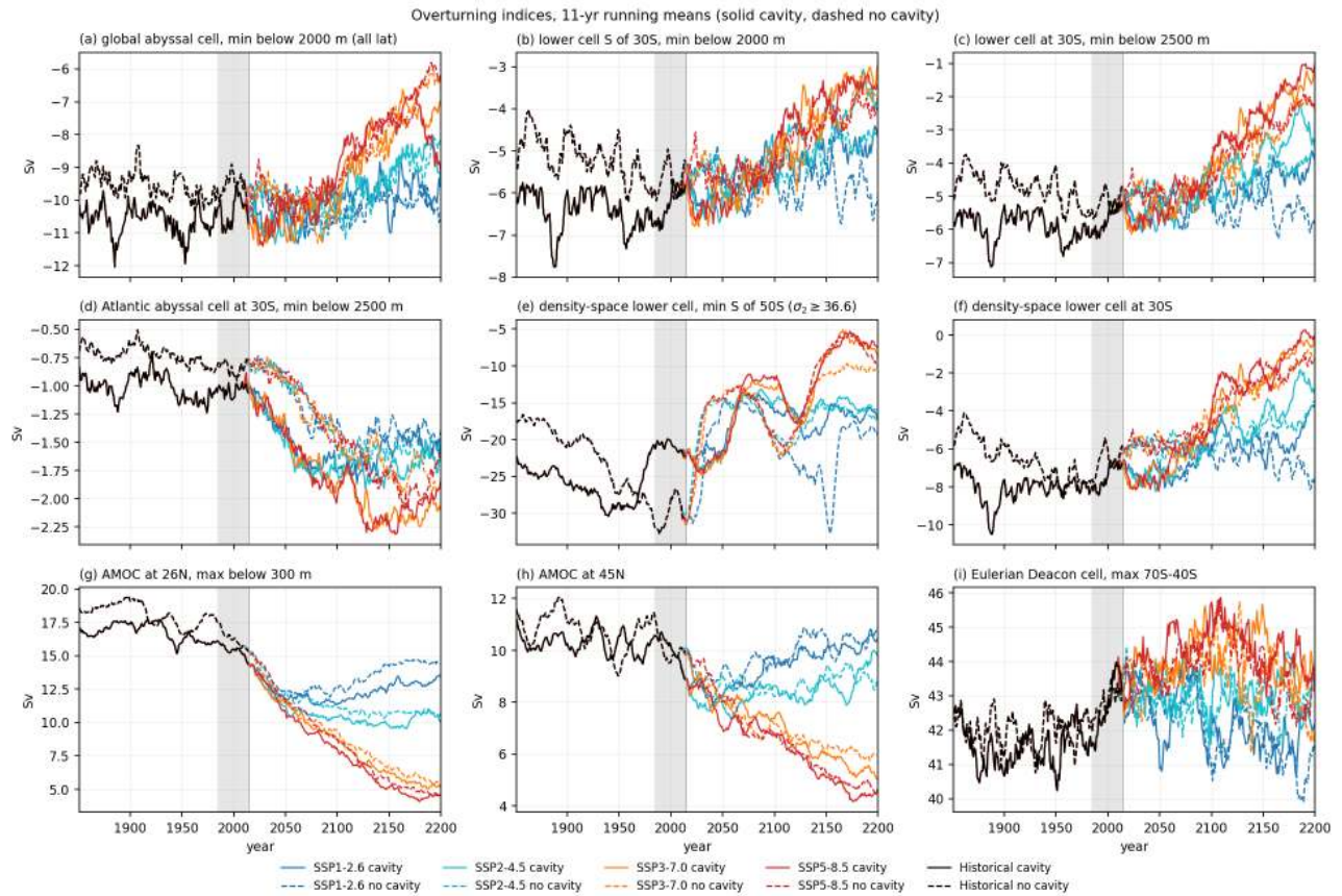
Figure 135: moc_indices_timeseries (moc). Eleven-year running means of overturning indices, 1851-2200, for all four SSP chains and both sets (solid cavity, dashed no cavity, black for the shared historical part, grey band pd). (a) global abyssal cell, minimum below 2000 m over all latitudes; (b) lower cell south of 30S, minimum below 2000 m; (c) lower cell at 30S, minimum below 2500 m; (d) Atlantic abyssal cell at 30S; (e) density-space lower cell, minimum south of 50S over sigma2 \geq 36.6 ; (f) density-space lower cell at 30S; (g) AMOC at 26N; (h) AMOC at 45N; (i) Eulerian Deacon cell maximum. The abyssal cell weakens only 25-32 percent by 2171-2200 under SSP5-8.5 and SSP3-7.0, whereas the lower cell at 30S loses 71-77 percent (cavity) and 57 percent (no cavity) and the density-space lower cell south of 50S loses 66-75 percent in both sets. The AMOC at 26N drops from 15.4 to 4.4 Sv (cavity) and from 16.2 to 4.8 Sv (no cavity) under SSP5-8.5 and to 13-14.5 Sv under SSP1-2.6. The Deacon cell changes by less than 5 percent.
