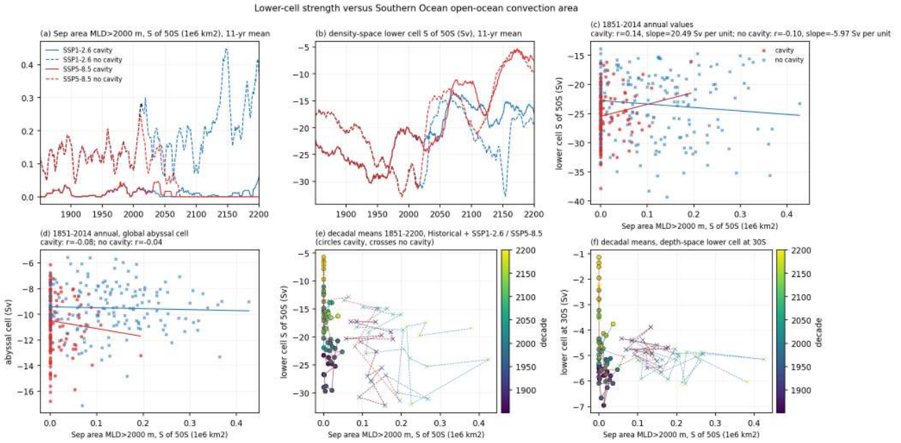
Figure 143: moc_vs_convection (moc). Relationship between lower-cell strength and Southern Ocean open-ocean convection. (a) September area with mixed layer deeper than 2000 m south of 50S (1e6 km²) and (b) the density-space lower cell south of 50S (Sv), 11-yr running means, historical plus SSP1-2.6 and SSP5-8.5 chains. (c) and (d) annual values 1851-2014, lower cell and global abyssal cell versus convection area, with linear fits and correlations for each set. (e) and (f) decadal means 1851-2200 (colour is the decade, circles cavity, crosses no cavity) for the density-space lower cell and the depth-space lower cell at 30S. The no-cavity run convects every winter near Maud Rise (0.10-0.16e6 km²) while the cavity run does so only in a few years, yet the interannual correlation between convection area and lower-cell strength is weak ( |r| < 0.15 for both sets). On centennial scales the no-cavity lower cell strengthens from -17 Sv (1851-1880) to -30 Sv (1985-2014) as its convection area grows from 0.10 to 0.16e6 km², whereas the cavity lower cell weakens from -27 Sv (1951-1980) to -21 Sv (pd) without convection.
