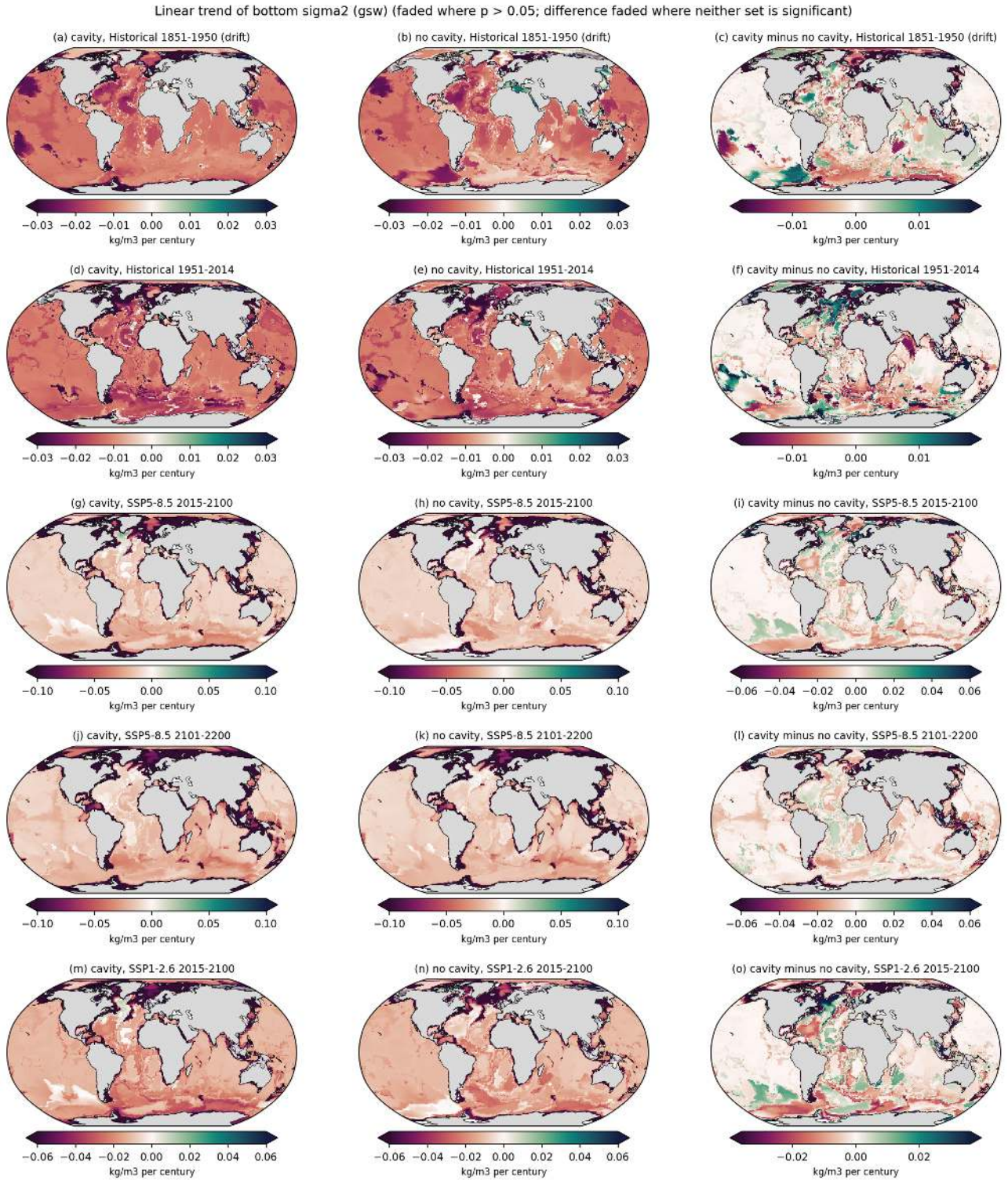
Figure 166: fig04_trend_bsig2_global (propagation). Same layout as fig01 for bottom sigma2 computed with gsw from bottom T and S (kg/m 3 per century). Take-away. Bottom density decreases everywhere except in parts of the North Atlantic; the Southern Ocean bottom lightens by 0.03 to 0.06 kg/m 3 per century in 2015-2100 under SSP5-8.5 because warming dominates over salinification. The abyssal Atlantic lightens despite cooling because freshening dominates.
