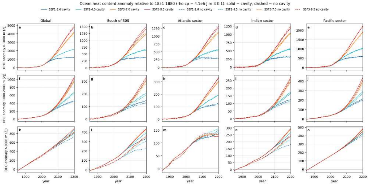
Figure 155: ohc_timeseries (census). Ocean heat content anomaly relative to 1851-1880 (ZJ, \rho_{cp} = 4.1 \times 10^6 J m -3 K -1 ) for 0-1000 m (top), 1000-2000 m (middle) and below 2000 m (bottom), for the global ocean, south of 30S and the Atlantic, Indian and Pacific sectors (full basins including their Southern Ocean part), all scenario chains and both sets. Cavity nodes are excluded from the layer means. Global 0-1000 m uptake by 2171-2200 is 1190-1200 ZJ (SSP1-2.6) and 4440 (cavity) to 4560 (no cavity) ZJ (SSP5-8.5). Below 2000 m the curves of all scenarios lie on top of each other until about 2100 (global 540 ZJ by end, 770-860 ZJ by far), which identifies a scenario-independent drift of 0.08 K per century. South of 30S below 2000 m the cavity run gains 30-70 ZJ more than the no-cavity run in all scenarios.
