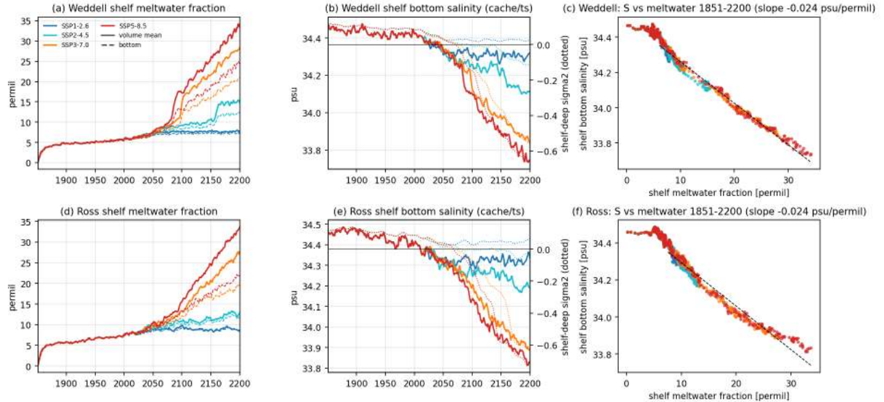
Figure 78: mw_fig13_shelf_relation (meltwater). Shelf meltwater and shelf water properties. (a, d) Volume-mean (solid) and bottom (dashed) meltwater fraction on the Weddell and Ross shelves (depth under 1000 m, cavity nodes excluded). (b, e) Shelf bottom salinity from cache/ts with the shelf minus deep bottom sigma2 contrast dotted (11 yr smoothed). (c, f) Bottom salinity versus shelf meltwater fraction for all years and scenarios with a linear fit over 2015-2200. Take-away. Present-day shelf meltwater is 5.8 permil (Weddell) and 7.5 permil (Ross), and 31 permil on both shelves in 2171-2200 under SSP5-8.5 (bottom 23 and 21 permil). Shelf bottom salinity falls by 0.0235 psu per permil of meltwater ( r = -0.99 on both shelves), 69 percent of the pure dilution slope of 0.034 psu per permil. The accumulated meltwater is more than enough to explain the whole projected shelf freshening. The shelf to deep density contrast crosses zero when the shelf meltwater fraction exceeds about 10 permil (Weddell 2072, Ross 2068 under SSP5-8.5).
