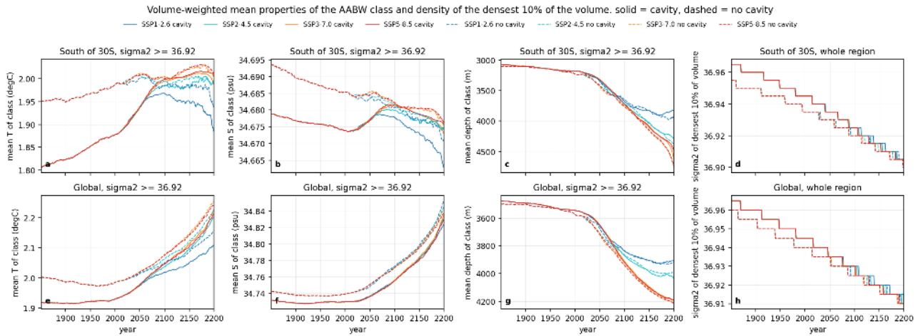
Figure 150: aabw_class_properties_timeseries (census). Volume-weighted mean potential temperature (a, e), salinity (b, f) and mean depth (c, g) of the AABW class ( \sigma_{\theta 2} \geq 36.92 ) south of 30S (top) and globally (bottom), and (d, h) the \sigma_{\theta 2} below which the densest 10 percent of the regional volume lies (0.005 resolution). The class south of 30S is 1.81 degC in 1851 and 1.88 degC at pd in the cavity run but 1.95-1.99 degC in the no-cavity run, it sinks from 3200 m to 3600 m (end) and 3900-4500 m (far) as the lighter upper part is lost. The densest 10 percent of the Southern Ocean volume lightens from 36.965 (cavity) and 36.955 (no cavity) in 1851 to 36.905 in 2200, by 0.06 kg m -3 in 350 years, at almost the same rate in all scenarios, and the 0.01 kg m -3 offset between the sets closes after about 2100.
