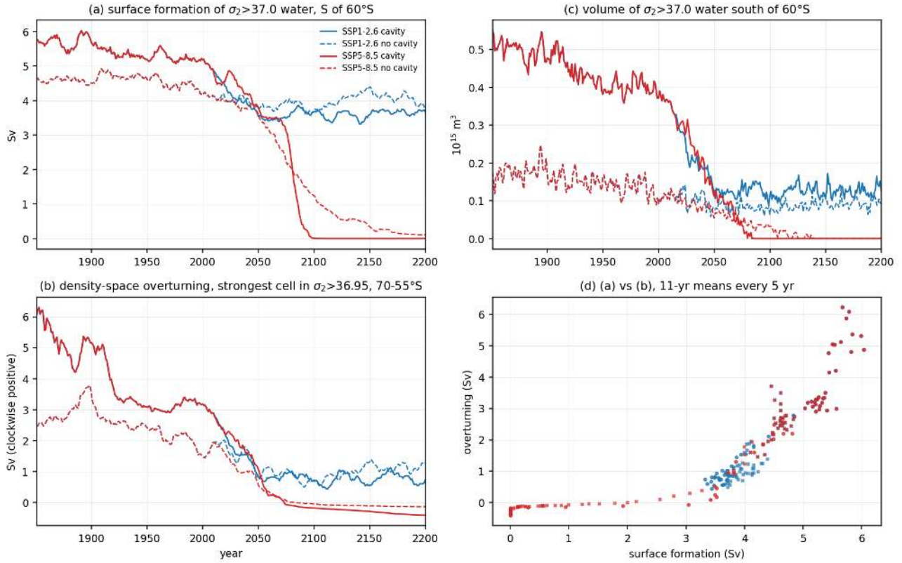
Figure 107: wmt_fig08_consistency_moc_census (wmt). Consistency of the surface formation with the interior. (a) surface formation of \sigma_2 above 37.0 water south of 60S, (b) strength of the densest overturning cell in density space (minimum of the global density-space stream function for \sigma_2 above 36.95 between 70S and 55S, sign reversed so that the clockwise AABW-type cell is positive), (c) volume of \sigma_2 above 37.0 water south of 60S from the census, (d) scatter of (a) against (b). SSP1-2.6 and SSP5-8.5 shown for both sets. The present-day dense cell is 3.1 Sv (cavity) and 1.8 Sv (no cavity), far smaller than the 5.1 and 4.3 Sv surface formation, and the dense volume is only 0.38 and 0.12 times 10^{15} \text{ m}^3 (0.5 and 0.2 percent of the volume south of 60S), so the residence time of surface-formed dense water is 1 to 2 years. Most of the surface densification is eroded by mixing before it reaches the deep ocean. The 11-yr smoothed surface formation and dense cell are correlated at 0.86 to 0.96 along the scenario chains. Under SSP5-8.5 the dense cell and the dense volume vanish in 2071-2100 in both sets.
