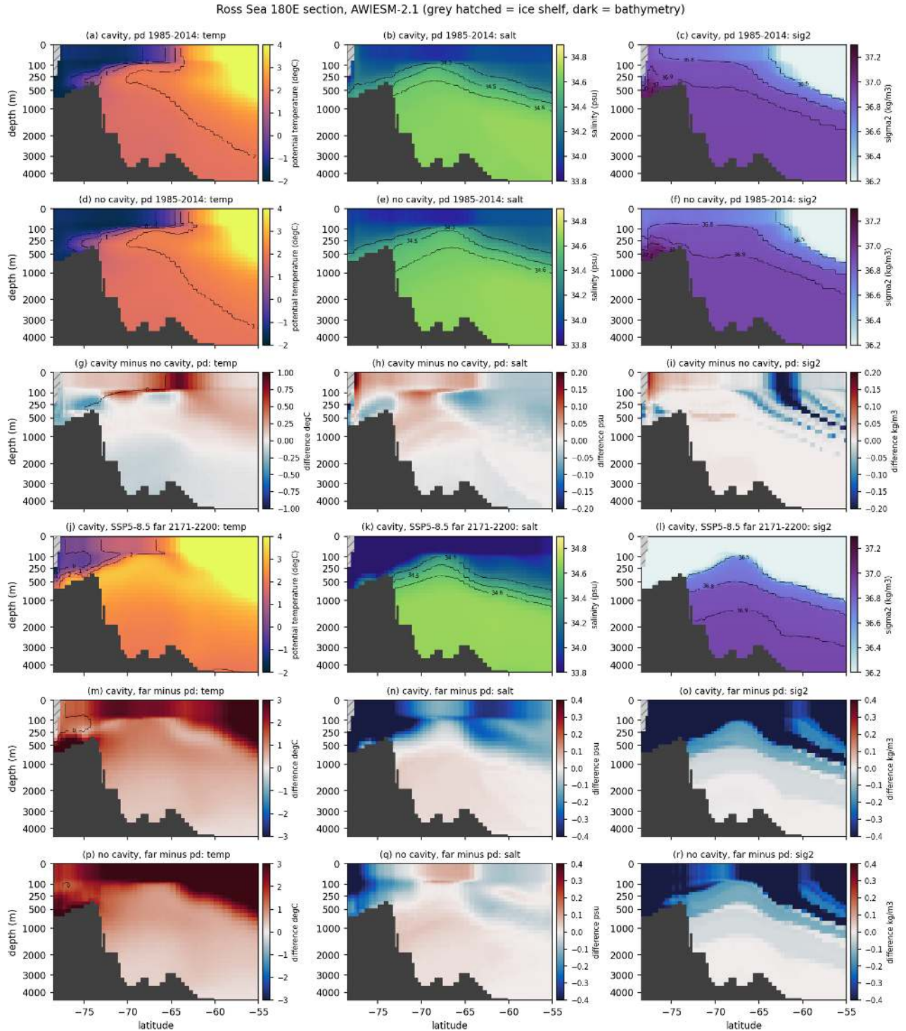
Figure 121: circ_sec_ross180 (circ). As above for 180E, 78.5S-55S across the Ross Sea shelf, slope and gyre. Take-away: the Ross shelf holds the densest model shelf water (bottom sigma2 37.03, S 34.41-34.44, T -0.8 to -0.6 degC) but it remains confined to the shelf. Under SSP5-8.5 the Ross shelf bottom warms to 2.5 (cavity) and 2.2 degC (no cavity) and freshens by 0.3 and 0.14 psu, the largest shelf change of all sections, and the shelf bottom density drops to 36.2 (cavity) and 36.7 (no cavity).
