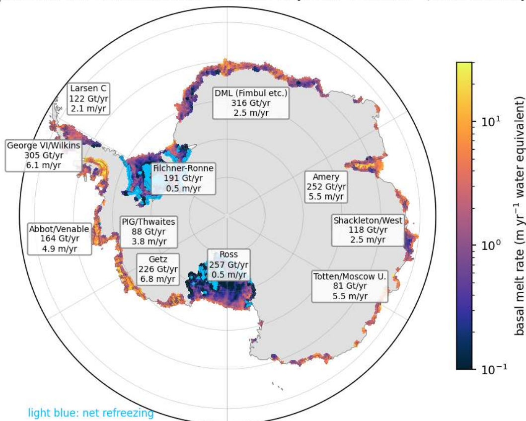
(a) PI_ICEv2_hist 1985-2014 basal melt rate; total 2364 Gt/yr over 1.42e6 km 2 (mean 1.66 m/yr)
