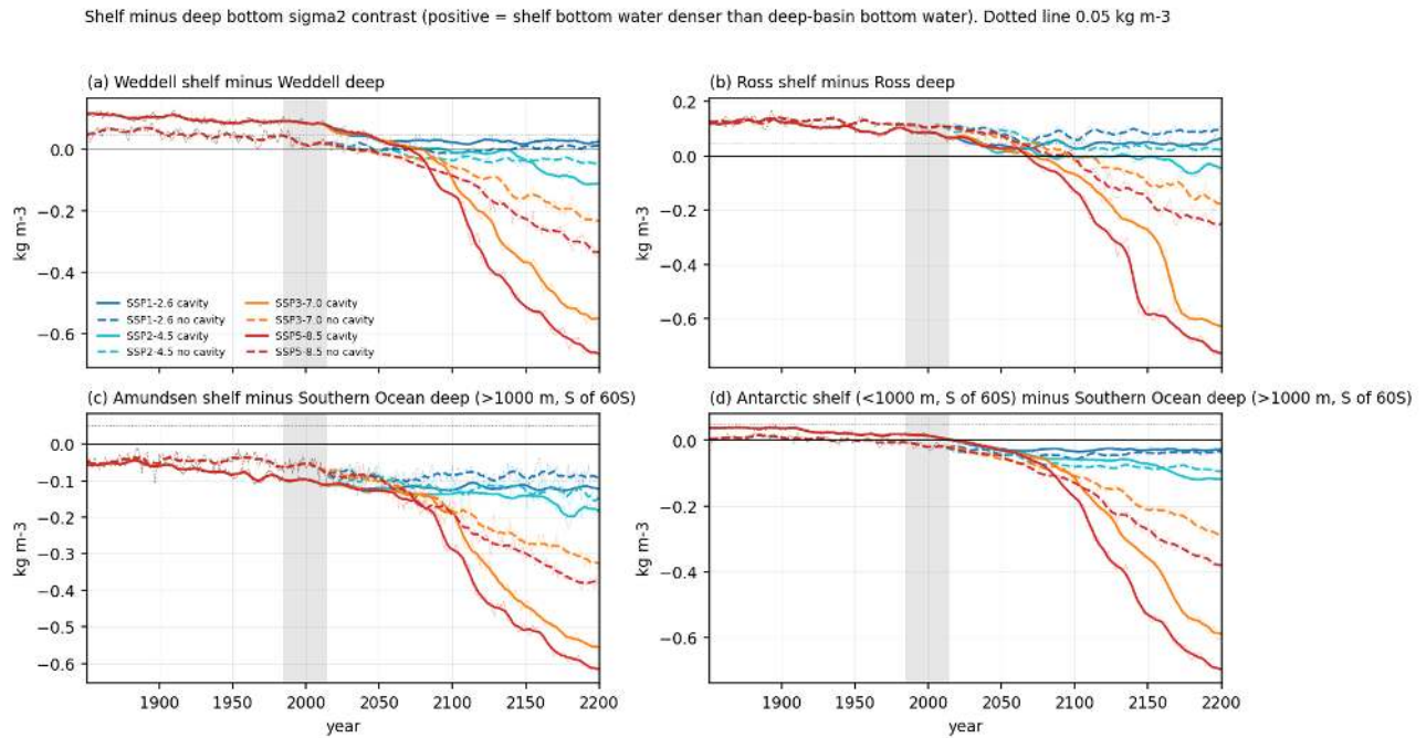
Figure 90: bottom_ts_contrast (bottom). Shelf minus deep bottom sigma2 contrast (kg m -3 ): Weddell shelf minus deep Weddell (a), Ross shelf minus deep Ross (b), Amundsen shelf minus deep Southern Ocean (c) and all Antarctic shelf minus deep Southern Ocean (d), 1851-2200, 11-yr running means over annual values. Positive values mean the shelf bottom water is on average denser than the deep bottom water and can in principle sink. Dotted line 0.05 kg m -3 . The Weddell and Ross contrasts are 0.08 to 0.12 kg m -3 in 1851-1880, have already halved by 2014 in the no-cavity Weddell, and reach zero around 2070 (Weddell cavity run SSP5-8.5 in 2072, Ross in 2068). Under SSP1-2.6 they level off at 0.02 to 0.05 kg m -3 and never vanish. The Amundsen shelf is always lighter than the deep ocean.
