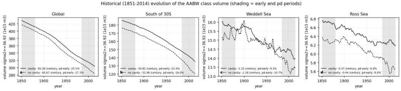
Figure 154: hist_drift_aabw_volume (census). Historical (1851-2014) evolution of the AABW class volume ( \sigma_2 \geq 36.92 ) for the global ocean, south of 30S, the Weddell Sea and the Ross Sea, cavity solid and no cavity dashed, with linear trends and the pd minus early change. The class loses 81 (cavity) and 86 (no cavity) \times 10^{15} m 3 per century globally and 31 and 33 \times 10^{15} m 3 per century south of 30S, i.e. 22-27 percent between early and pd. The Weddell and Ross Sea volumes fall by 9-11 and 7-9 percent. This is a spin-up drift of the abyss common to both sets.
