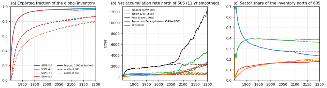
Figure 75: mw_fig10_export (meltwater). Export. (a) Fraction of the global inventory beyond the 1000 m isobath (solid), north of 60S (dashed) and north of 55S (dotted) for all scenarios. (b) Net accumulation rate of the inventory north of 60S per sector and in total, 11 yr smoothed, SSP5-8.5 solid and SSP1-2.6 dashed. (c) Sector share of the inventory north of 60S. Take-away. At present day 96 percent of all meltwater released since 1851 is beyond the 1000 m isobath, 77 percent is north of 60S and 65 percent north of 55S. The accumulation rate north of 60S is 2010 Gt/yr at present day (85 percent of the melt rate) and 11100 Gt/yr in 2171-2200 under SSP5-8.5. The Indian sector carries 39 percent of the northward export, the Weddell sector 29 percent, Ross and Amundsen 16 percent each.
