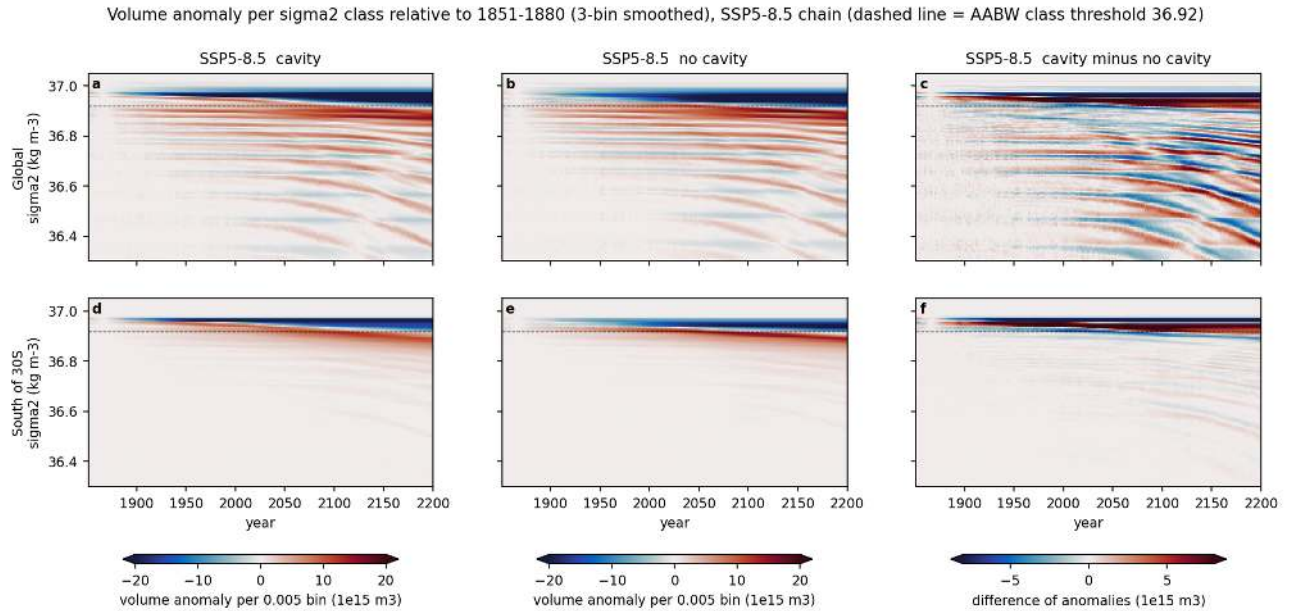
Figure 151: hov_density_ssp585 (census). Hovmoeller diagram of the volume anomaly per 0.005 \sigma_{\theta 2} class relative to 1851-1880 (3-bin running mean in density) for the SSP5-8.5 chain, global (top) and south of 30S (bottom), cavity (left), no cavity (middle) and the difference of the anomalies (right). The dashed line is the 36.92 threshold. The abyssal mode loses volume above 36.93 and gains below it from 1851 on, the band of gain migrates steadily to lower density (36.90-36.92 by 2100, 36.85-36.90 by 2200), and after 2050 volume is lost across the whole column above 36.7 as the upper ocean warms. The difference panel shows the cavity run keeping more volume in the 36.93-36.96 classes until about 2100.
