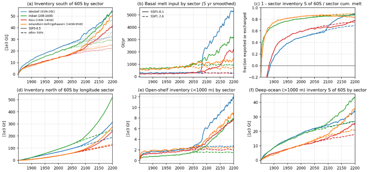
Figure 69: mw_fig04_sectors (meltwater). Sector view. Sectors are Weddell (65W-20E), Indian (20E-160E), Ross (160E-140W) and Amundsen-Bellingshausen (140W-65W). (a) Inventory south of 60S per sector for all scenarios (SSP5-8.5 solid, others dashed). (b) Basal melt per sector from the named ice shelves in cache/ts, SSP5-8.5 solid and SSP1-2.6 dashed. (c) One minus the sector inventory south of 60S divided by the sector cumulative melt, a measure of how much of a sector's own meltwater has left its southern domain (negative values mean net import from other sectors). (d) Inventory north of 60S by longitude sector. (e) Open-shelf inventory per sector. (f) Deep-ocean inventory south of 60S per sector. Take-away. The Weddell sector holds the largest inventory south of 60S at present day although its melt input (about 300 Gt/yr) is the smallest. It retains 51 percent of its own cumulative input while the Indian and Amundsen sectors retain 19 and 15 percent. The Weddell sector imports meltwater from upstream along the coastal current and keeps it in the gyre. The Indian sector exports most (39 percent of the inventory north of 60S). After the FRIS melt jump in 2078 (SSP5-8.5) the Weddell open-shelf inventory doubles within 15 years.
