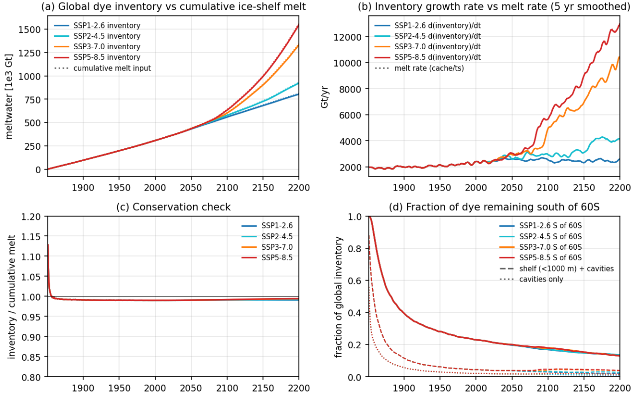
Figure 66: mw_fig01_budget (meltwater). Tracer history and budget. (a) Global dye inventory (sum of concentration times cell volume, in 1e3 Gt) for the four scenario chains, with the cumulative basal melt from cache/ts melt_shelf dotted. (b) Yearly growth rate of the inventory versus the melt rate, 5 yr smoothed. (c) Ratio of inventory to cumulative melt (the annual-mean dye lags the input by half a year, which is corrected). (d) Fraction of the global inventory that resides south of 60S, on the shelf plus cavities, and in the cavities only. Take-away. The dye starts from zero in 1851 (the 1851 annual mean holds 1078 Gt, half of one year of melt). It is conserved to 1 percent over 350 years (ratio 0.990 in 2014 and 0.991 to 0.994 in 2200). The inventory is 340e3 Gt in 2014 and 805e3 (SSP1-2.6) to 1552e3 Gt (SSP5-8.5) in 2200. The fraction south of 60S falls from 73 percent in 1851-1880 to 23 percent in 1985-2014 and 14 percent in 2171-2200 in all scenarios, and the shelf plus cavity share is only 4.4 percent at present day.
