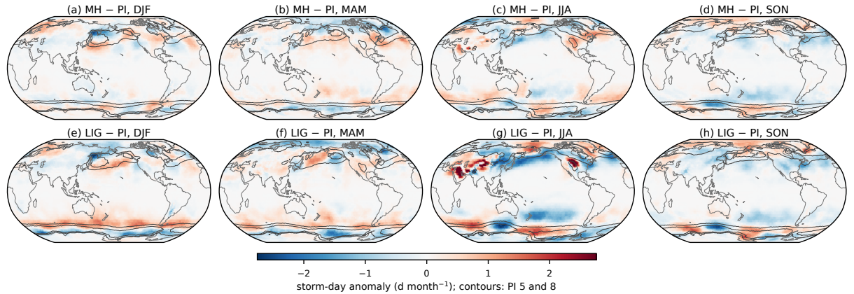
FIG. A4. Storm-day anomalies of the real-orbit experiments relative to piControl, from the same storm-day product as the main ensemble. (a)–(d) midHolocene minus piControl for DJF, MAM, JJA, and SON. (e)–(h) lig127k minus piControl. Contours outline the piControl climatology at 5 and 8 d month -1 . The isolated warm-season maxima over subtropical continental interiors reflect stationary surface heat lows rather than traveling cyclones.
