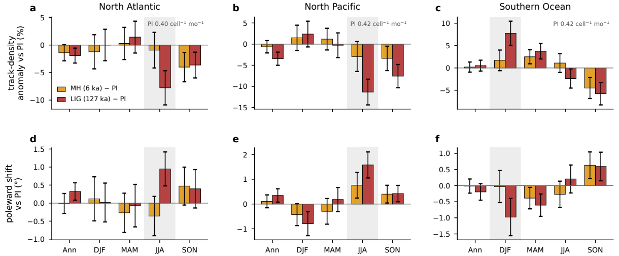
FIG. A3. Seasonal storm response of AWI-ESM-1-1-LR to real orbital states, tracked with the same pipeline as the main ensemble and referenced to piControl. (a)–(c) Anomalies of basin-mean track density for midHolocene (gold) and lig127k (red), as percentages of the piControl mean, for the annual mean and the four seasons, with error bars giving twice the standard error of the 30-year difference and the local summer shaded. Track density is normalized per T63 grid cell, and the annotated piControl values give the absolute scale in the units of Fig. 4. (d)–(f) The corresponding change in the track-point mean latitude, positive poleward.
