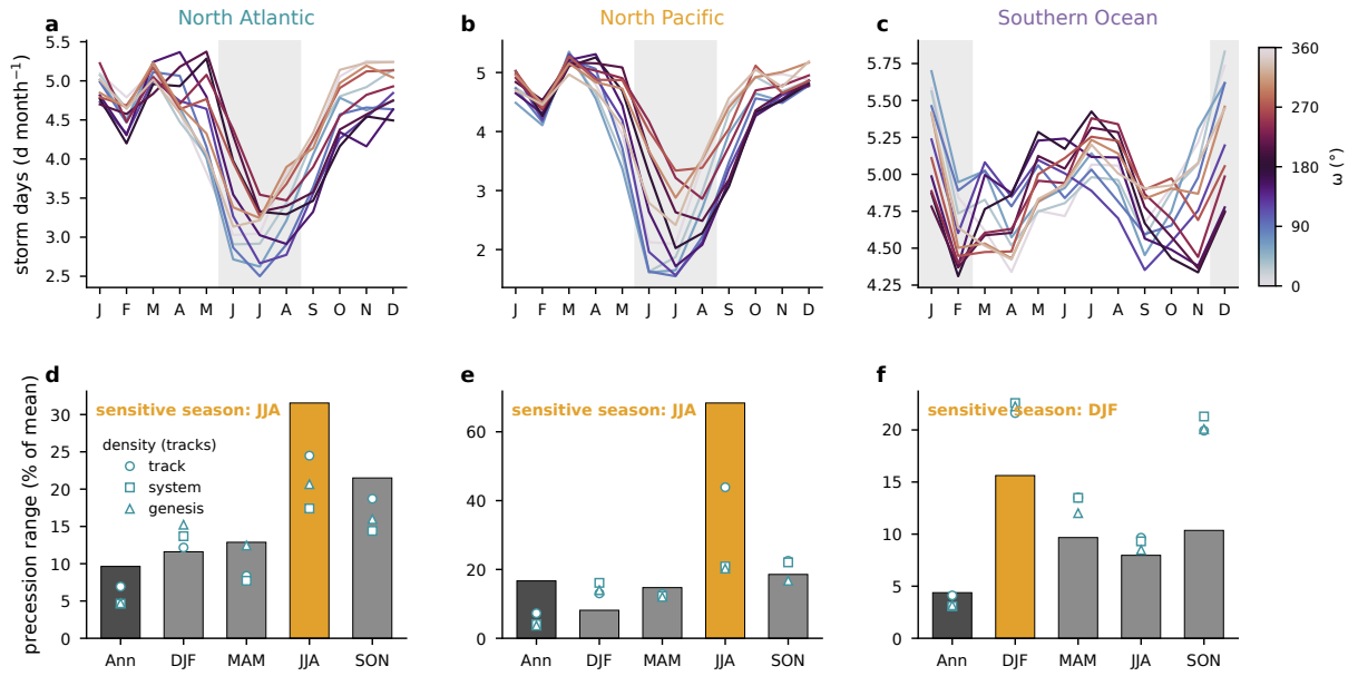
FIG. 4. Seasonal concentration of the precessional storm response. (a)–(c) Basin-mean storm days (d month -1 ) by calendar month for the North Atlantic, the North Pacific, and the Southern Ocean, one line per phase colored by \omega , with local summer shaded. (d)–(f) Across-phase range of storm days (maximum minus minimum, percent of the phase mean) for the annual mean and the four seasons, with the local-summer bar highlighted; open symbols give the corresponding ranges of track, system, and genesis densities from the Lagrangian tracks.
